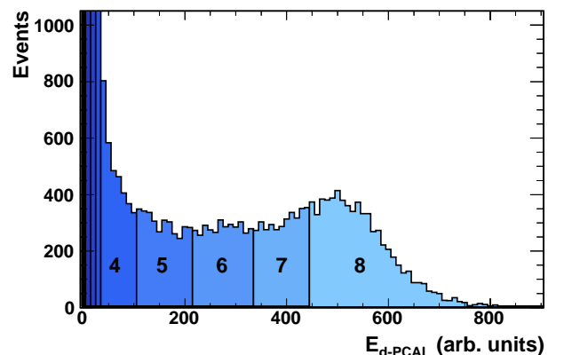
Figure 8. (Color online) Regions used to study the characteristics of events with different total charge deposited in the d-PCAL. Region 0 is the black colored bin located at the lowest detected E_{\text{d-PCAL}} signal.
