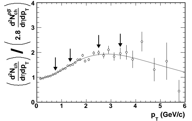
Figure 15. The ratio of d^2N_{ch}/dp_T d\eta of d+Au in the 40-70% E_{Ring} centrality bin to that in p+\bar{p} , scaled by 2.8 so that the ratio is unity at p_T = 0.35 GeV/c. The line is the ratio of fits to the two spectra using Eq. 1. The arrows mark the p_T values at which the centrality dependence of the relative yield is studied (see Fig. 16).
