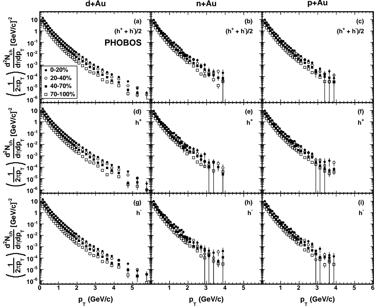
Figure 11. The invariant yield of (h^+ + h^-)/2 , h^+ , and h^- in four centrality bins determined for d+Au using the E_{\text{Ring}} centrality variable. The spectra for d+Au , n+Au , and p+Au are shown in separate columns. Due to the use of identical E_{\text{Ring}} cuts in all cases, the different data sets do not correspond to the listed fraction of the total inelastic cross section for nucleon-gold interactions. See text for details. Only statistical errors are shown. The spectra are obtained using particles that have a pseudorapidity 0.2 < \eta < 1.4 .
