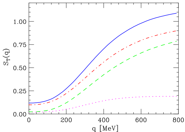
FIG. 2. (color online) Sum rule of the electromagnetic response of carbon in the transverse channel. The dashed line shows the results obtained including the one-nucleon current only, while the solid line corresponds to the full calculation. The dot-dash line represents the sum rule computed neglecting the interference term, the contribution of which is displayed by the dotted line. The results are normalised so that the dashed line approaches unity as |\mathbf{q}| \rightarrow \infty . Monte Carlo errors bars are not visible on the scale of the figure.
