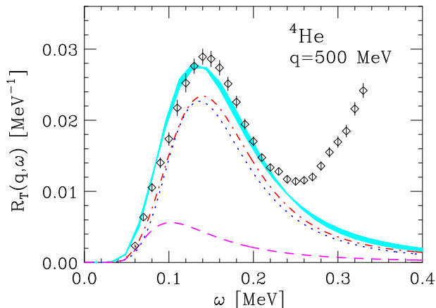
FIG. 1. (color online) Transverse response function of {}^4\text{He} , obtained within the approach of Ref. [18]. The shaded area shows the results of the full calculation, with the associated uncertainty arising from the inversion of the Euclidean response, while the dotted line has been obtained including the one-nucleon current only. The dot-dash line represents the response computed neglecting the interference term, the contribution of which is displayed by the dashes. The data are taken from Ref. [13].
