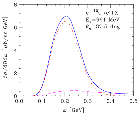
FIG. 3. (color online) Cross section of the process e + {}^{12}\text{C} \rightarrow e' + X at beam energy E_e = 961 MeV and electron scattering angle \theta_e = 37.5 deg, computed using Eq. (18) with the spectral function of Ref. [20]. The solid line shows the results of the full calculation, while the dot-dash and dashed lines, respectively.
