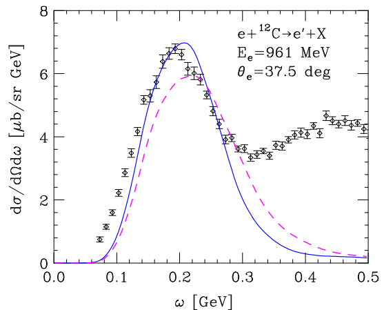
FIG. 4. (color online) Electron-carbon cross section obtained from Eq. (18) using relativistic (solid line) and non relativistic (dashed line) kinematics. The experimental data are from Ref. [23].
