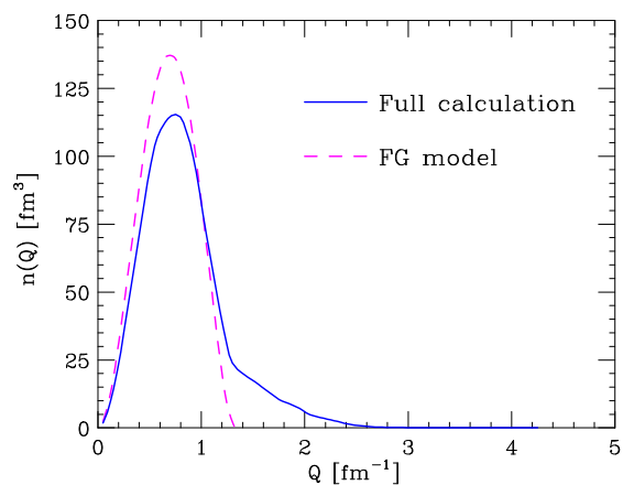
FIG. 5. (color online) Relative momentum distribution of a nucleon pair in isospin symmetric nuclear matter at equilibrium density.
