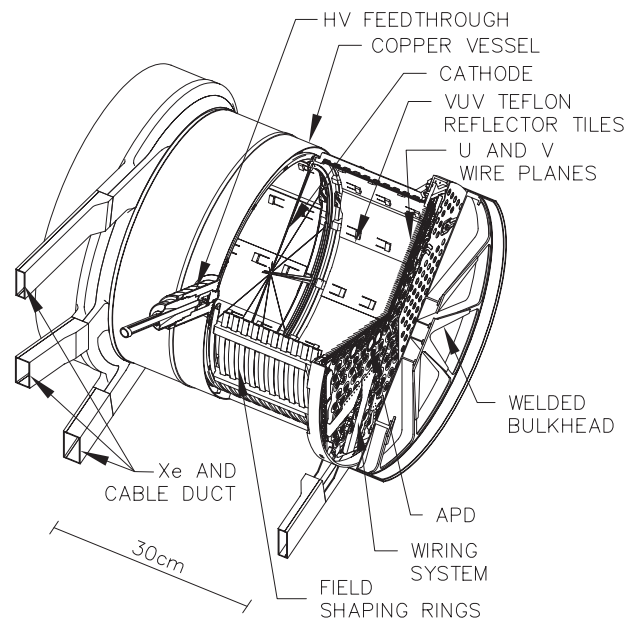
FIG. 2. Cutaway view of the EXO-200 Cu TPC. 'Wiring system' refers to the flat polyimide cables behind the APD platter. Additional flat polyimide cables are within the Cu TPC legs ('Cable duct' in figure). Acrylic spacers, insulators and field cage resistors are components of the as shown 'Field shaping rings' system, and are all external to the Teflon ® reflectors ('VUV (Vacuum Ultraviolet) Teflon Reflector Tiles'). A Cu tube and support system used for deployment of calibration sources outside the Cu vessel is not shown.
