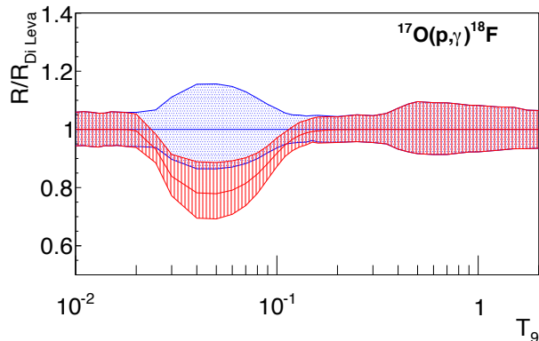
FIG. 14. (Color online) Comparison of the THM reaction rate of the ^{17}\text{O}(p,\gamma)^{18}\text{F} reaction with the direct one [28]. The blue area is used to display the range on uncertainty characterizing direct data [28]. The red area, instead, marks the reaction-rate interval allowed by the experimental uncertainties on the 65 keV resonance strength only, as listed in Tab. III.
