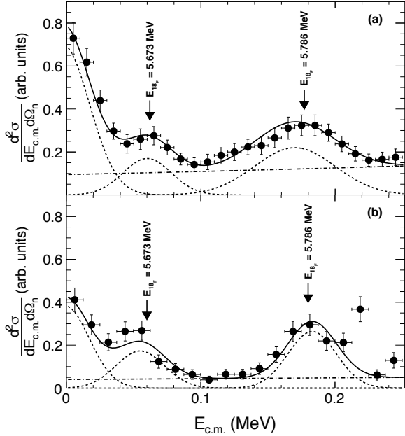
FIG. 12. Cross section of the TH reaction (full circles) for the LNS (a) and NSL (b) experiments. The full line represents the result of a fit including three Gaussian curves and a first-order polynomial to take into account the combinatorial background contribution to the cross section.
