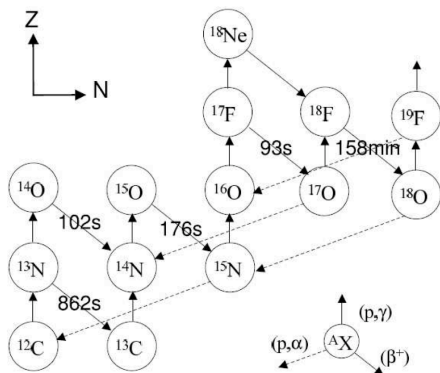
FIG. 1. Scheme of the carbon-nitrogen-oxygen (hot CNO) cycle of hydrogen burning which operates in nova explosions. The lifetime of the unstable nuclei are displayed.
