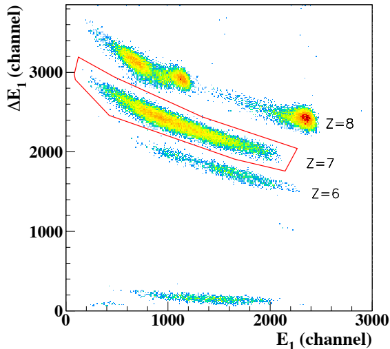
FIG. 5. (Color online) \Delta E - E matrix for the gas detector used as a first stadium of the telescopes formed with the PSD 1 . The telescopes were devoted to the identification of Z=7 particles, which are selected with a graphical cut (red lines).
