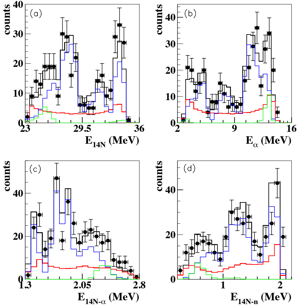
FIG. 9. (Color online) {}^2\text{H}({}^{17}\text{O}, \alpha {}^{14}\text{N})n yield as a function of E_{14\text{N}} , E_\alpha , E_{14\text{N}-\alpha} and E_{14\text{N}-n} for \theta_{14\text{N}}=6.0^\circ \pm 0.5^\circ and \theta_\alpha=21.0^\circ \pm 0.5^\circ . In panel (a), the black line is a fit of the coincidence yield obtained by taking into account SD (green line), QF (blue line) as well as combinatorial background (red line) contributions summed incoherently (see text for more details). In panels (b)-(d), the data are represented as a function of other variables. A remarkable agreement between the data and the incoherent sum (black lines) obtained using the same parameters for the SD (green line), QF (blue line) and combinatorial background contributions (red line) is clearly shown for all of the variables.
