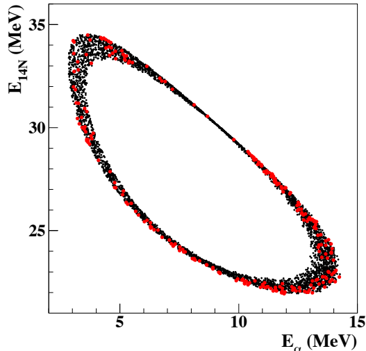
FIG. 7. (Color online) Experimental kinematic locus (red circles) for the 3-body {}^2\text{H}({}^{17}\text{O}, \alpha {}^{14}\text{N})\text{n} reaction induced at E_{beam}=41 MeV and for \theta_{14\text{N}} = 6.0^\circ \pm 0.5^\circ and \theta_\alpha = 21.0^\circ \pm 0.5^\circ (LNS experiment), superimposed onto the simulated kinematical locus (black circles) as discussed in the text. The spectra is relative to the events measured in coincidence among PSD 1 -PSD 5 detectors.
