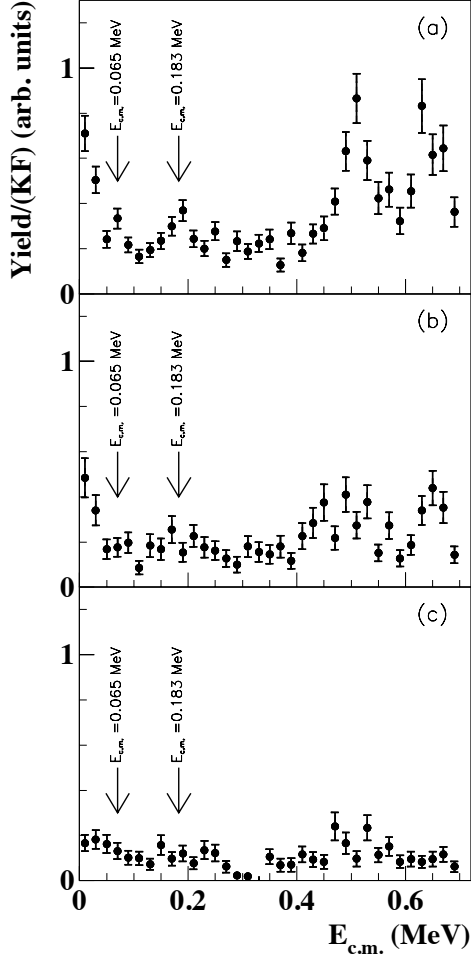
FIG. 10. PSD 1 -PSD 5 coincidence yield (LNS experiment), extracted for different neutron momentum p_n ranges: |\vec{p}_n| \leq 30 MeV/c (a), 30 \text{ MeV/c} \leq |\vec{p}_n| \leq 60 MeV/c (b) and finally 60 \text{ MeV/c} \leq |\vec{p}_n| \leq 90 MeV/c (c). In each case, the coincidence yield is divided by the kinematical factor to remove phase-space effects, thus the trend of the cross section as a function of E_{c.m.} and of p_n only is left out.
