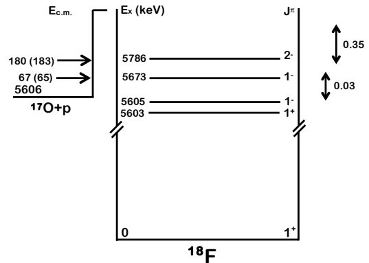
FIG. 2. Diagram of the ^{18}\text{F} levels intervening in the ^{17}\text{O}(p,\alpha)^{14}\text{N} up to energies of about 200 keV. The excitation energies and the J^\pi assignments are from [11]. The energy of the ^{17}\text{O} -p system in the center of mass reference system, E_{c.m.} , of the observed resonances are indicated, as reported in [11]. The values in the bracket are those measured in the recent works of [12, 13]. The vertical arrows fix the Gamow windows for nova explosion ( T_9 = 0.35 ) and AGB stars ( T_9 = 0.03 ).
