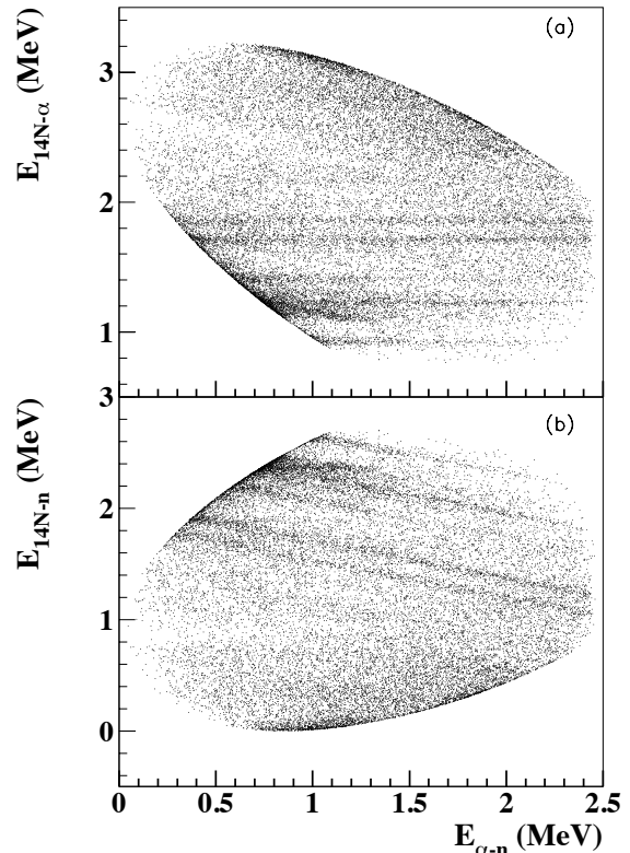
FIG. 8. (a) E_{14\text{N}-\alpha} vs. E_{\alpha-n} 2D plot. The presence of horizontal loci at E_{14\text{N}-\alpha}=1.26 MeV, 1.37 MeV, 1.67 MeV and 1.82 MeV demonstrates the feeding of the {}^{14}\text{N}+\alpha+n channel through the population of the {}^{18}\text{F} excited states at E_X=5.672 MeV ( J^\pi=1^- ), E_X=5.786 MeV ( J^\pi=2^- ), E_X=6.094 MeV ( J^\pi=4^- ) and E_X=6.108 MeV ( J^\pi=1^+ ) (unresolved), E_X=6.240 MeV ( J^\pi=3^- ) and E_X=6.242 MeV ( J^\pi=3^- ) (unresolved), respectively. Moreover, the horizontal loci at E_{14\text{N}-\alpha}=1.09 and 1.19 MeV corresponded to three sub-threshold levels (two of them are unresolved) at E_X=5.502 ( J^\pi=3^- ), E_X=5.603 ( J^\pi=1^+ ), E_X=5.605 ( J^\pi=1^- ) MeV. (b) Similarly, the E_{14\text{N}-n} vs. E_{\alpha-n} 2D plot shows the occurrence of a SD process taking place by populating {}^{15}\text{N} excited states at E_X from 13 and 13.35 MeV determining the appearance of horizontal loci at \sim 2.0 and \sim 2.5 MeV.
