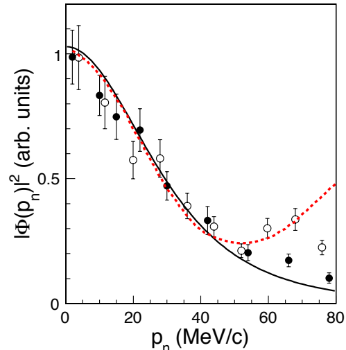
FIG. 11. (Color online) Experimental momentum distributions (full dots for LNS experiment and empty dots for NSL experiments) compared with the theoretical ones, given by the square of the Huthén function (black line) in the PWIA and by the DWBA momentum distribution evaluated by means of FRESKO code (red dotted line).
