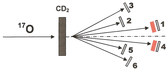
FIG. 4. (Color online) Experimental set-up adopted for the study of the ^2\text{H}(^{17}\text{O},\alpha\ ^{14}\text{N})\text{n} reaction. The displacement of the detectors assures the covering of the QF angular region.
