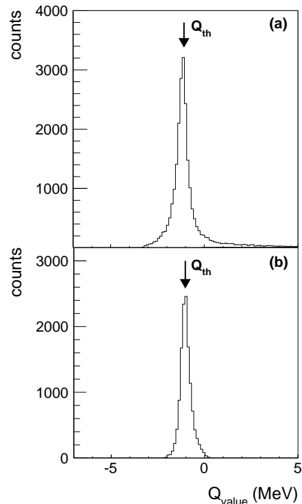
FIG. 6. Experimental Q -value spectra for LNS (a) and NSL (b) experiments. A single peak shows up in both spectra, centered at about -1.0 MeV, corresponding to the {}^2\text{H}({}^{17}\text{O},\alpha){}^{14}\text{N} channel. The black arrows correspond to the theoretical Q -value, Q_{th}=-1.033 MeV.
