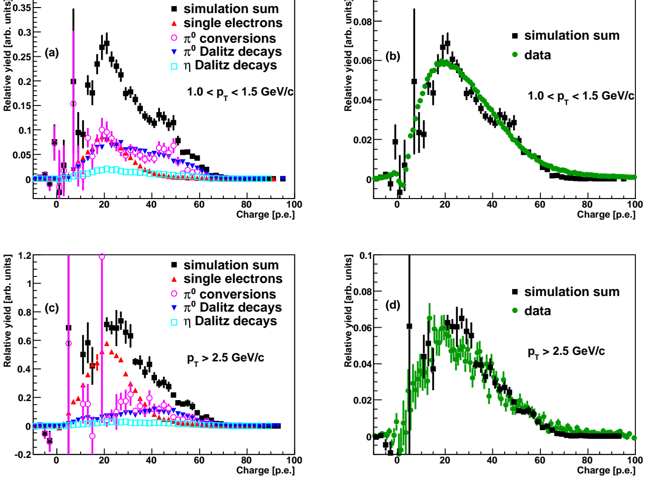
FIG. 4. (Color online) Simulated response of the HBD to different sources of electrons compared to the measured distribution for two different p_T ranges, (a) 1.0 < p_T < 1.5 GeV/c and (c) p_T > 2.5 GeV/c. (black squares) total simulation, (red triangles) single electrons, (blue inverted triangles) \pi^0 Dalitz decays, (open magenta circles) conversions, (open cyan squares) \eta Dalitz decays, and (green circles) data. For visual comparison, in (b) and (d) the distributions are normalized to 1 for the same p_T ranges as in (a) and (c).
