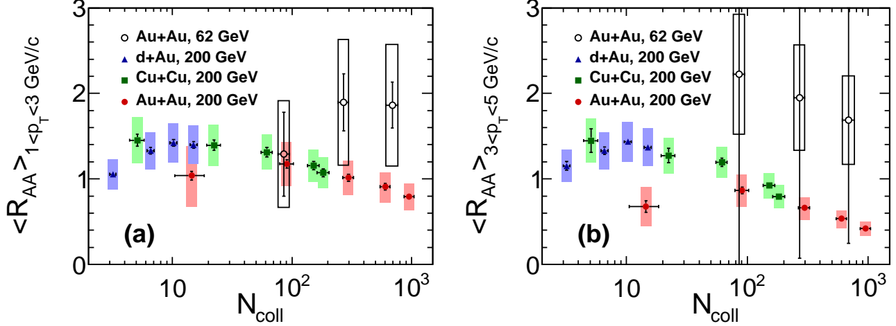
FIG. 17. (Color online) The R_{AA} values for electrons from heavy-flavor decay in Au+Au collisions at 62.4 GeV with the R_{AA} results from d+Au, Cu+Cu, and Au+Au collisions at \sqrt{s_{NN}} = 200 GeV (data from [9, 21]). The error bars (boxes) represent the statistical (systematic) uncertainties. The p_T ranges are as indicated: (a) 1 < p_T < 3 GeV/c and (b) 3 < p_T < 5 GeV/c.
