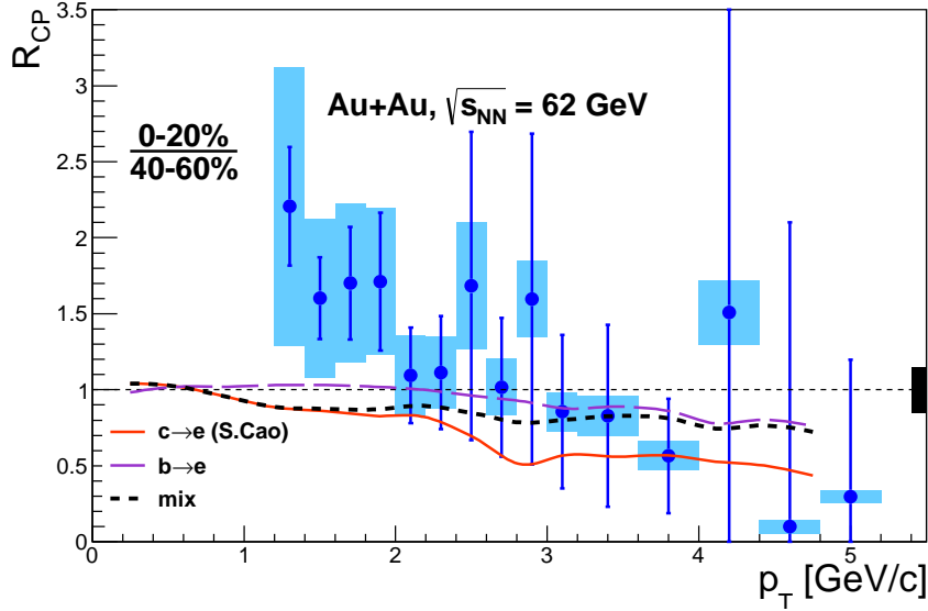
FIG. 20. (Color online) Heavy-flavor electron R_{CP} between centrality 0%–20% and 40%–60% in Au+Au collisions at \sqrt{s_{NN}} = 62.4 GeV. The curves are calculated using a model based on energy loss [46, 47].
