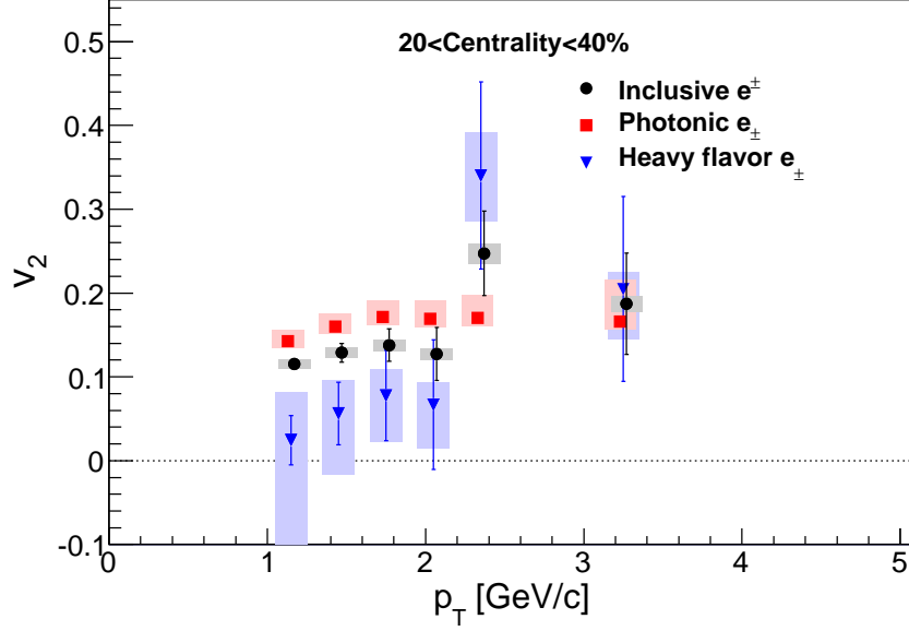
FIG. 21. (Color online) Candidate (inclusive), photonic, and heavy-flavor electron v_2 in Au+Au collisions at \sqrt{s_{NN}} = 62.4 GeV for 20%–40% centrality.
