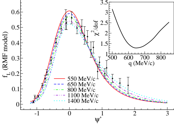
FIG. 7: (Color online) Longitudinal scaling function for (e, e') computed within RMF. Each line correspond to a different momentum transferred (see legend). The scaling functions have been shifted to place the maximum at \psi' = 0 . In the inner smaller plot the reduced- \chi^2 , defined as \chi^2/25 = \frac{1}{25} \sum_{i=1}^{25} [(f_{L,i}^{ee'} - f_{L,i}^{RMF})/\sigma_{L,i}^{exp}]^2 where \sigma_{L,i}^{exp} are the errors of the experimental data, is presented versus q . The minimum \chi^2 is around q = 650 MeV/c. Data from Ref. [9].
