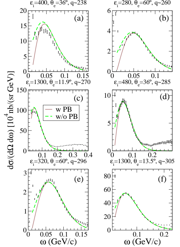
FIG. 17: (Color online) SuSA with and without Pauli Blocking is compared with data. E_{shift} = 10 MeV has been employed.
