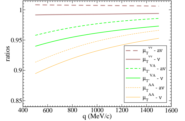
FIG. 8: (Color online) Ratios of transverse scaling functions.
