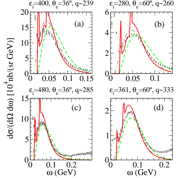
FIG. 9: (Color online) Comparison of inclusive ^{12}\text{C}(e, e') cross sections and predictions of the RMF (red-solid line), SuSA (green-dashed line) and SuSAv2 (brown-dotted-dashed line) models (see text for details). Set of panels corresponding to low- q values. Data taken from [22].
