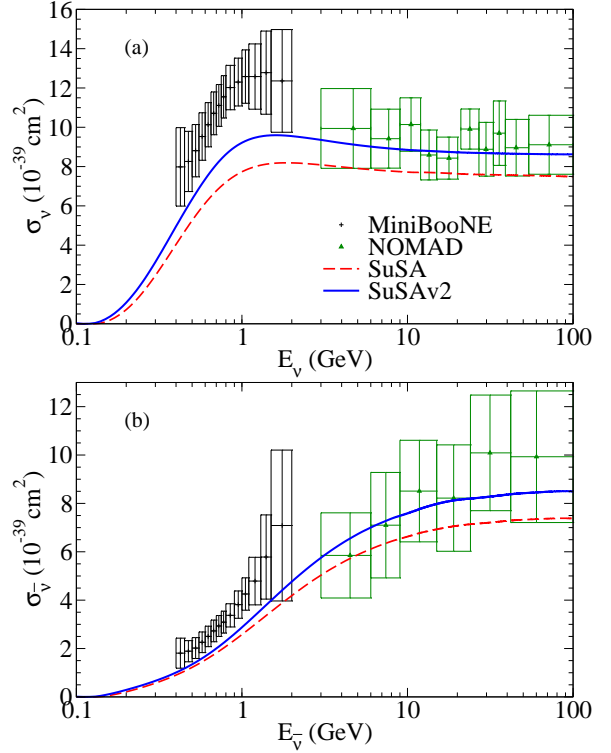
FIG. 14: (Color online) Panel (a): CCQE (\nu, \mu^-) cross section per nucleon is presented as a function of the incident neutrino energy, E_\nu . Data from MiniBooNE [26] and NOMAD [30] are compared with SuSA (dashed-red line) and SuSAv2 (solid-blue line) predictions. Panel (b): As in panel (a), but now for the antineutrino-induced reaction, ^{12}\text{C}(\bar{\nu}, \mu^+) .
