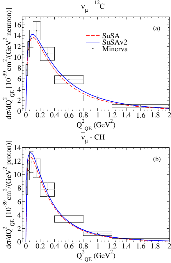
FIG. 15: (Color online) CCQE neutrino (panel (a)) and antineutrino (panel (b)) MINER \nu A data are compared with SuSA (dashed-red line) and SuSAv2 (solid-blue line) predictions. Data taken from [28, 29].
