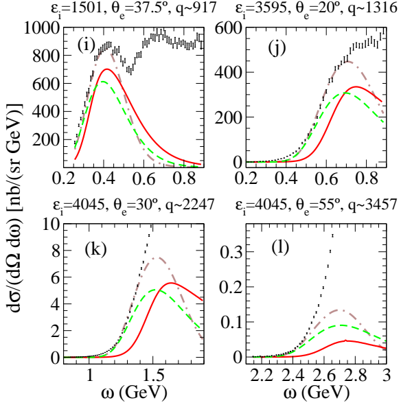
FIG. 11: (Color online) Continuation of Fig. 9. Set of panels corresponding to high- q values.
