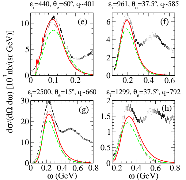
FIG. 10: (Color online) Continuation of Fig. 9. Set of panels corresponding to medium- q values.
