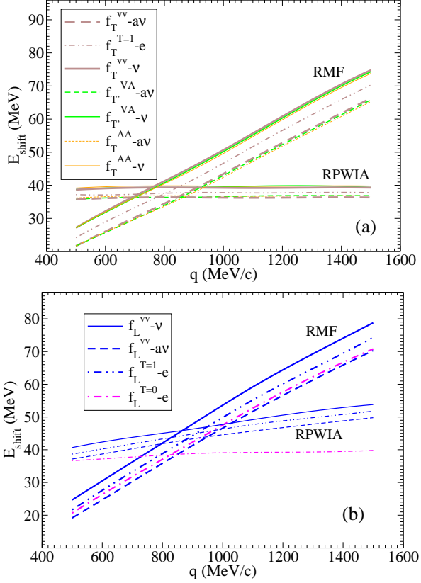
FIG. 5: (Color online) Panel (a): Shift energy, E_{shift} , needed in order to have the corresponding scaling function peak located at \psi' = 0 , as function of q . Results for the transverse set of scaling functions. Panel (b): As for panel (a), but now for the longitudinal set of scaling functions.
