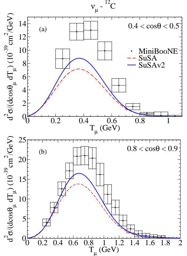
FIG. 12: (Color online) MiniBooNE double differential (\nu, \mu^-) cross section data [26] are compared with SuSA (dashed-red line) and SuSAv2 (solid-blue line) predictions. In panel (a) the scattering angle of the muon is 0.4 < \cos \theta < 0.5 , while in panel (b) 0.8 < \cos \theta < 0.9 .
