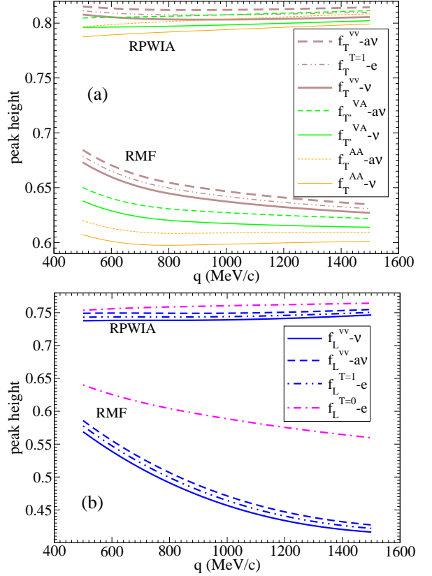
FIG. 4: (Color online) Panel (a): Peak height of the transverse set of scaling functions as a function of the transferred momentum q . The upper set of lines corresponds to the prediction within RPWIA, while the lower set of lines has been obtained with the RMF model. Panel (b): As for the panel (a), but now for the longitudinal set of scaling functions.
