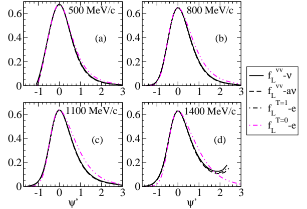
FIG. 2: (Color online) As in Fig. 1, but now for the longitudinal RMF scaling functions.
