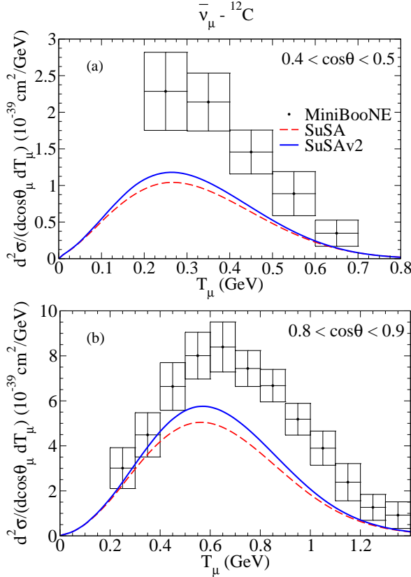
FIG. 13: (Color online) As in Fig. 12, but now for the antineutrino-induced reaction, (\bar{\nu}, \mu^+) . Data taken from [27].
