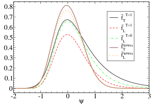
FIG. 16: (Color online) Reference scaling functions in SuSAv2 model.
