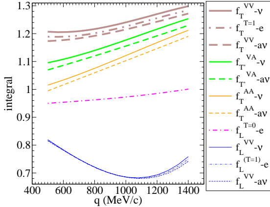
FIG. 6: (Color online) Integrals of RMF scaling functions as functions of q .
