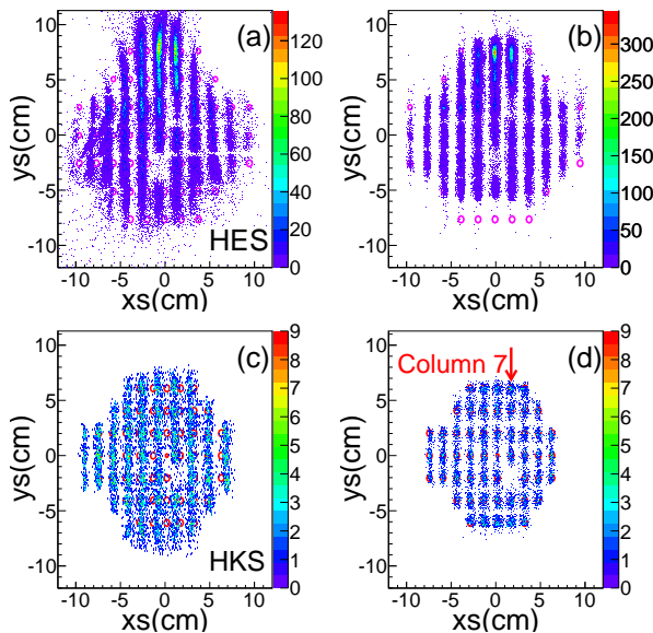
FIG. 5. (Color online) The reconstructed real HES and HKS SS events at the SS plate in comparison to the actual geometry of the SS holes. (a, c) before field correction and (b, d) after field correction.
