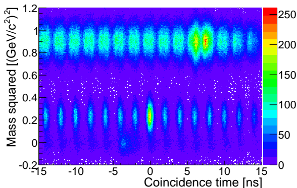
FIG. 3. (Color online) The 2-dimensional correlation between the derived mass squared and the coincidence time without the \text{A}\check{\text{C}} and \text{W}\check{\text{C}} cuts. After the \text{A}\check{\text{C}} and \text{W}\check{\text{C}} cuts, the three rows of pulse trains were clearly separated.
