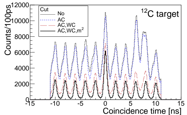
FIG. 2. (Color online) The coincidence time spectra with a sequence of the kaon identification cuts.
