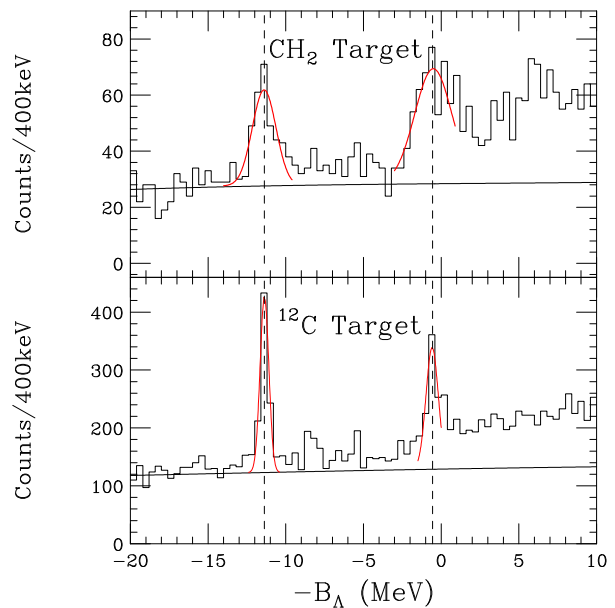
FIG. 9. (Color online) Spectroscopy of ^{12}\Lambda\text{B} obtained by the ^{12}\text{C}(e, e'K^+) reaction from the \text{CH}_2 and ^{12}\text{C} targets from experiment E05-115. The same alignment procedure was followed for E01-011.
