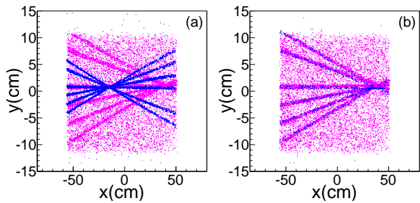
FIG. 4. (Color online) The HKS focal plane Y vs X correlations for the events selected from the 7 th column of the SS holes. Blue - simulated data and Magenta - real data. (a) before field correction and (b) after field correction.
