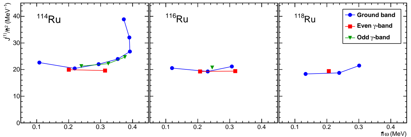
FIG. 5: Kinematic moment-of-inertia, \mathcal{J}^{(1)} , as a function of the rotational frequency, \hbar\omega , for the ground-state and quasi- \gamma bands in ^{114-118}\text{Ru} .
