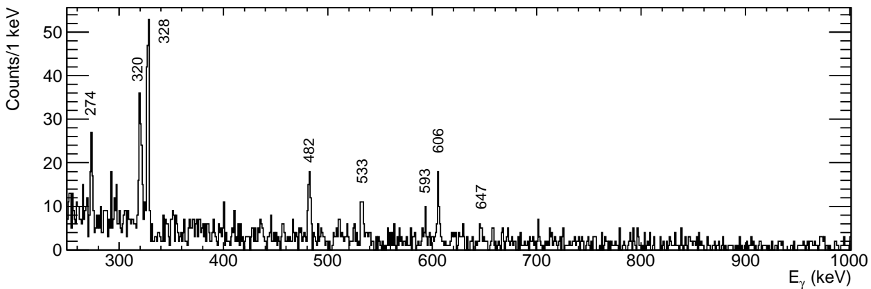
FIG. 2: Spectrum of \gamma -rays following the \beta -decay of ^{118}\text{Tc} . Transitions from excited states in ^{118}\text{Ru} , from this work, has been labeled.
