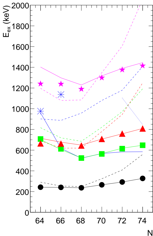
FIG. 10: (Color online) Experimental (symbols) and calculated (lines) energy systematics of the 2_1^+ (black, circles), 2_2^+ (green, squares), 4_1^+ (red, triangles), 0_2^+ (blue, asterisks) and 6_1^+ (magenta, stars) in the Ru isotopes. The solid lines show the IBM-1 fits from this work, while the dashed lines show the IBM-2 calculation from Ref. [11]. Algebraic Collective Model calculations of the 0_2^+ states for N = 72, 74 , see Sec. IV C, are shown as a dashed line.
