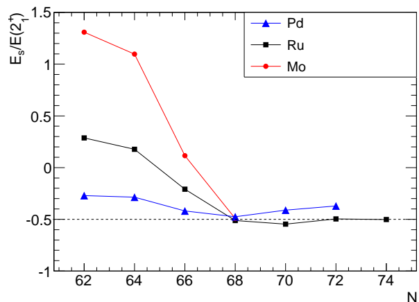
FIG. 7: (Color online) Experimental ratio between the difference between the 2_2^+ and 4_1^+ states, and the energy of the 2_1^+ state, E_2/E(2_1^+) , for the neutron-rich the molybdenum, ruthenium and palladium isotopes.
