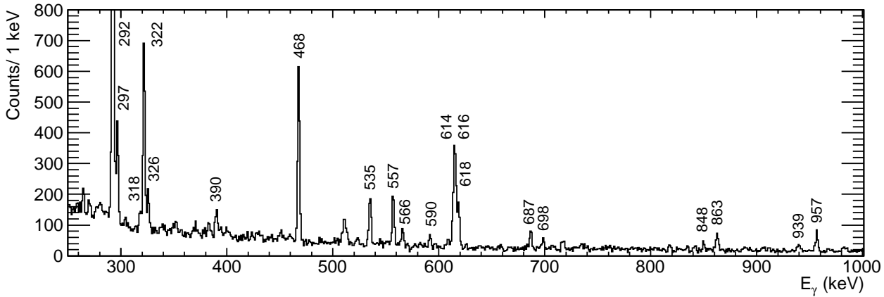
FIG. 1: Spectrum of \gamma -rays following the \beta -decay of ^{116}\text{Tc} . Transitions from excited states in ^{116}\text{Ru} , from this work, has been labeled. The height of the 292 keV \gamma -ray peak is \sim 2100 counts.
