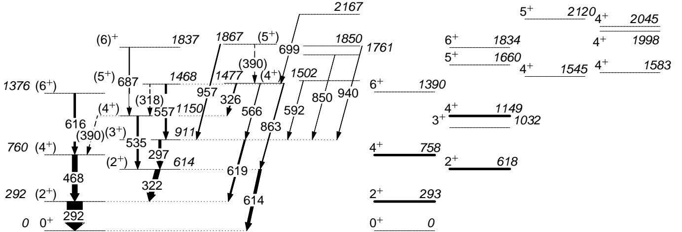
FIG. 3: Experimental level scheme of ^{116}\text{Ru} as obtained in this work (left) and calculated from the IBM-1 model (right). The thickness of the arrows are proportional to the intensities of the \gamma -rays. The thick levels in the IBM-1 level scheme have been used to fit the energies of the model to the experimental data.
