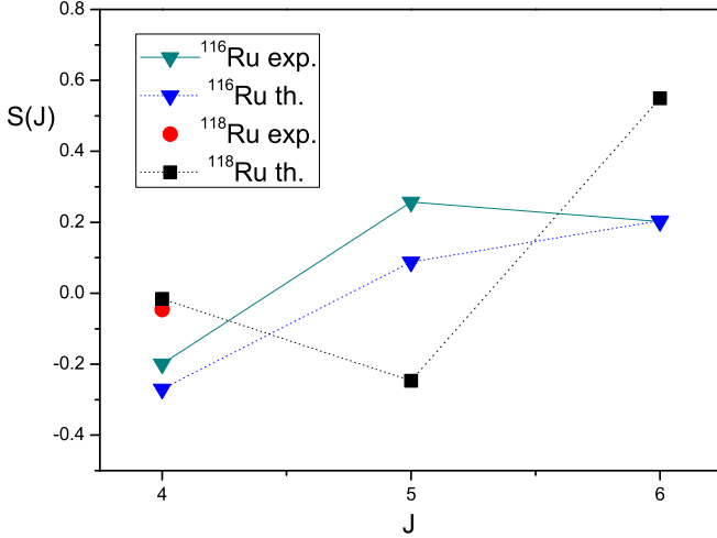
FIG. 12: Energy staggering of the quasi- \gamma band for ^{116}\text{Ru} and ^{118}\text{Ru} .
