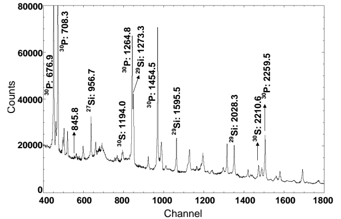
Figure 4: Singles \gamma -ray spectrum measured during phase II of the experiment at 90^\circ using detector 1. Selected strong transitions are labeled by their parent nuclei and with energies (in keV) that are weighted averages between both phases of the experiment. The 2210.6-keV ( 2_1^+ \rightarrow 0_1^+ ) and 1194-keV ( 2_2^+ \rightarrow 2_1^+ ) peaks originate from levels in ^{30}\text{S} .
