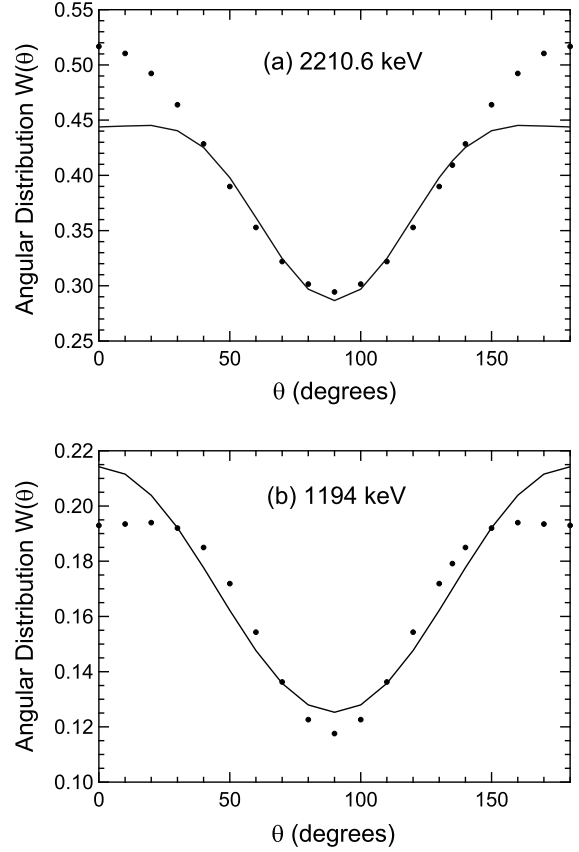
Figure 9: Experimental \gamma -ray angular distributions shown in circles in comparison with the theoretical angular distributions normalized to the data shown with solid lines. The former were obtained from fitting Eq. (7) to relative intensities shown in Fig. 8, and the latter were calculated using Eqs. (2) and (3). The comparison is made for the 2210.6-keV (a) and 1194-keV (b) \gamma -rays. The normalization of the theoretical angular distributions is best performed with \sigma/j = 0.6 and \delta = 0 for the 2210.6-keV \gamma -ray, and with \sigma/j = 0.5 and \delta = 0.16 for the 1194-keV \gamma -ray. The agreement between the theoretical and experimental curves over most of the angles is good for the 2210.6-keV \gamma -ray and less satisfactory for the 1194-keV \gamma -ray (see text). For those angles lower than 40^\circ and higher than 150^\circ , the W(\theta)_{theo}^{norm} diverges significantly from W(\theta)_{exp} due to the lack of data points for normalization at those angles.
