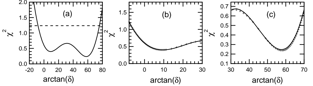
Figure 10: \chi^2 (solid line) vs. \arctan\delta for the 1194-keV \gamma -ray de-exciting the 3404.7-keV state of ^{30}\text{S} (a). The dashed line shows \chi_{min}^2 + 1 , and is therefore our 1\sigma confidence level (see text). Polynomial fits of the 3 rd degree are shown in panels (b) and (c) with solid black lines passing through a selected portion of \chi^2 , denoted by + signs, vs. \arctan\delta .
