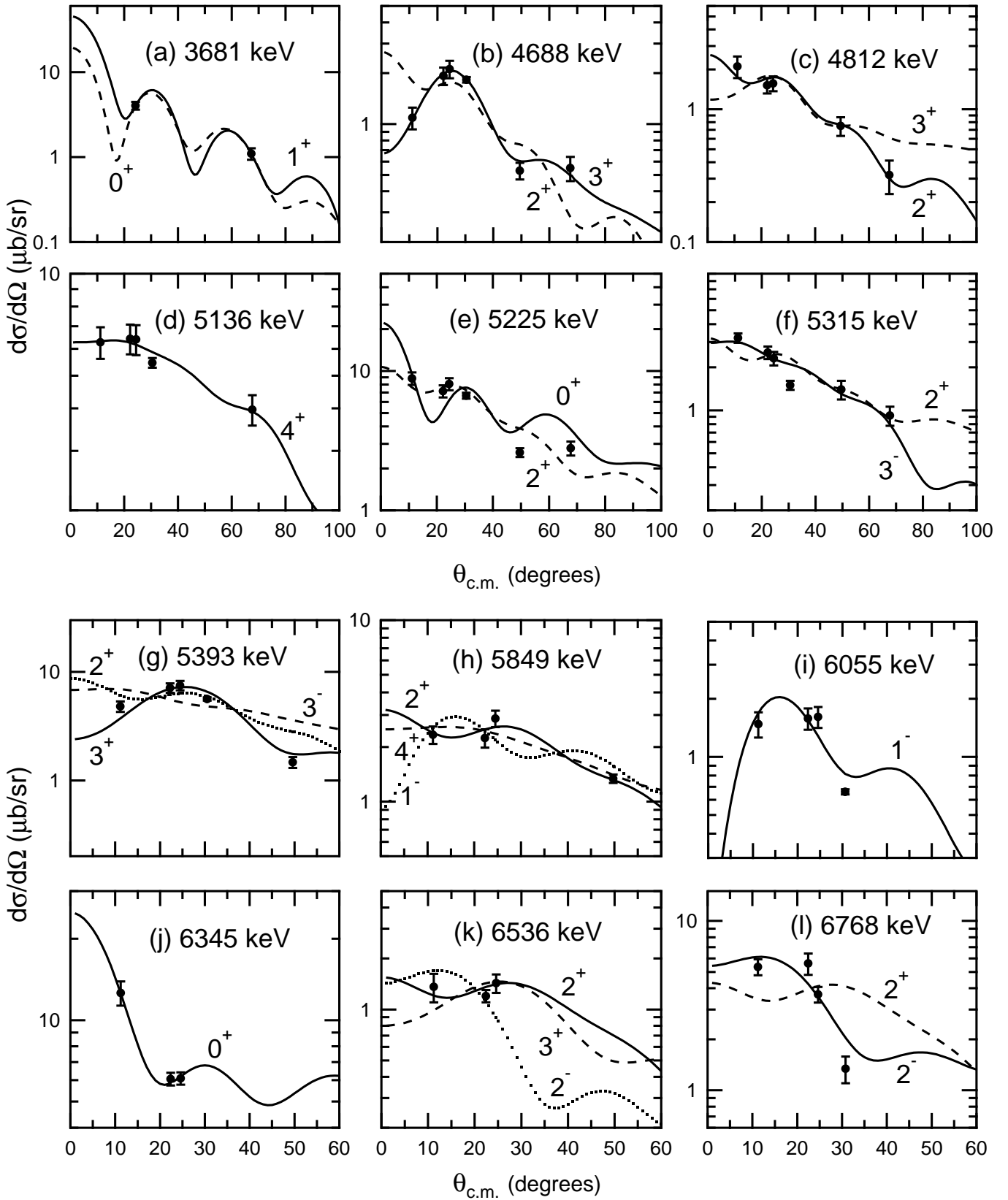
Figure 3: Triton angular distributions populating states of ^{30}\text{S} compared with the DWBA curves for the natural-parity state and multi-step CRC calculations for the unnatural-parity levels. The filled circles with error bars are the measured differential cross sections in the center-of-mass system, and the solid, dashed or dotted curves are the theoretical angular distributions obtained via using FRESKO. If not shown, the error bar is smaller than the point size. The excitation energies are given on the top middle of each plot.
