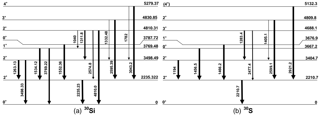
Figure 6: A portion of ^{30}\text{Si} decay scheme [42] (a) in comparison with that of ^{30}\text{S} based on the results of the present work (b). The \gamma -ray branches of these mirror nuclei are not to scale; however, the thicker the arrow, the stronger the branch. All the observed \gamma -rays are shown with their energies (in keV) corrected for the recoil energies of the corresponding ^{30}\text{S} excited states, which are also shown (in keV). The \gamma -ray transitions with energies above 3 MeV in ^{30}\text{S} could not be resolved in our experiments due to the presence of strong ^{30}\text{P} transitions in that region.
