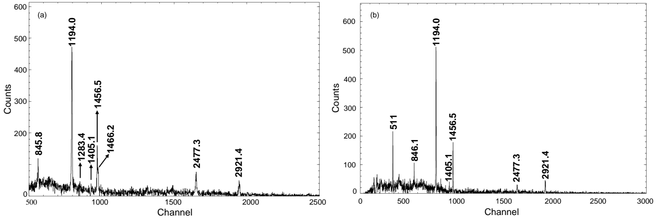
Figure 5: The \gamma - \gamma coincidence spectrum measured during phase II at 90^\circ (a) and 135^\circ (b) obtained from gating on the 2210.6-keV ( 2_1^+ \rightarrow 0_1^+ ) transition of ^{30}\text{S} . Peaks corresponding to the transitions from known ^{30}\text{S} states are labeled with energies (in keV). At 135^\circ , the labeled energies are corrected for Doppler shift except that of the 846.1-keV \gamma -ray (see text). The 2477.1-keV and 2599.5-keV peaks are from the decays of proton-unbound states at 4688.0 keV and 4810.4 keV, respectively.
