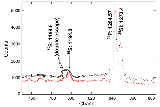
Figure 7: (Color online) The 1194-keV peak together with the double escape peak of the 2210.6-keV line of ^{30}\text{S} . The other two peaks are identified by their parent nucleus and their energy (in keV). The black and red spectra are measured by the 50% and 70% relative efficiency detectors, respectively. For a short time during Phase II of the experiment, these detectors were placed at \pm 90^\circ with respect to the beam axis. The 1188.6-keV transition is the double escape peak of the 2210.6-keV \gamma -ray of ^{30}\text{S} , and its yield has decreased significantly when measured by the larger detector at -90^\circ . The peak corresponding to the 1194-keV \gamma -ray is one of the two that stands out in the spectrum measured by the larger detector at -90^\circ .
