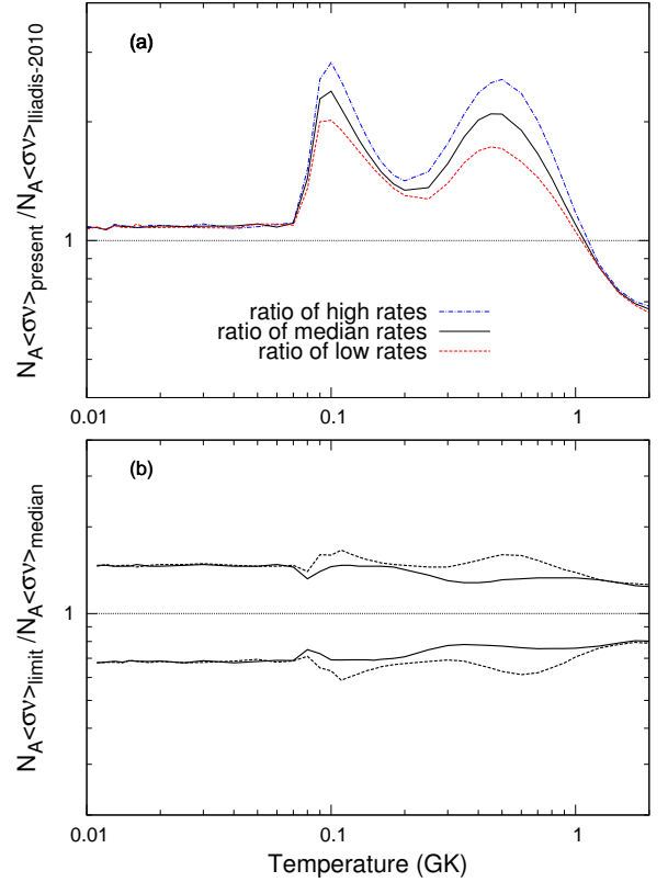
Figure 12: (Color online) The ratio of our Monte Carlo low, median and high rates to those obtained in Ref. [12] (a). Our median rate is 2.3 times larger than that of Ref. [12] at T = 0.1 GK. The uncertainty bands (b) corresponding to N_A < \sigma \nu >_{\text{high}} / N_A < \sigma \nu >_{\text{median}} and N_A < \sigma \nu >_{\text{low}} / N_A < \sigma \nu >_{\text{median}} from our Monte Carlo rate (solid lines) compared to those of Ref. [12] (dashed lines). At T = 0.1 GK, the ratio of the N_A < \sigma \nu >_{\text{high}} / N_A < \sigma \nu >_{\text{low}} from our Monte Carlo rate is 72% smaller than that of the Monte Carlo rate reported in Ref. [12].
