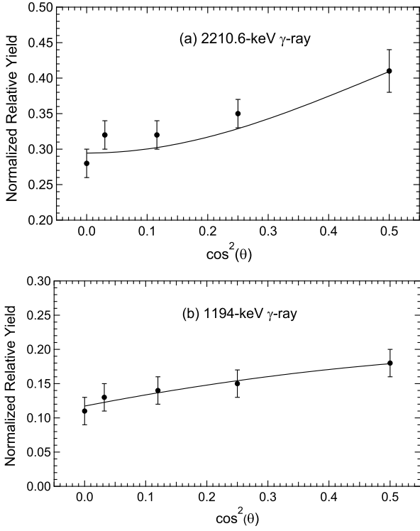
Figure 8: Experimental \gamma -ray angular distributions of the 2210.6-keV (a) and the 1194-keV (b) transitions. Both \gamma -rays are observed in the singles spectra obtained during phase II of the experiment. They correspond to the 2_1^+ \rightarrow 0_1^+ and 2_2^+ \rightarrow 2_1^+ transitions in ^{30}\text{S} , respectively. The solid lines are best fits to Legendre polynomials.
