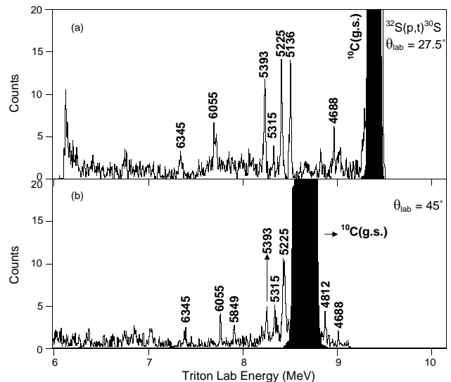
Figure 1: Triton spectra from the ^{32}\text{S}(p,t)^{30}\text{S} reaction measured at 27.5^\circ (a) and 45^\circ (b) obtained with the implanted target. Peaks corresponding to ^{30}\text{S} states are labeled with energies in keV. The filled histograms are background spectra measured with an isotopically enriched ^{12}\text{C} target, normalized to the ^{32}\text{S}(p,t)^{30}\text{S} data. The main contaminant is the ground state (g.s.) of ^{10}\text{C} . For 27.5^\circ , an aluminum plate along the focal plane blocked the region corresponding to tritons with energies higher than 9.5 MeV, where elastically scattered protons reached the focal plane. At 45^\circ the gates cut the region to the right of the peak corresponding to the 4688-keV state.
