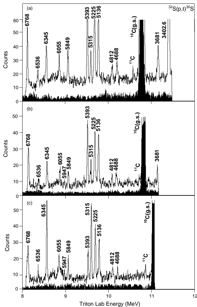
Figure 2: Triton spectra measured (in phase I) from the ^{32}\text{S}(p,t)^{30}\text{S} reaction at 22^\circ (a), 20^\circ (b), and 10^\circ (c) obtained with the CdS target (for details, see Ref. [23]). Peaks corresponding to ^{30}\text{S} states are labeled with energies in keV. The states with E_x > 5.5 MeV were not published in Ref. [23]. The filled histograms are background spectra measured with a ^{111}\text{Cd} target on a carbon backing, normalized to the ^{32}\text{S}(p,t)^{30}\text{S} data. A peak from the ^{13}\text{C}(p,t)^{11}\text{C} reaction is also identified and labeled by its parent nucleus. For 10^\circ and 20^\circ , an aluminum plate along the focal plane blocked the region corresponding to tritons whose energies are higher than 11 MeV, where elastically scattered protons reached the focal plane.
