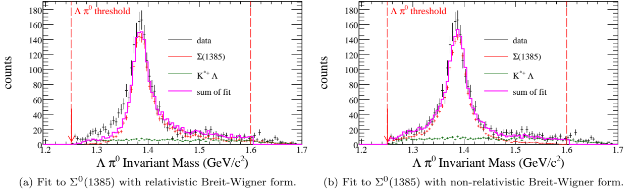
FIG. 14. (Color online) Sample invariant mass spectra for W = 2.6 \text{ GeV} and \cos \theta_{K^+}^{c.m.} = 0.65 showing the \Sigma^0(1385) peak using a Monte Carlo template based on (a) relativistic Breit-Wigner (mass-dependent width) (b) non-relativistic Breit-Wigner (mass-independent width). The fit with the relativistic Breit-Wigner form clearly does not fit the data well.
