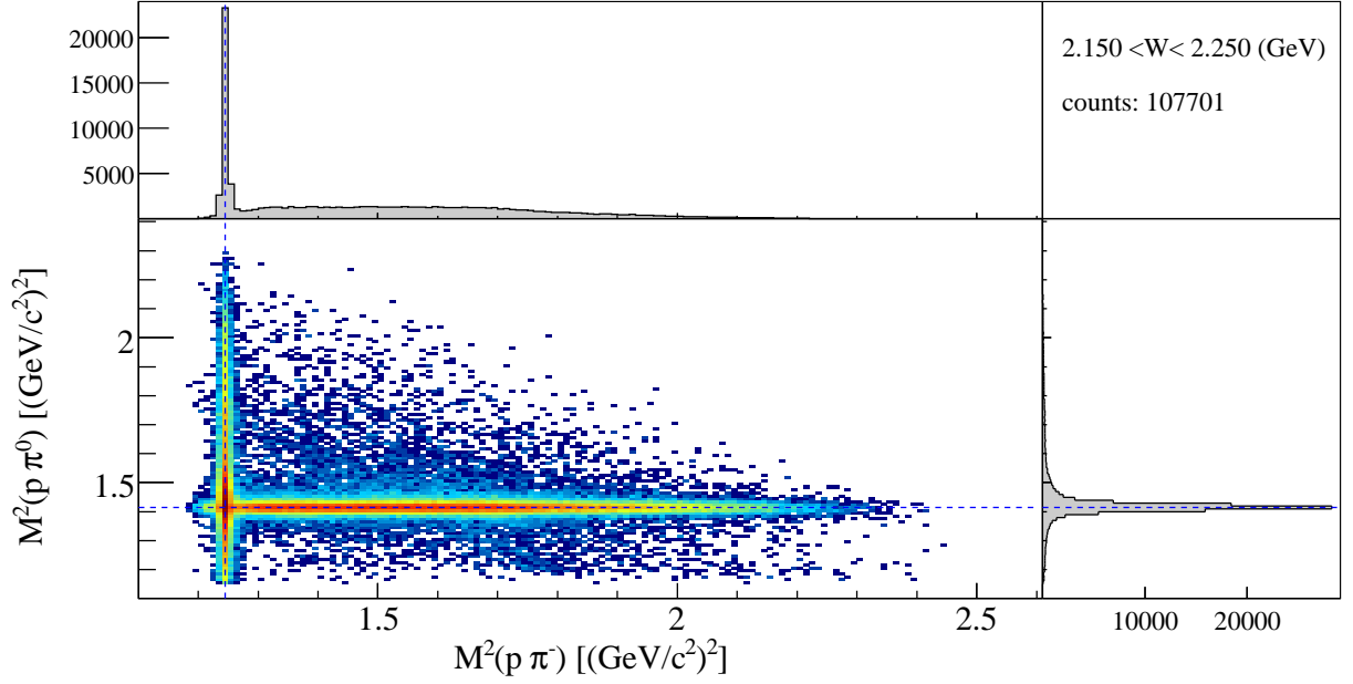
FIG. 5. (Color online) M^2(p\pi^0) versus M^2(p\pi^-) for a given energy bin, with projections. The bands corresponding to the \Lambda (vertical) and \Sigma^+ (horizontal) are clearly seen.
