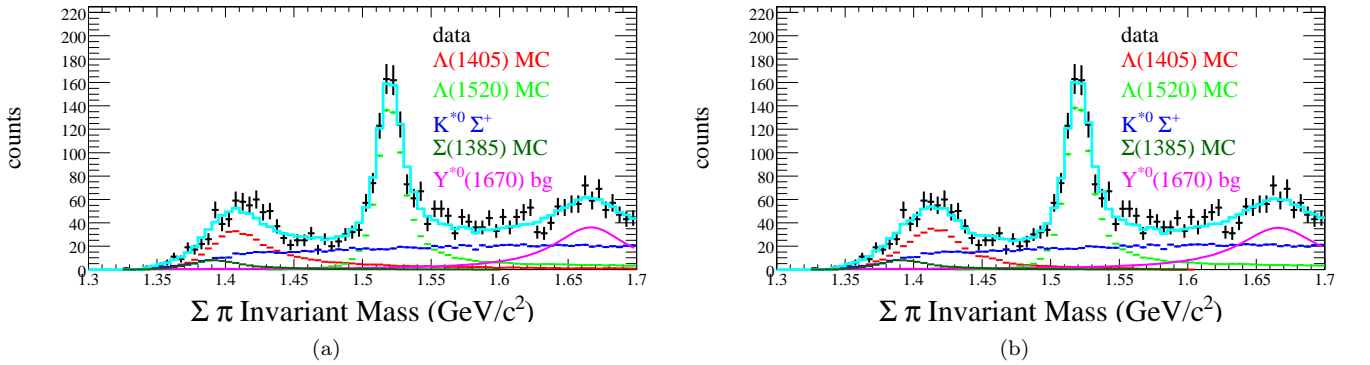
FIG. 15. (Color online) Fit result to the strong final state of \Sigma^+\pi^- before and after Monte Carlo iteration, for W = 2.5 \text{ GeV} , \cos \theta_{K^+}^{c.m.} = 0.35 , as a function of the \Sigma^+\pi^- invariant mass. The data are shown with black crosses. (a) Before iteration. Each Monte Carlo template and the Breit-Wigner function for the Y^*(1670) is shown by a separate color. The total simulation is shown in cyan. (b) After iterations of the \Lambda(1405) template.
