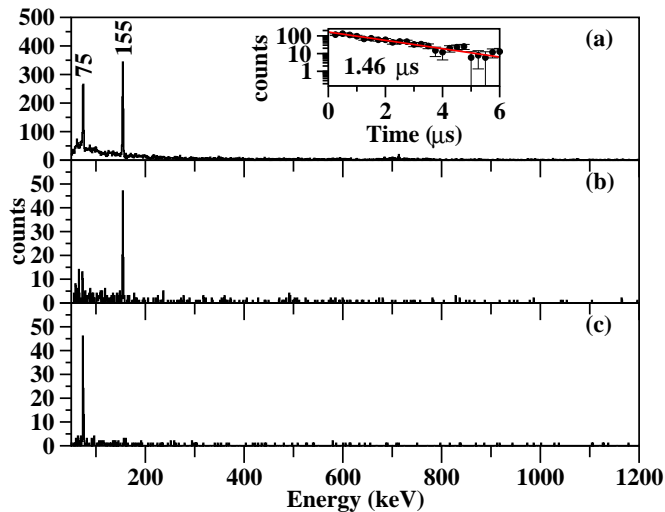
FIG. 12: (color on-line) Gamma-ray energy spectra observed in coincidence with ^{124}\text{Ag} ions. (a) total projection; (b) \gamma -rays in coincidence with the 75-keV transition; (c) \gamma -rays in coincidence with the 155-keV transition; (inset) a summed time spectrum for the 75-keV and the 155-keV transitions.
