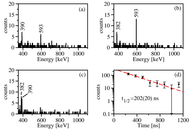
FIG. 4: (color on-line) ^{123}\text{Ag} \gamma -rays, observed in coincidence with the (a) 382-keV, (b) 390-keV, and (c) 593-keV transition, respectively. (d) a summed time spectrum for the three transitions.
