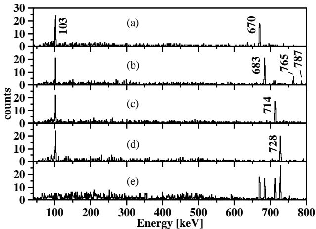
FIG. 7: ^{125}\text{Ag} \gamma -rays, observed in coincidence with the (a) 728-keV, (b) 714-keV, (c) 683-keV, (d) 670-keV, and (e) 103-keV transitions, respectively.
