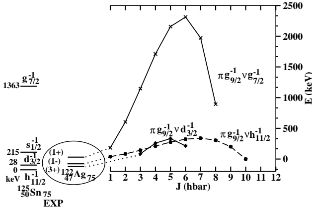
FIG. 17: Proton-neutron quasi-particle multiplets in ^{122}\text{Ag} . Neutron single-particle states in ^{125}\text{Sn} are taken from [44].
