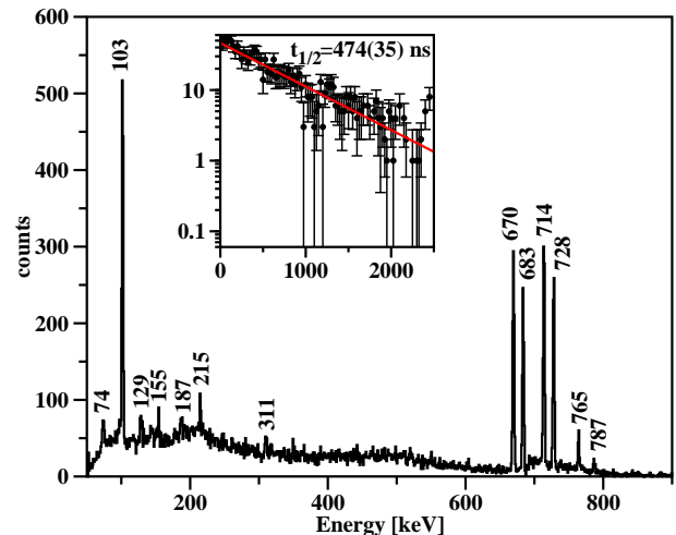
FIG. 6: (color on-line) Gamma-ray energy spectrum, observed in coincidence with the ^{125}\text{Ag} ions. (inset) A summed time spectrum for the 103-keV, 683-keV and 728-keV transitions.
