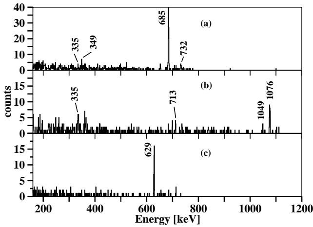
FIG. 2: ^{123}\text{Ag} \gamma -rays, observed in coincidence with the (a) 713-keV, (b) 349-keV and (c) 769-keV transition, respectively.
