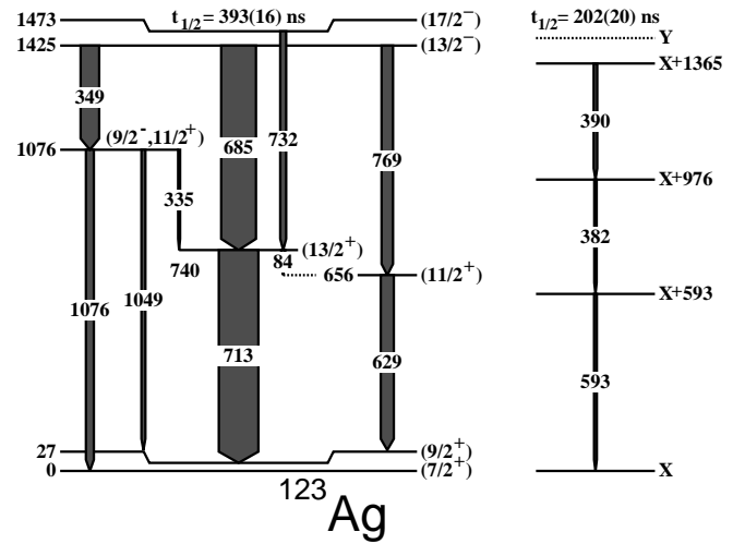
FIG. 3: Partial level scheme of ^{123}\text{Ag} , based on the \gamma -ray coincidences observed in the present work.
