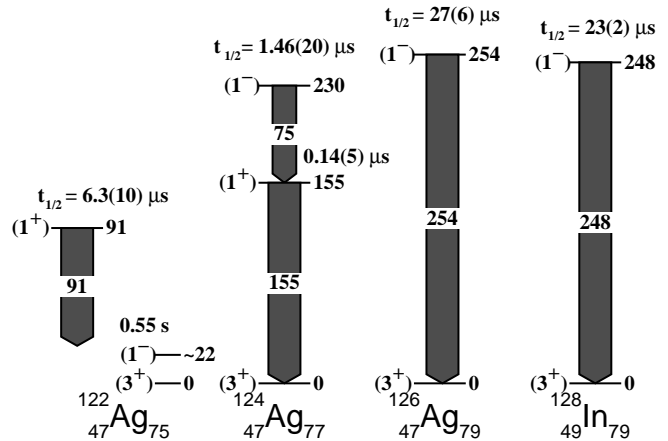
FIG. 10: ^{122,124,126}\text{Ag} level schemes compared to the ^{128}\text{In} level scheme reported in [19]. The (1^-) level in ^{122}\text{Ag} is from [32].
