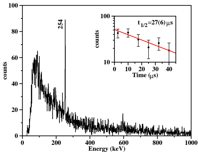
FIG. 14: (color on-line) Gamma-ray energy spectrum observed in delayed coincidence with the ^{126}\text{Ag} ions. (inset) Time spectrum gated on the 254-keV transition.
