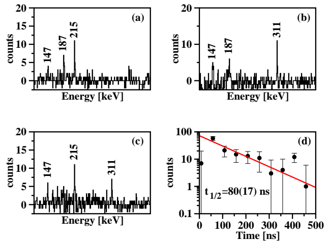
FIG. 9: (color on-line) ^{125}\text{Ag} \gamma -rays, observed in coincidence with the (a) 311-keV, (b) 215-keV and (c) 187-keV transition, respectively. (d) a summed time spectrum for the three transitions.
