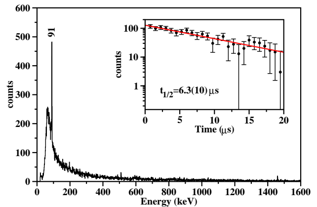
FIG. 11: (color on-line) Gamma-ray energy spectrum observed in coincidence with ^{122}\text{Ag} ions. The inset shows the time distribution of the 91-keV transition.
