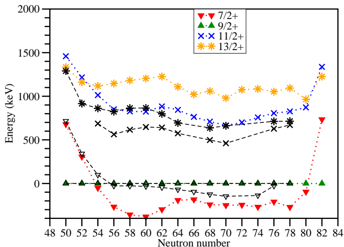
FIG. 15: (color on-line) Evolution of the \pi g_{9/2}^{-3} cluster in odd-A Ag nuclei. The theoretical level energies are plotted with colored symbols and compared to the experimental level energies in black. The same symbols are used for theoretical and experimental levels of a given spin and parity.
