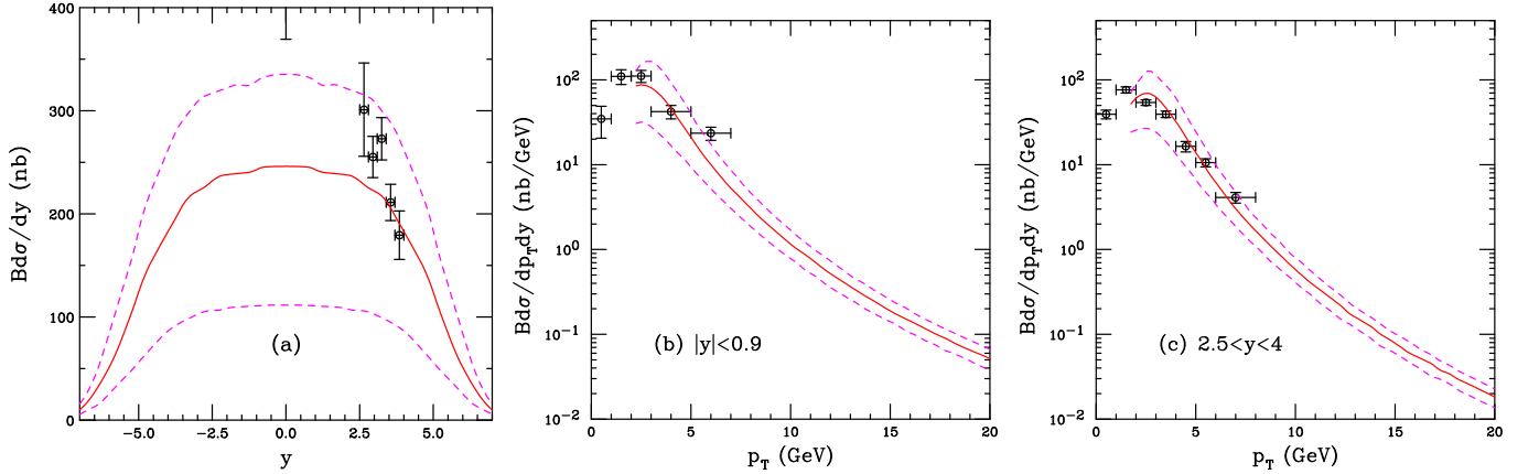
FIG. 12: (Color online) The J/\psi rapidity distribution (a) and the midrapidity, |y| < 0.9 (b), and forward rapidity, 2.5 < y < 4 (c) p_T distributions at \sqrt{s} = 7 TeV and their uncertainties calculated with the same parameters as in Fig. 1(d). The results are compared to the ALICE rapidity distribution as well as the mid and forward rapidity p_T distributions [72]. No additional scaling factor has been applied. The solid red curve shows the central value while the dashed magenta curves outline the uncertainty band. A \langle k_T^2 \rangle kick of 1.49 GeV ^2 is applied to the p_T distributions, as discussed in the text.
