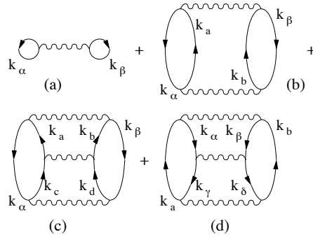
FIG. 4: First-, second-, and third-order diagrams of the Goldstone expansion included in our calculations with V_{NN} vertices only. Latin-letter subscripts denote particle states, greek-letter subscripts correspond to hole states.
