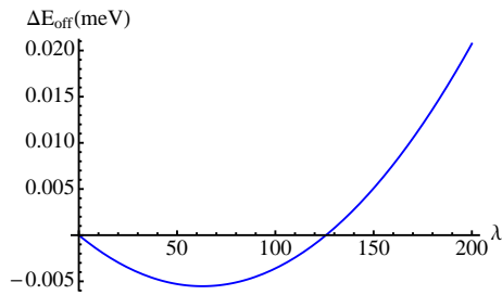
FIG. 2: (Color online) The energy shift \Delta E_{\text{off}} as a function of the parameter \lambda , using Eq. (43).
