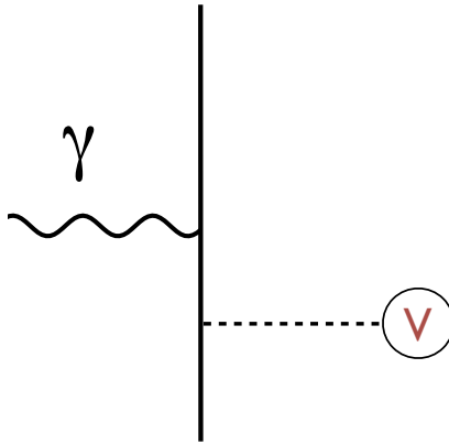
FIG. 1: (Color online) A photon (wiggly line) interacts with a bound nucleon that is off its mass shell because of the interaction V .
