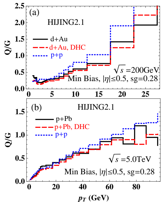
FIG. 3: (color online) (a) Quark to gluon ratio as a function of p_T in p + p (dotted) p(d) + A collisions at the RHIC and (b) LHC energies from HIJING 2.1 without (solid) and with (dashed) de-coherent hard scatterings (DHC).
