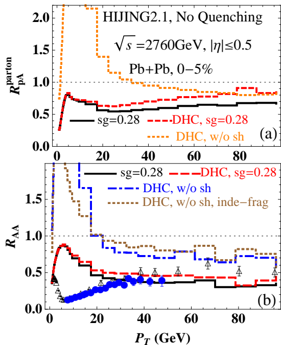
FIG. 6: (color online) (a) Nuclear modification factors for final parton and (b) charged hadrons in central Pb+Pb collisions at \sqrt{s} = 2.76 TeV from HIJING 2.1 with different options: default (solid), DHC (dashed), DHC without parton shadowing (dot-dashed) and DHC without parton shadowing and independent fragmentation (dotted), as compared to data from the ALICE and CMS experiment [28, 29]. Jet quenching due to final-state interaction is not considered in the HIJING calculations.
