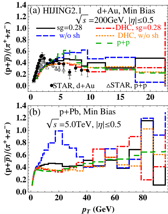
FIG. 4: (color online) (a) Proton to pion ratio at RHIC and (b) LHC from HIJING 2.1 with different options: default (solid), without shadowing (ashed), DHC (dot-dashed), DHC without parton shadowing (dotted) in d + Au collisions at RHIC and p + Pb at LHC. The ratio in p + p collisions is also shown (long dashed). The RHIC experimental data are from STAR [22].
