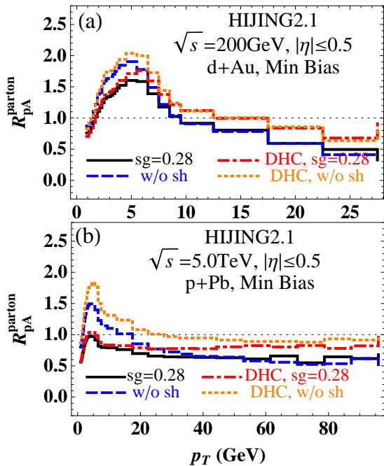
FIG. 2: (color online) (a) Nuclear modification factor for parton p_T spectra in p(d) + A collisions at \sqrt{s_{NN}} = 200 GeV and (b) 5.0 TeV from HIJING 2.1 with (solid), without (dashed) parton shadowing and with de-coherent hard scatterings (DHC) (dot-dashed and dotted).
