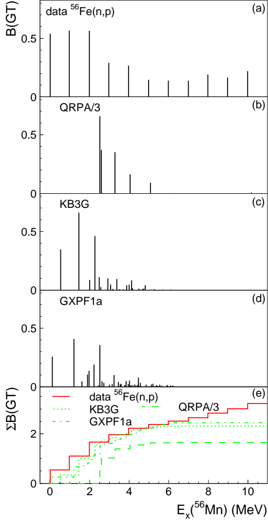
FIG. 13. (Color online) GT transitions from ^{56}\text{Fe} to ^{56}\text{Mn} : (a) from (n,p) data, (b) from calculations in QRPA (divided by a factor of 3), (c) from shell-model calculations using the KB3G interaction and (d) from shell-model calculations using the GXPF1a interaction. In (e), running sums of B(GT) as a function of excitation energy are plotted.
