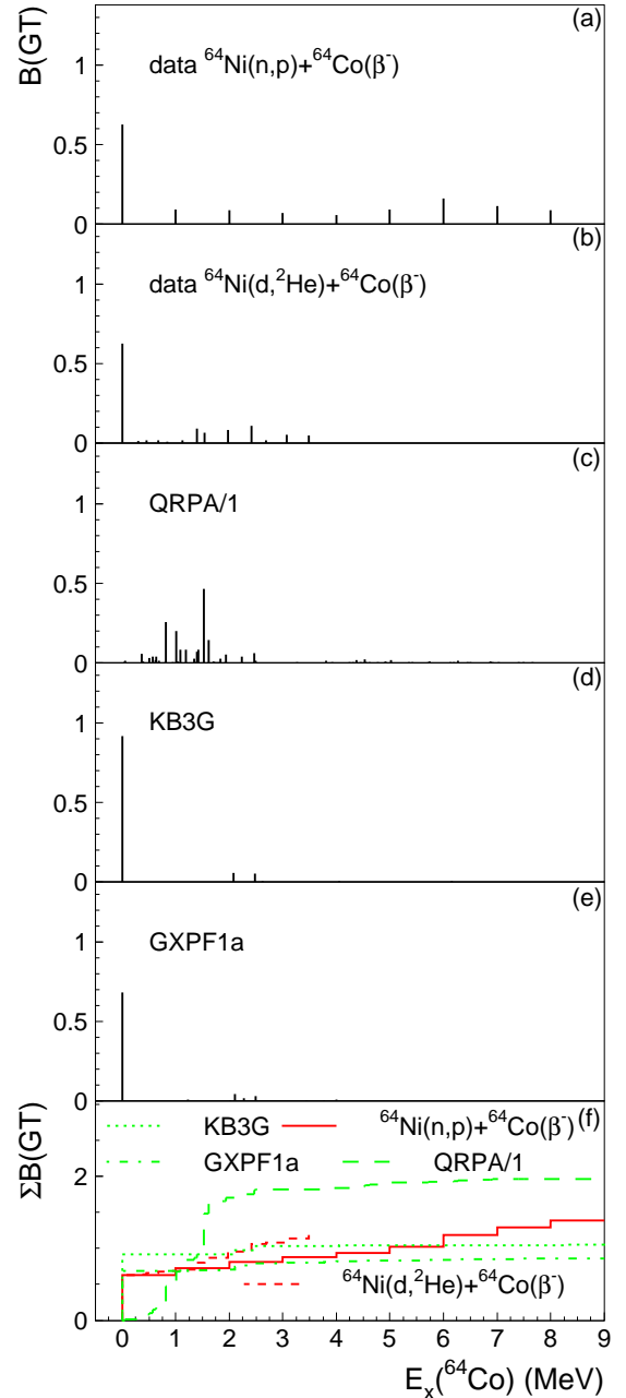
FIG. 23. (Color online) GT transitions from ^{64}\text{Ni} to ^{64}\text{Co} : (a) from ( n,p ) and \beta -decay data, (b) from ( d,^2\text{He} ) and \beta -decay data, (c) from calculations in QRPA, (d) from shell-model calculations using the KB3G interaction and (e) from shell-model calculations using the GXPF1a interaction. In (f), running sums of B(GT) as a function of excitation energy are plotted.
