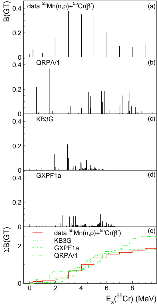
FIG. 11. (Color online) GT transitions from ^{55}\text{Mn} to ^{55}\text{Cr} : (a) from (n,p) and \beta -decay data, (b) from calculations in QRPA, (c) from shell-model calculations using the KB3G interaction and (d) from shell-model calculations using the GXPF1a interaction. In (e), running sums of B(GT) as a function of excitation energy are plotted.
