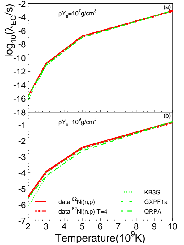
FIG. 22. (Color online) Electron-capture rates for ^{62}\text{Ni}(e^-, \nu_e)^{62}\text{Co} for experimental and theoretical GT strengths, plotted as a function of temperature at two densities, \rho Y_e = 10^7 \text{ g/cm}^3 (a) and \rho Y_e = 10^9 \text{ g/cm}^3 (b).
