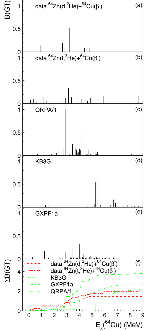
FIG. 25. (Color online) GT transitions from ^{64}\text{Zn} to ^{64}\text{Cu} : (a) from (d, ^2\text{He}) and \beta -decay data, (b) from (t, ^3\text{He}) and \beta -decay data, (c) from calculations in QRPA, (d) from shell-model calculations using the KB3G interaction and (e) from shell-model calculations using the GXPF1a interaction. In (f), running sums of B(GT) as a function of excitation energy are plotted.
