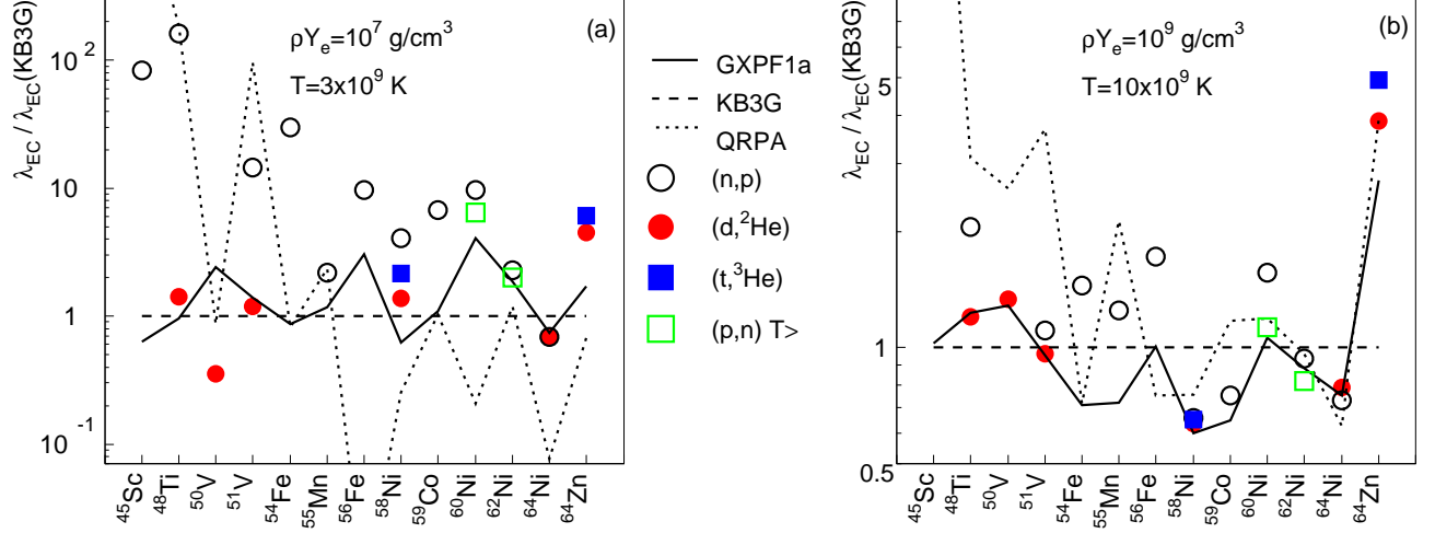
FIG. 27. (Color online) Comparison of EC rates for 13 pf -shell nuclei calculated on the basis of theoretical (connected by lines) and experimental (indicated by markers) GT strength distributions. All rates are plotted relative to those calculated by in the shell-model with the KB3G interaction (for which the relative rate thus equals unity). The relative EC rates are shown for two combinations of stellar density and temperature: (a) \rho Y_e = 10^7 \text{ g/cm}^3 and T = 3 \times 10^9 \text{ K} and (b) \rho Y_e = 10^9 \text{ g/cm}^3 T = 10 \times 10^9 \text{ K} .
