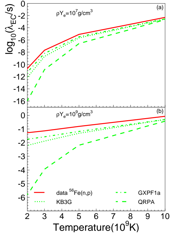
FIG. 14. (Color online) Electron-capture rates for ^{56}\text{Fe}(e^-, \nu_e)^{56}\text{Mn} based on experimental and theoretical GT strengths plotted in Fig. 13, as a function of temperature at two densities, \rho Y_e = 10^7 \text{ g/cm}^3 (a) and \rho Y_e = 10^9 \text{ g/cm}^3 (b).
