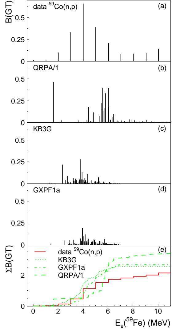
FIG. 17. (Color online) GT transitions from ^{59}Co to ^{59}Fe : (a) from (n,p) data, (b) from calculations in QRPA (without additional scaling), (c) from shell-model calculations using the KB3G interaction and (d) from shell-model calculations using the GXPF1a interaction. In (e), running sums of B(GT) as a function of excitation energy are plotted.
