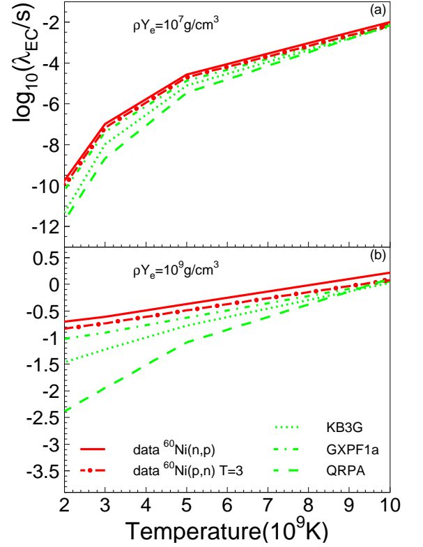
FIG. 20. (Color online) Electron-capture rates for ^{60}\text{Ni}(e^-, \nu_e)^{60}\text{Co} for experimental and theoretical GT strengths plotted in Fig. 19, as a function of temperature at two densities, \rho Y_e = 10^7 \text{ g/cm}^3 (a) and \rho Y_e = 10^9 \text{ g/cm}^3 (b).
