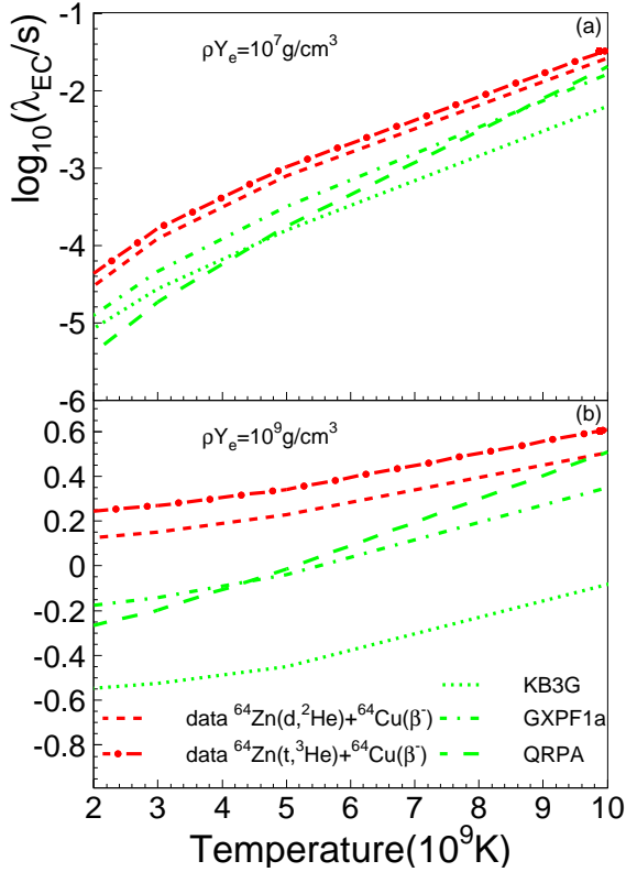
FIG. 26. (Color online) Electron-capture rates for {}^{64}\text{Zn}(e^-, \nu_e){}^{64}\text{Cu} for experimental and theoretical GT strengths shown in Fig. 25, plotted as a function of temperature at two densities, \rho Y_e = 10^7 \text{ g/cm}^3 (a) and \rho Y_e = 10^9 \text{ g/cm}^3 (b).
