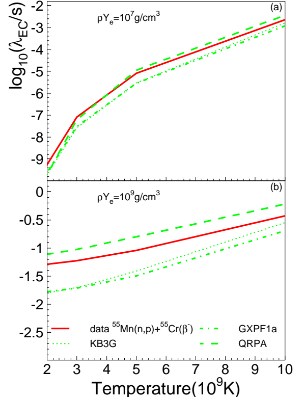
FIG. 12. (Color online) Electron-capture rates for ^{55}\text{Mn}(e^-, \nu_e)^{55}\text{Cr} based on experimental and theoretical GT strengths shown in Fig. 11, plotted as a function of temperature at two densities, \rho Y_e = 10^7 \text{ g/cm}^3 (a) and \rho Y_e = 10^9 \text{ g/cm}^3 (b).
