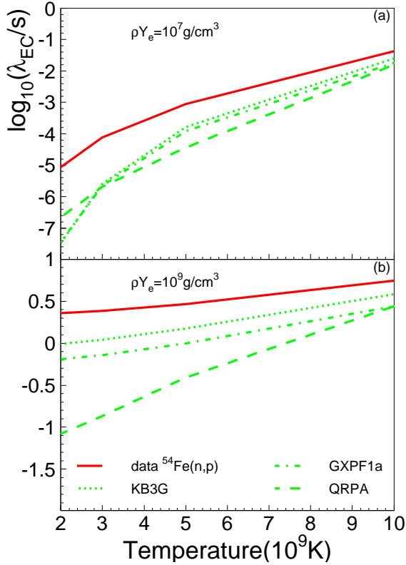
FIG. 10. (Color online) Electron-capture rates for ^{54}\text{Fe}(e^-, \nu_e)^{54}\text{Mn} based on experimental and theoretical GT strengths shown in Fig. 9. plotted as a function of temperature at two densities, \rho Y_e = 10^7 \text{ g/cm}^3 (a) and \rho Y_e = 10^9 \text{ g/cm}^3 (b).
