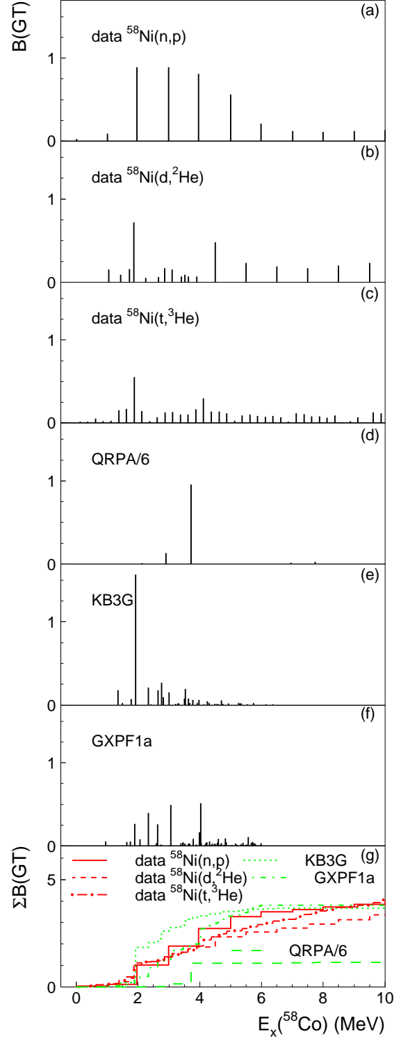
FIG. 15. (Color online) GT transitions from ^{58}\text{Ni} to ^{58}\text{Co} : (a) from (n, p) data, (b) from (d, ^2\text{He}) data, (c) from (t, ^3\text{He}) data (d) from calculations in QRPA (divided by a factor of 6), (e) from shell-model calculations using the KB3G interaction and (f) from shell-model calculations using the GXPF1a interaction. In (g), running sums of B(GT) as a function of excitation energy are plotted.
