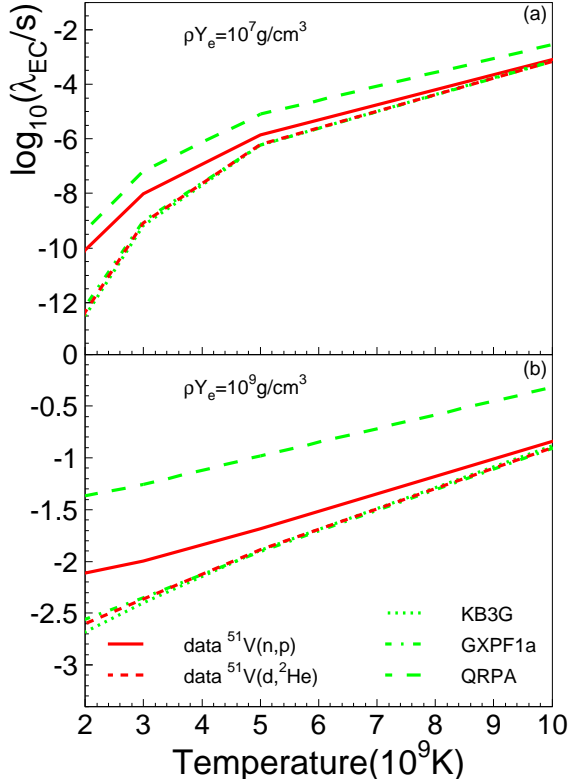
FIG. 8. (Color online) Electron-capture rates for ^{51}\text{V}(e^-, \nu_e)^{51}\text{Ti} , based on experimental and theoretical GT strength distributions shown in Fig. 7, plotted as a function of temperature at two densities, \rho Y_e = 10^7 g/cm ^3 (a) and \rho Y_e = 10^9 g/cm ^3 (b). Note that the rates based on the shell-model calculations with the KB3G and GXPF1a interactions overlap.
