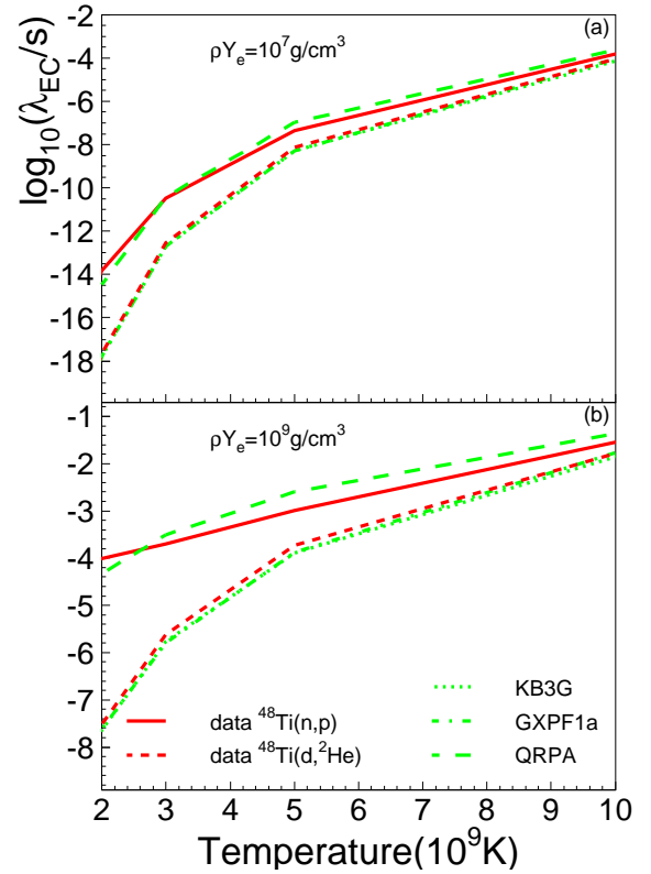
FIG. 4. (Color online)Electron-capture rates for ^{48}\text{Ti}(e^-, \nu_e)^{48}\text{Sc} , based on experimental and theoretical GT strength distributions shown in Fig. 3, plotted as a function of temperature at two densities, \rho Y_e = 10^7 \text{ g/cm}^3 (a) and \rho Y_e = 10^9 \text{ g/cm}^3 (b). Note that the rates based on the shell-model calculations with the KB3G and GXPF1a interactions overlap.
