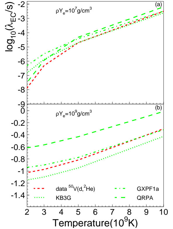
FIG. 6. (Color online) Electron-capture rates for ^{50}\text{V}(e^-, \nu_e)^{50}\text{Ti} based on experimental and theoretical GT strength shown in Fig. 5GT, plotted as a function of temperature at two densities, \rho Y_e = 10^7 \text{ g/cm}^3 (a) and \rho Y_e = 10^9 \text{ g/cm}^3 (b).
