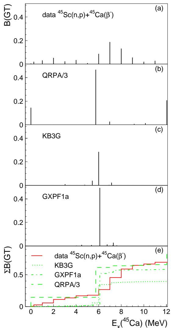
FIG. 1. (Color online) GT transitions from ^{45}\text{Sc} to ^{45}\text{Ca} : (a) from (n,p) and \beta -decay data, (b) from calculations in QRPA (divided by a factor of 3), (c) from shell-model calculation using the KB3G interaction and (d) from shell-model calculations using the GXPF1a interaction. In (e), running sums of B(\text{GT}) as a function of excitation energy are plotted. Here, and all similar graphs, the shell-model strengths have been scaled by (0.74)^2 (see text).
