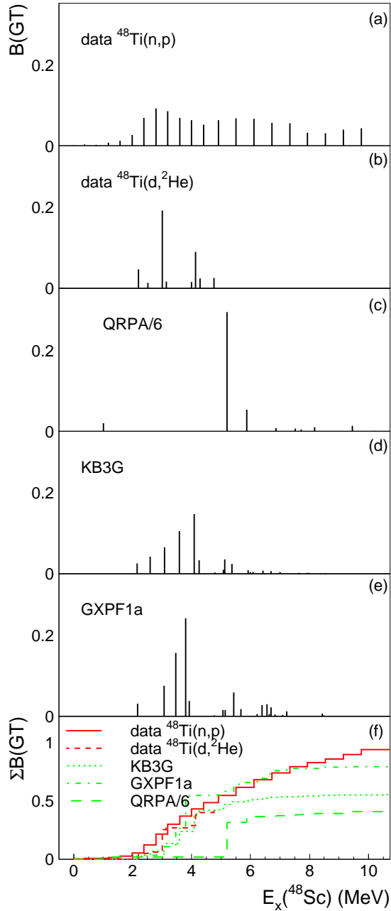
FIG. 3. (Color online)GT transitions from ^{48}\text{Ti} to ^{48}\text{Sc} : (a) from (n,p) , (b) from (d,^2\text{He}) data, (c) from calculations in QRPA (divided by a factor of 6), (d) from shell-model calculations using the KB3G interaction and (e) from shell-model calculation using the GXPF1a interaction. In (f), running sums of B(GT) as a function of excitation energy are plotted.
