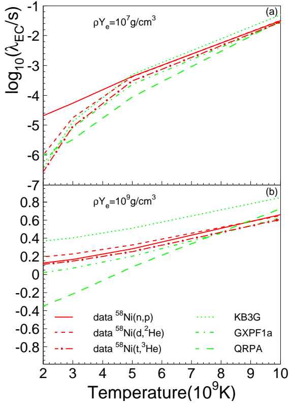
FIG. 16. (Color online) Electron-capture rates for ^{58}Ni(e^-, \nu_e)^{58}Co based on experimental and theoretical GT strengths from Fig. 15, plotted as a function of temperature at two densities, \rho Y_e = 10^7 g/cm^3 (a) and \rho Y_e = 10^9 g/cm^3 (b).
