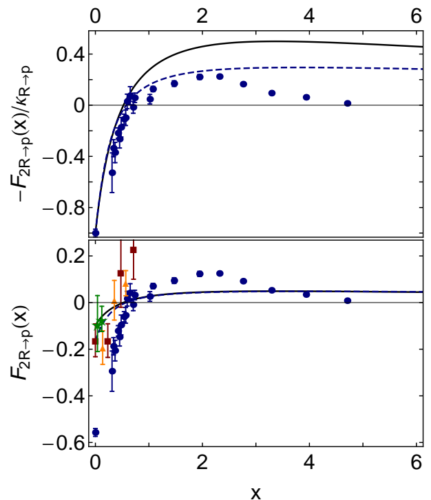
FIG. 11. Comparison between F_{2*}(x) computed using the framework described herein and available data [18–20], with x = Q^2/m_N^2 . Upper panel – normalised to unity at x = 0 ; and lower panel , as computed. In both panels the dashed curve was computed with a model for the dressed-quark anomalous electromagnetic moment, Sec.V. The squares, triangles and stars are preliminary results from a simulation of N_f = 2 + 1 lattice-QCD at, respectively, m_\pi^2/m_{\pi\text{expt.}}^2 \simeq 8, 10, 40 [62].
