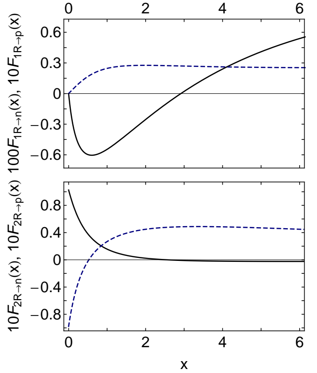
FIG. 13. Upper panel – F_{1R^0 \rightarrow n} (solid) as a function of x = Q^2/m_N^2 compared with F_{1R^+ \rightarrow p} (dashed), computed using the framework described herein. Lower panel – Analogue for F_{2R^0 \rightarrow n} .
