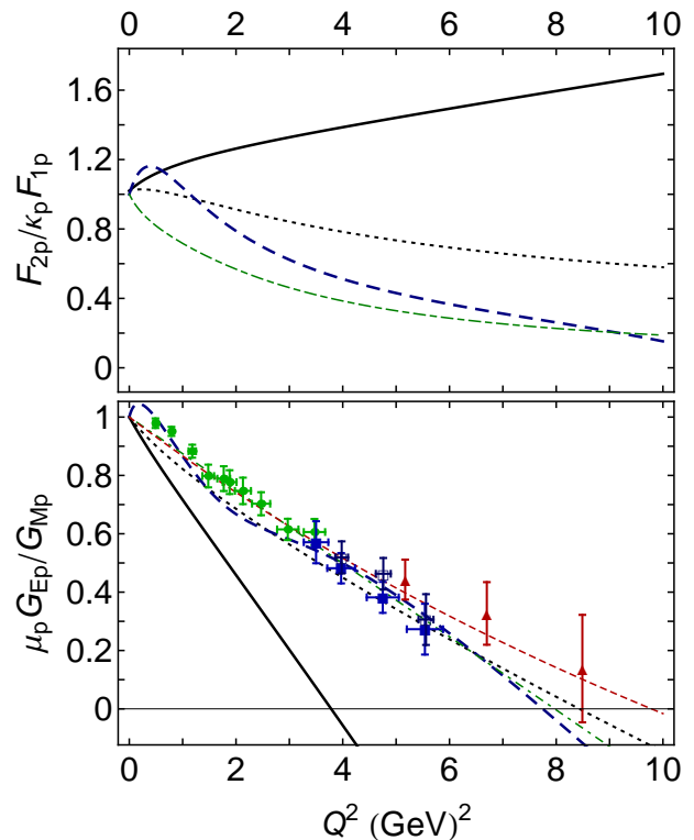
FIG. 7. Upper panel: Normalised ratio of proton Pauli and Dirac form factors. Solid curve – contact interaction; long-dashed curve – result from Ref. [41], which employed QCD-like momentum-dependence for the dressed-quark propagators and diquark Bethe-Salpeter amplitudes; long-dash-dotted curve – drawn from parametrisation of experimental data in Ref. [35]; and dotted curve – softened contact-interaction result, described in connection with Eq. (6). Lower panel: Normalised ratio of proton Sachs electric and magnetic form factors. Solid curve and long-dashed curve , as above; dot-dashed curve – linear fit to data in Refs. [51–55], constrained to one at Q^2 = 0 ; short-dashed curve – [1, 1]-Padé fit to that data; and dotted curve – softened contact-interaction result, described in connection with Eq. (6). In addition, we have represented a selection of data explicitly: filled-squares [52]; circles [54]; up-triangles [55]; and open-squares [56].
