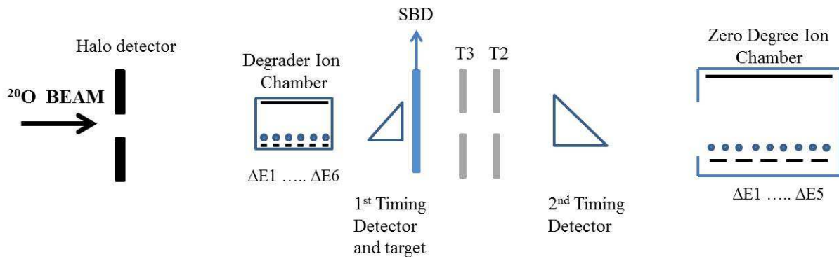
FIG. 1: (Color online) Experimental setup used to measure the fusion of incident ^{20}\text{O} ions with ^{12}\text{C} target nuclei.
