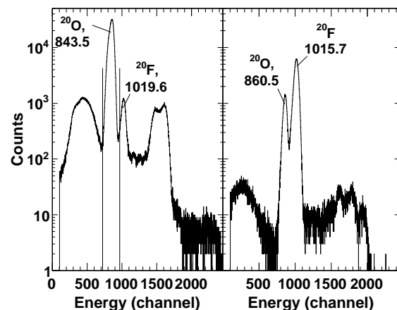
FIG. 2: Left panel: Energy spectra from one of the anodes of the degrader ionization chamber CID with the incident ^{20}\text{O} beam. Right panel: Energy spectra from the same CID anode when the CIME cyclotron was tuned to ^{20}\text{F} at the end of the experiment.
