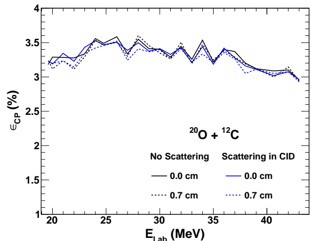
FIG. 6: (Color online) Efficiency for detecting the residue and light charged particle
