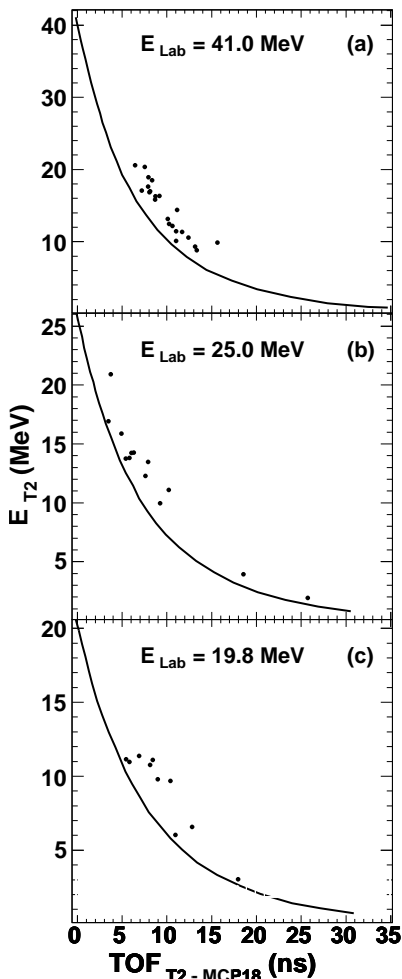
FIG. 5: Energy-TOF spectra of particles in the T2 detector observed in coincidence with a charged particle in T3. The solid line indicates the position of the slit-scatter line observed in Fig. 3.
