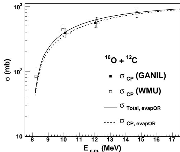
FIG. 10: Measured fusion cross-sections from the reaction ^{16}\text{O} + ^{12}\text{C} associated with charged particle emission channels (solid points) compared to the predictions of the evapOR model. The total predicted fusion cross-section is shown as a solid line while the cross-section predicted for the charged particle channels is represented by the dashed line. Also shown as open symbols is the fusion cross-section of ^{20}\text{O} + ^{12}\text{C} . Horizontal error bars on the data points measured at GANIL reflect the energy dispersion due to degrading the incident beam.
