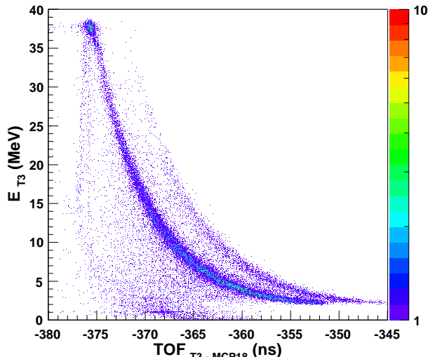
FIG. 4: (Color online) Two dimensional energy-TOF spectrum for particles detected in the T3 detector.
