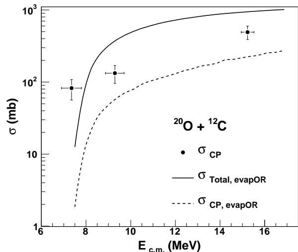
FIG. 8: Measured fusion cross-sections associated with charged particle emission channels (solid points) compared to the predictions of the evapOR model. The total predicted fusion cross-section is shown as a solid line while the cross-section predicted for the charged particle channels is represented by the dashed line. Horizontal error bars on the data points reflect the energy dispersion due to degrading the incident beam.
