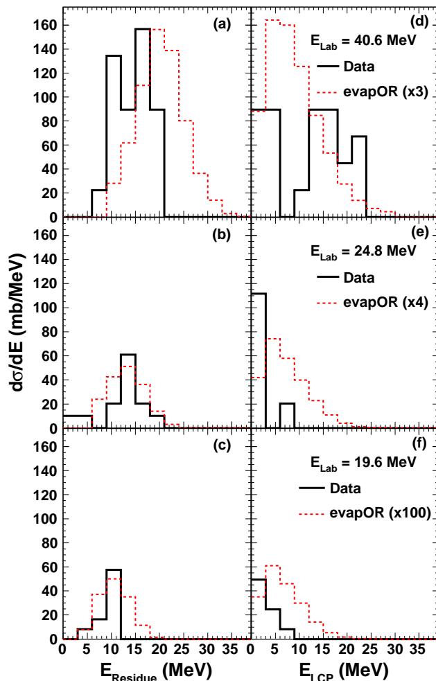
FIG. 7: (Color online) Energy distribution of light charged particles and residues compared to predictions of the statistical model evapOR
