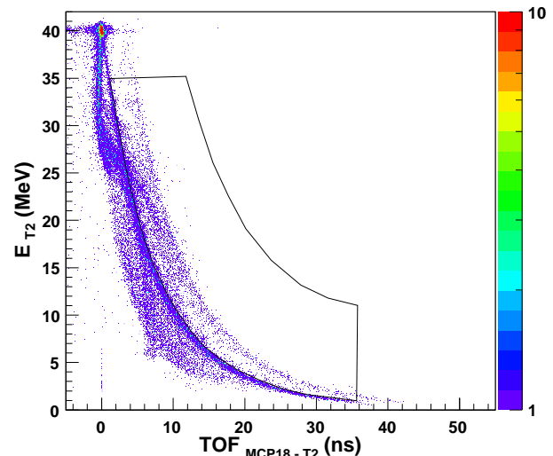
FIG. 3: (Color online) Two dimensional energy-TOF spectrum for particles detected in the T2 detector. The polygonal gate indicates the region used to search for coincidences between evaporation residues in T2 and light charged particles in T3. See text for details.
