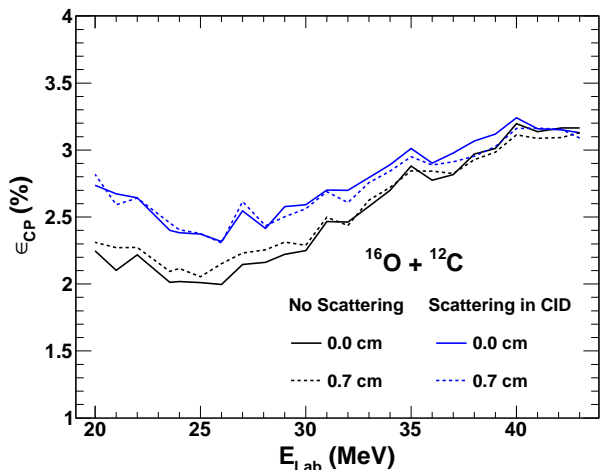
FIG. 9: (Color online) Efficiency for detecting the residue and light charged particle in the reaction ^{16}\text{O} + ^{12}\text{C} measured at GANIL.
