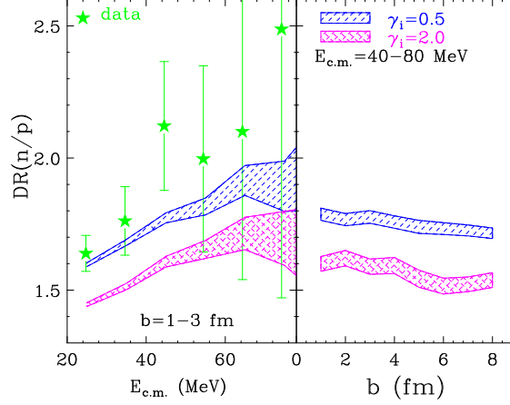
FIG. 5. (Color online) (Left panel) Double n/p yield ratios, DR(n/p) , from transverse emitted nucleons as a function of kinetic energy. The solid stars are data from Ref. [27]. (Right panel) DR(n/p) from transverse emitted high kinetic energy nucleons ( E_{c.m.} > 40 MeV ) as a function of impact parameter. The upper shaded region is for \gamma_i = 0.5 and the lower shaded region is for \gamma_i = 2.0 .
