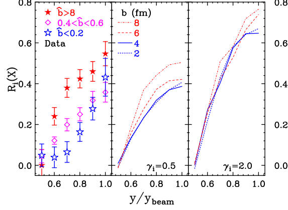
FIG. 8. (Color online) (Left panel) Experimental R_i as a function of rapidity for three centrality gates [16]. (Middle panel) The calculated results of R_i(X = \delta_{N,frag}) as a function of rapidity for b = 2, 4, 6, 8 fm for \gamma_i = 0.5 and (Right panel) \gamma_i = 2.0 .
