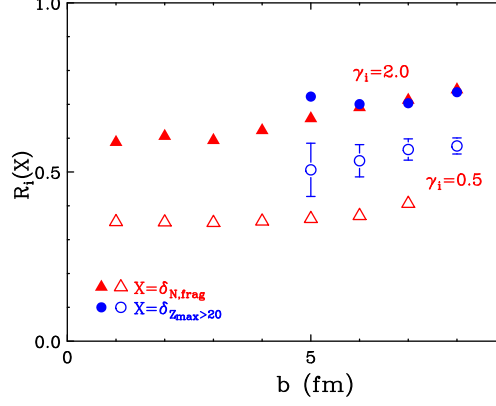
FIG. 7. (Color online) Isospin transport ratios as a function of impact parameter with two tracers for a soft symmetry case ( \gamma_i = 0.5 , open symbols) and a stiff symmetry case ( \gamma_i = 2.0 , closed symbols). Upright triangle symbols are for the tracer defined by the isospin asymmetry of all fragments and unbound nucleons with velocity cut ( v_z^{N,frag} > 0.5v_{beam}^{c.m.} ), X = \delta_{N,frag} . Circles are for the tracer defined by the heaviest fragment with Z_{max} > 20 in projectile region, X = \delta_{Z_{max} > 20} .
