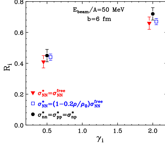
FIG. 9. (Color online) The effects of different in-medium NN cross sections on R_i(X = \delta_{N,frag}) . The inverted triangles are for the free space NN cross section \sigma_{nn/np}^* = \sigma_{nn/np}^{free} (case 1 in text). The open squares are for the isospin-dependent in-medium NN cross section with phenomenological formula \sigma_{nn/np}^* = (1 - 0.2\rho/\rho_0)\sigma_{nn/np}^{free} (case 2). The solid circles are for the isospin-independent in-medium NN cross section \sigma_{nn}^* = \sigma_{pp}^* = \sigma_{np}^* (case 3).
