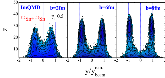
FIG. 4. (Color online) Multiplicity of fragments with charge Z as a function of their scaled rapidity y/y_{beam}^{c.m.} for ^{112}\text{Sn} + ^{112}\text{Sn} at E/A=50\text{MeV} for b=2 fm (left panel), 6 fm (middle panel), and 8 fm (right panel).
