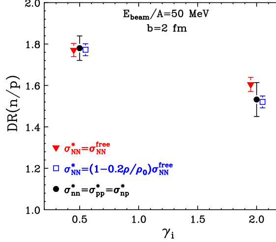
FIG. 6. (Color online) Effects of different in-medium NN cross sections on the DR(n/p) from transverse emitted high energy nucleons ( E_{c.m.} > 40 MeV). The inverted triangles are for the free space NN cross section (case 1 in text). The open squares are for the isospin-dependent in-medium NN cross section with a phenomenological formula (case 2). The solid circles are for the isospin-independent in-medium NN cross section (case 3).
