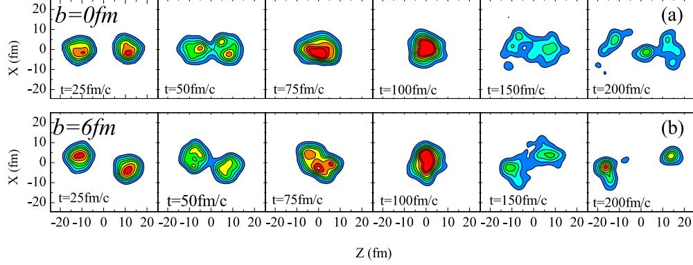
FIG. 2. (Color online) Time evolution of the nucleon density in the reaction plane for ^{124}\text{Sn} + ^{124}\text{Sn} collisions at E/A=50\text{MeV} at b=0 (top panels) and 6 (bottom panels) fm.
