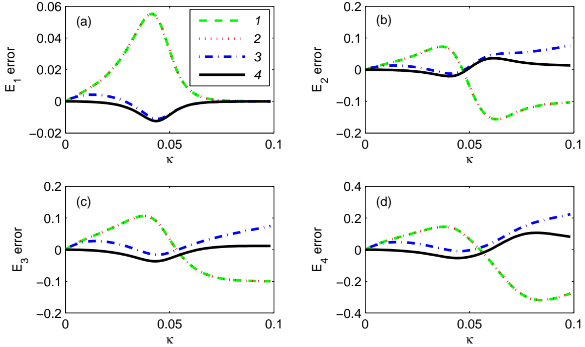
FIG. 2: (Color online) The errors of the first four excitation energies E - E_{\text{exact}} as a function of \kappa in a set of calculations. Panels (a), (b), (c), and (d) are for the first, second, third, and fourth excitation energy, respectively. Four lines on each panel are obtained by diagonalizing different collective Hamiltonian in different phonon space. 1 (green dashed line): H = \frac{\omega^2}{2}\alpha^2 + \frac{1}{2}\pi^2 + \frac{\Lambda^{(40)}}{4!}\alpha^4 in \{|0 \leq n < +\infty\} . 2 (red dotted line): H = \frac{\omega^2}{2}\alpha^2 + \frac{1}{2}\pi^2 + \frac{\Lambda^{(40)}}{4!}\alpha^4 in \{|0 \leq n \leq \Omega\} . 3 (blue dashed-dotted line): H = \frac{\omega^2}{2}\alpha^2 + \frac{1}{2}\pi^2 + \frac{\Lambda^{(40)}}{4!}\alpha^4 in \{|0 \leq n \leq \Omega\} , but with \omega^2 = 1 - \kappa^2\Omega(\Omega + 2) replacing that in Eq. (29). 4 (black solid line): H = \frac{\omega^2}{2}\alpha^2 + \frac{1}{2}\pi^2 + \frac{\Lambda^{(40)}}{4!}\alpha^4 + \frac{\Lambda^{(04)}}{4!}\pi^4 in \{|0 \leq n \leq \Omega\} , also with \omega^2 = 1 - \kappa^2\Omega(\Omega + 2) . 1 and 2 closely overlap and are indistinguishable on the figure.
