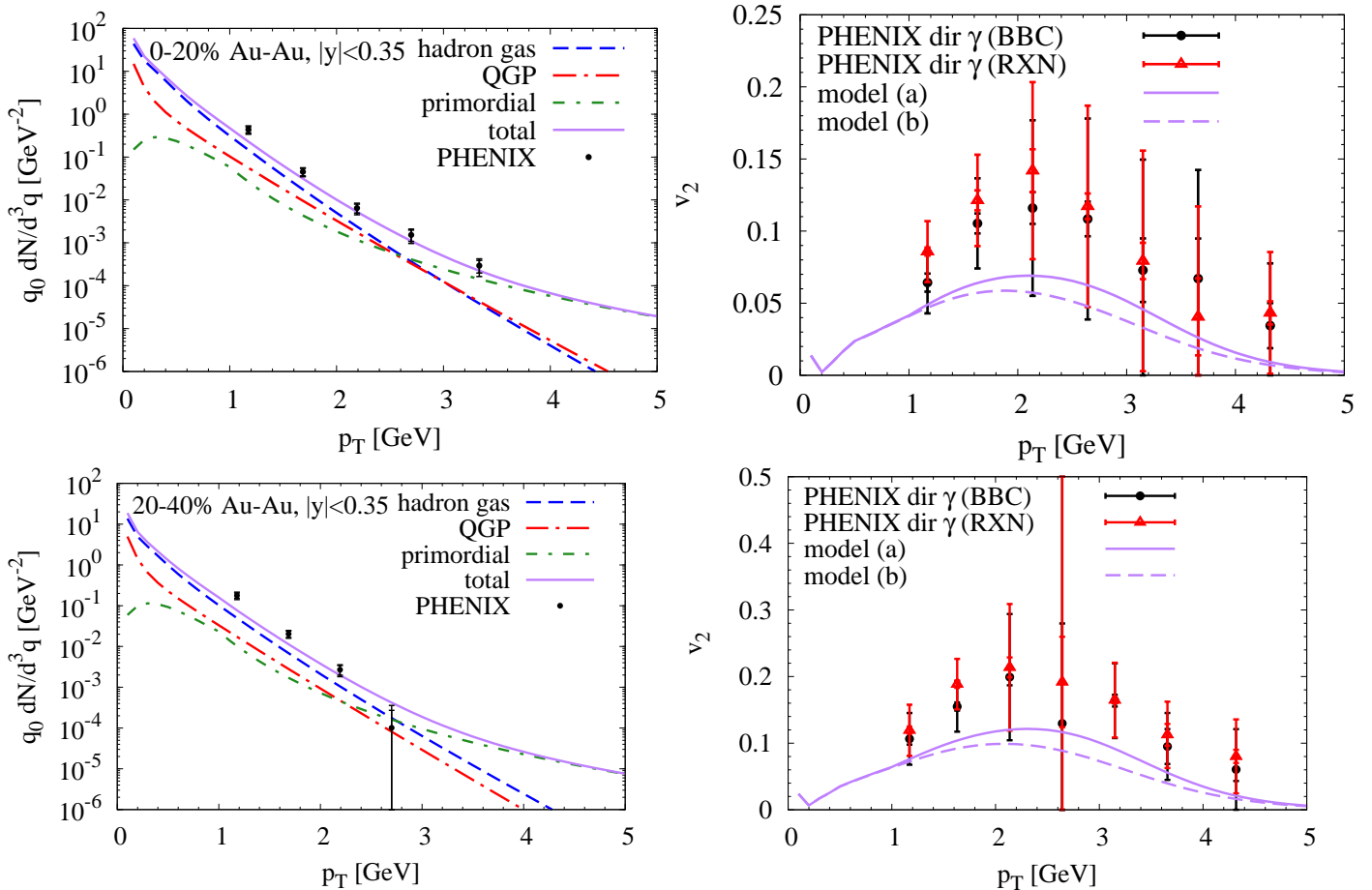
FIG. 5: (Color online) Comparison of our calculated direct-photon spectra (left panels) and their elliptic-flow coefficient (right panels) from an elliptically expanding fireball model with QGP and hadronic radiation, supplemented with primordial emission, to PHENIX data [7, 11] in 0-20% (upper panels) and 20-40% (lower panels) central Au-Au( \sqrt{s} = 200 AGeV) collisions. Models (a) and (b) in the right panels refer to the use of the pQCD parameterization and the PHENIX fit for primordial production, respectively (in the left panels, only model (a) is displayed).
