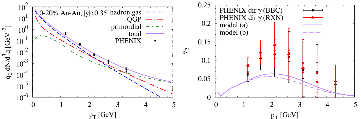
FIG. 6: (Color online) Same as Fig. 5 for 0-20% Au-Au collisions, but with a QGP contribution evaluated for a reduced thermalization time of \tau_0 \simeq 0.17 \text{ fm}/c translating into an average initial temperature of T_0 \simeq 445 \text{ MeV} .
