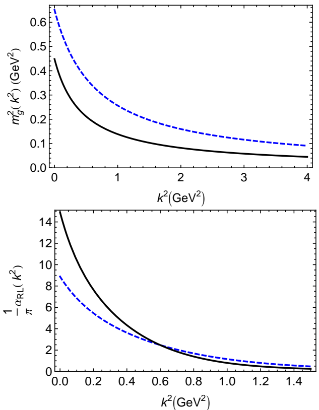
FIG. 1. Upper panel – Rainbow-ladder gluon running-mass inferred from Eq. (8) via Eq. (10). Lower panel – rainbow-ladder effective coupling inferred from Eq. (8). In both panels: \omega = 0.5 GeV (solid curve); \omega = 0.6 GeV (dashed curve).
