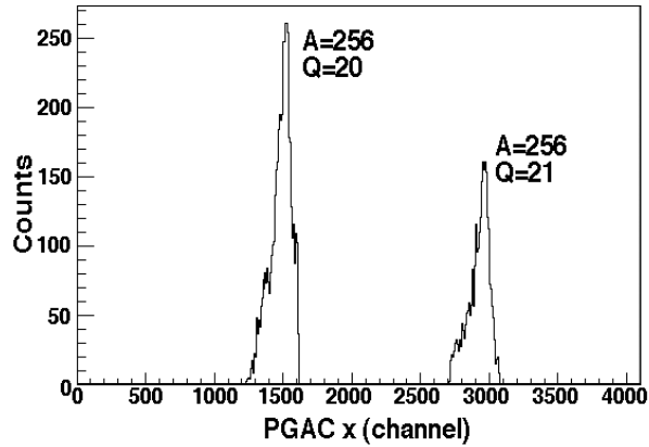
FIG. 2: A/Q spectrum for A=256 recoils, measured at the focal plane of the FMA, with additional software gates placed on the time-of-flight between PGAC and DSSD and the recoil energy.
