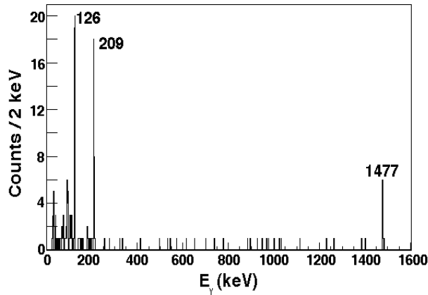
FIG. 4: \gamma spectrum in coincidence with the isomeric electrons from ^{216}\text{Th} shown in Fig. 3.
