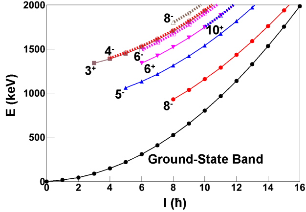
FIG. 1: (Color online) Estimated ground-state and 2-qp rotational bands in ^{256}\text{Rf} . The energies are given by E(I) = A[I(I+1)-K(K+1)] + E_0 . Bandhead energies E_0 , calculated as described in the text, are given in Table I. Rotational parameters A are taken as 7.3 and 6 keV for the ground-state and 2-qp bands, respectively. Solid and dotted lines denote proton and neutron configurations, K^\pi values are given for 2-qp bands. The origin and population of a high-K isomer depend on the relative energies of the high-K rotational bands.
