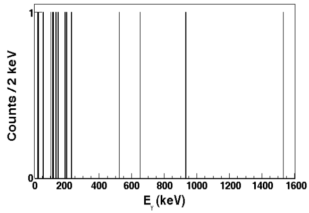
FIG. 7: \gamma spectrum in coincidence with the isomeric electrons shown in Fig. 6. No candidates for isomeric transitions are detected.
