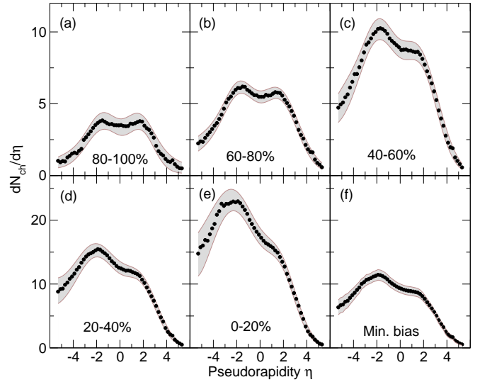
FIG. 28: The charged particle multiplicity, dN_{ch}/d\eta , is shown for five centrality bins for d + Au collisions (panels a-e). The grey-shaded area represents the 1\sigma standard deviation. The minimum-bias distribution is shown in panel f. The pseudorapidity, \eta , is given relative to the deuteron beam, which travels in the positive z direction.
