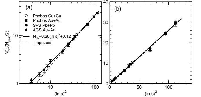
FIG. 26: Doubly logarithmic (panel a) and linear (panel b) plots of N_{ch}^p/\langle N_{part}/2 \rangle vs. (\ln s)^2 . The PHOBOS results are for 0-3% central collisions. The trend is extended to lower energies with data from the SPS [22] and AGS [49]. The dashed and solid curves were calculated using Eqs. 16 and 17, respectively.
