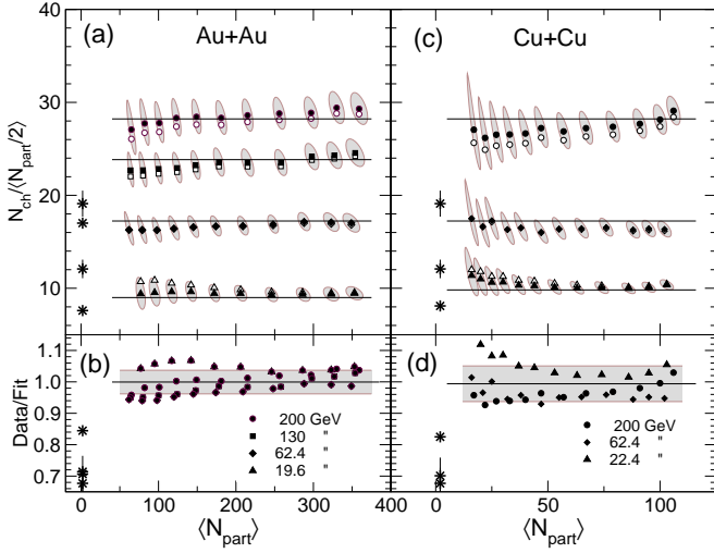
FIG. 27: Two estimates of the total charged particle multiplicity per participant pair, 2N_{ch}|\eta|<5.4/\langle N_{part} \rangle (open points) and 2N_{ch}^p/\langle N_{part} \rangle (solid points), are shown as a function of centrality for each energy for Au + Au (panel a) and Cu + Cu (panel c) collisions. Horizontal lines represent centrality independent levels predicted by Eq. 17. The lower panels show the ratio of data to the Eq. 17 prediction. The solid line is the average of all data points and the grey-shaded area the 1\sigma standard deviation. Corresponding data for p\bar{p}/pp collisions are shown as stars, see Figs. 24 and 25 for details.
