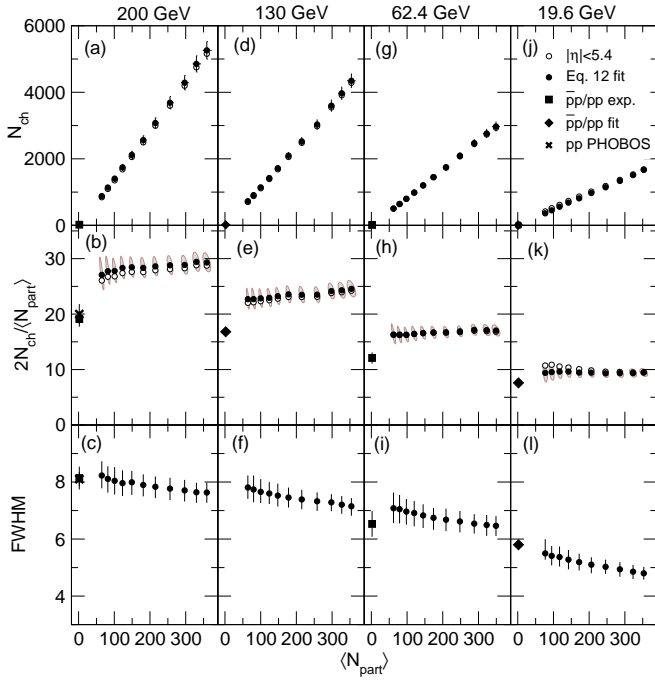
FIG. 24: The total charged particle multiplicity, N_{ch} , the total charged particle multiplicity per participant pair, 2N_{ch}/\langle N_{part} \rangle and the full width at half maximum, FWHM are shown as a function of centrality for each energy for Au + Au collisions. The first two quantities are shown for both the measured region N_{ch}|_{|\eta|<5.4} (open points) and based on extrapolations, N_{ch}^p (solid circles), see text for details. Corresponding data for inelastic \bar{p}p collisions [43] at 200 GeV and pp collisions [42] are shown as solid squares, whereas the crosses are from the present work and solid diamonds represent an overall fit N_{ch} = -0.42 + 4.69s^{0.155} for inelastic collisions [52]. The FWHM for 200 GeV \bar{p}p and 62.4 GeV pp collisions (solid squares) were obtained from Refs. [43] and Ref. [42], respectively, whereas the value (solid diamond) for 19.6 GeV represents an extrapolation based on data in the latter work. No FWHM data are available for 130 GeV pp collisions. Error bars and ellipses represent systematic 90% C.L. errors.
