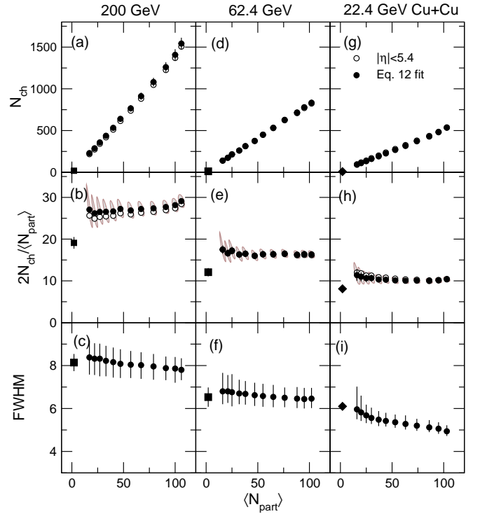
FIG. 25: Same as Fig. 24 but for Cu+Cu collisions. The data for 22.4 GeV pp collisions (solid diamonds) were obtained as for the 19.6 GeV data shown in Fig. 24.
