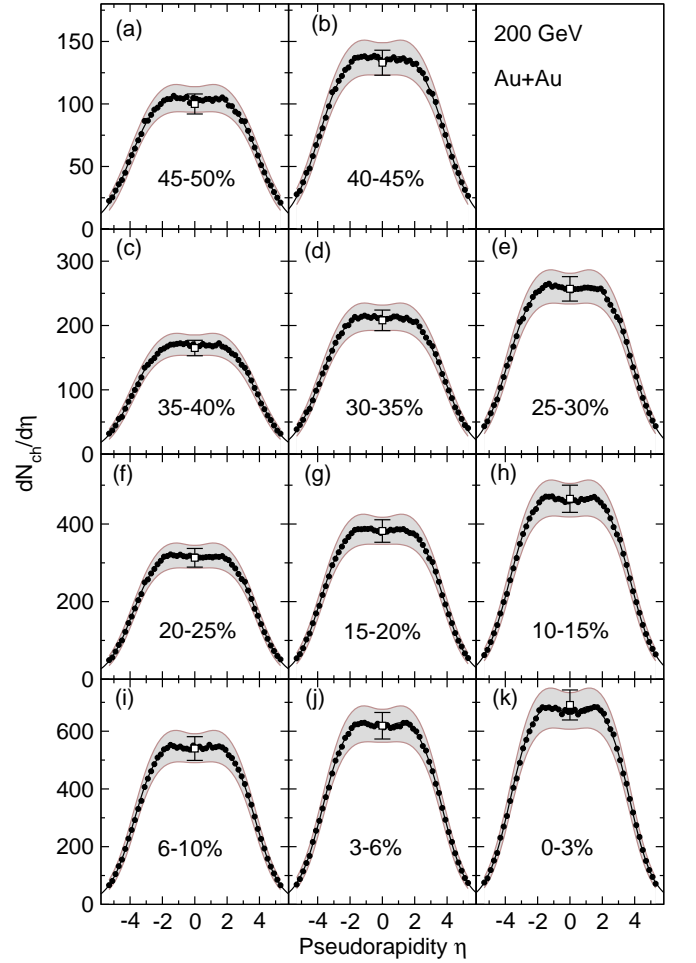
FIG. 18: Same as Fig. 17 but for Au+Au collisions at \sqrt{s_{NN}} = 200 GeV. The solid curves represent best fits to the data over the full \eta range using Eq. 14 and the shaded regions represent 90% C.L. systematic errors. The open points were obtained by the tracklet analysis in the range |\eta| < 1 .
