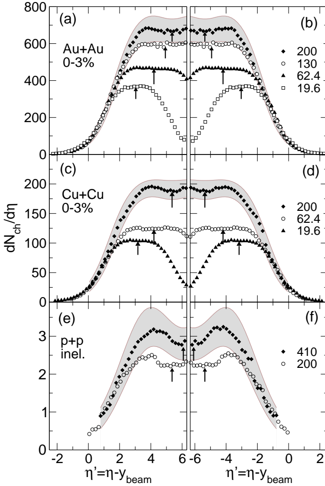
FIG. 30: Illustration of the extended longitudinal scaling ( a.k.a. limiting fragmentation scaling) for Au + Au (panels a, b), Cu + Cu (panels c, d), and p + p collisions (panels e, f). The systematic errors (90% C.L.) are shown as shaded areas for the highest energy only for each system. The arrows indicate the location of mid-rapidity ( \eta=0 ).
