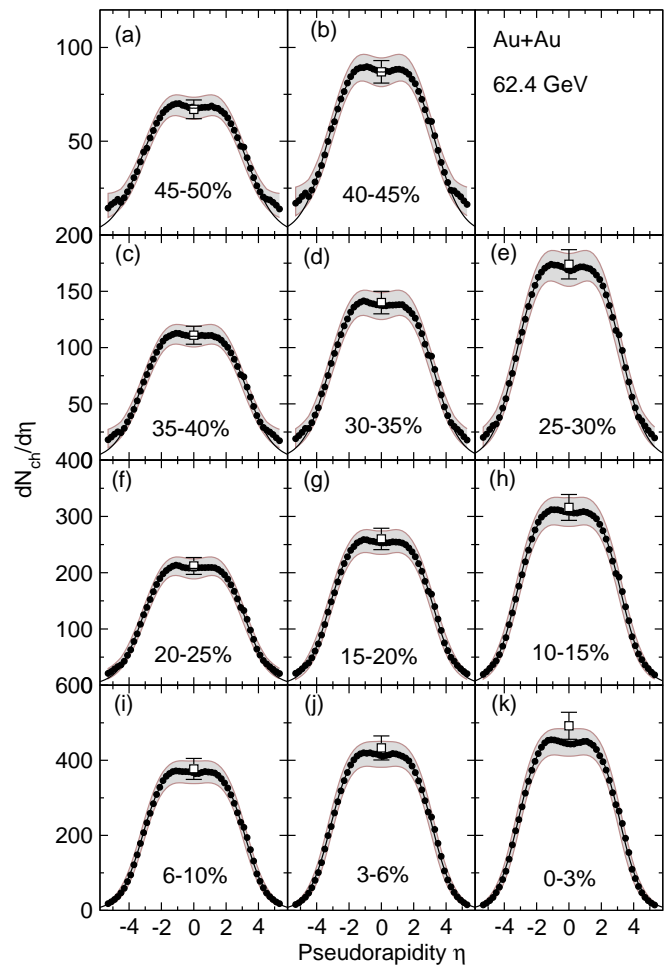
FIG. 16: dN_{ch}/d\eta vs \eta (solid points) for eleven centrality bins representing 50% of the total cross section for Au+Au collisions at \sqrt{s_{NN}}=62.4 GeV. The solid curve is a fit to the data within the -4.2 < \eta < 4.2 region using Eq. 14 (see text for details). The shaded band represent 90% C.L. systematic errors. The open points were obtained by the tracklet analysis in the range |\eta| < 1 .
