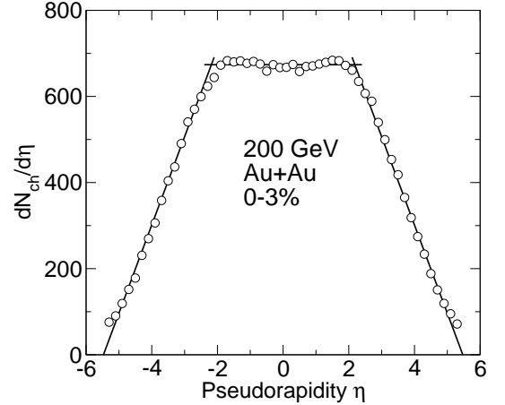
FIG. 23: Illustration of the trapezoidal approximation for 200 GeV Au+Au collisions at 0-3% centrality. Open circles represent the data (errors are not shown for clarity) and the black lines represent the piecewise linear trapezoidal approximation to the data as described in the text.
