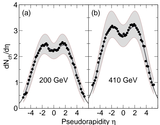
FIG. 29: The charged particle multiplicity, dN_{ch}/d\eta , is shown for 200 GeV (panel a) and 410 GeV (panel b) for pp inelastic collisions. The grey-shaded area represents the 90% confidence limit systematic error. The solid curves are symmetric double-Gaussian fits to the data used to derive the total multiplicities listed in Table IV.
