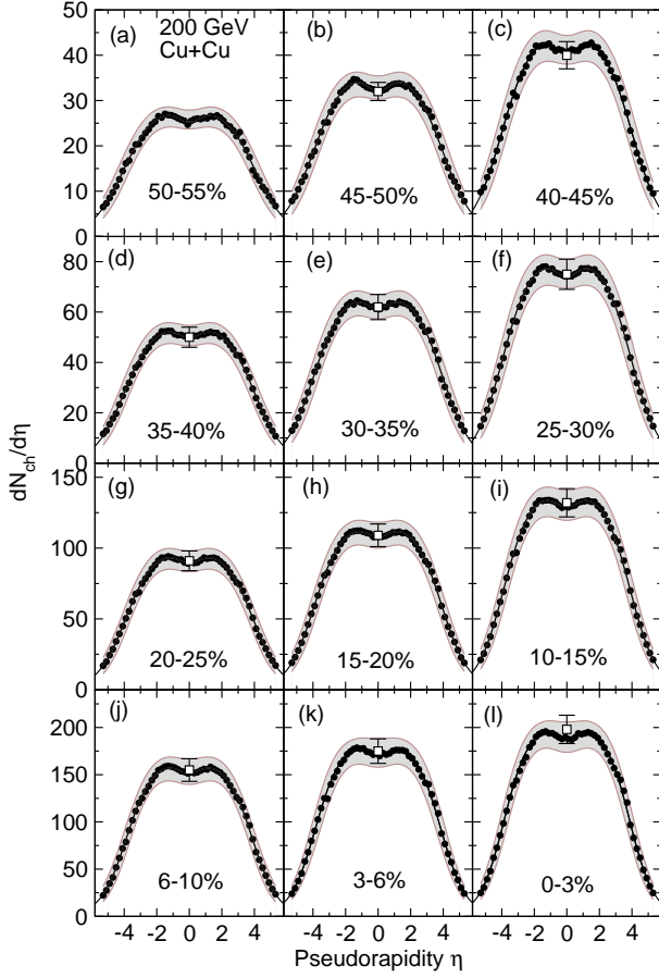
FIG. 21: Same as Fig. 20 but for \sqrt{s_{NN}} = 200 GeV. The solid curve is a fit to the data over the full \eta region using Eq. 14. The open points were obtained by the tracklet analysis for events in the range |\eta| < 1 .
