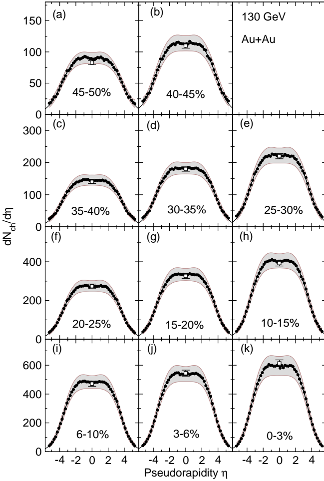
FIG. 17: Same as Fig. 16 but for Au+Au collisions at \sqrt{s_{NN}} = 130 GeV. The solid curves represent best fits to the data over the region -4.9 < \eta < 4.9 using Eq. 14 (see text) and the shaded regions represent the systematic error band at 90% confidence limit. The open points were obtained by the tracklet analysis in the range |\eta| < 1 .
