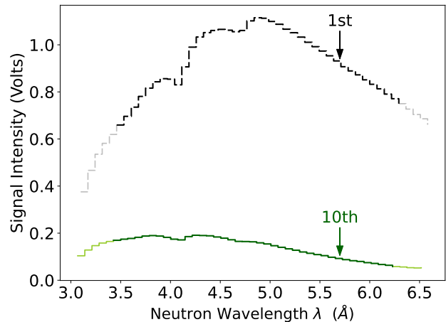
FIG. 1: The selected measured outputs of the central signal wires of the 1 st and the 10 th wire planes out of 16 planes. The plots indicate how the incoming beam intensity and shape change as it passes through the ^3\text{He} gas in the chamber. The signals were measured as a function of TOF but are plotted as a function of the neutron wavelength. Due to 17 cm difference in distance between the two wire planes from the moderator, the neutron wavelengths on the 10 th are little shorter than on the 1 st wire, consequently, there is a half time bin shift between the wavelength plots. The signals represent collected charges after the emitted proton and triton from the n\text{-}^3\text{He} capture deposit their kinetic energy to ^3\text{He} gas, see text for details. The integration ranges of the two signals are indicated with thicker lines. The two small dips at 4.1 Å and 4.7 Å are residuals from neutron transmission Bragg-edges on the aluminum beamline windows.
