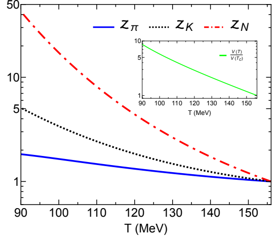
FIG. 4. Temperature dependence of pion (solid line), kaon (dashed line) and nucleon (dash-dotted line) fugacities as well as the volume ratio of hadronic matter (solid line in the inset).
