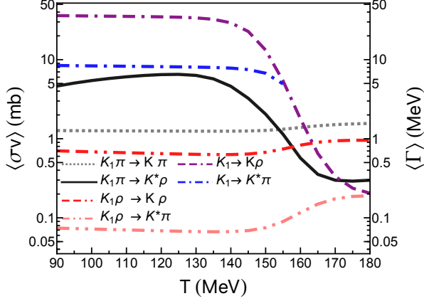
FIG. 3. Temperature dependence of thermal averaged cross sections \langle\sigma v\rangle for the reactions K_1\pi \rightarrow K\pi (dotted line), K_1\pi \rightarrow K^*\rho (solid line), K_1\rho \rightarrow K\rho (dash-dash-dot-dotted line), and K_1\rho \rightarrow K^*\pi (dash-dot-dotted line), and thermal averaged decay widths \langle\Gamma\rangle of K_1 \rightarrow K\rho (dash-dash-dotted line) and K_1 \rightarrow K^*\pi (dash-dotted line).
