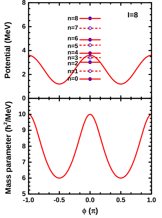
FIG. 2. Upper panel: classical potential energy V(\phi) as a function of \phi for spin I = 8 . The dots show the quantal energies E_v calculated by TRM, while the horizontal lines represent the energies obtained by the collective Hamiltonian H_{CH} , which incorporates a \phi -dependent mass parameters B(\phi) shown in the lower panel. Note that for the even phonon states, they are calculated from I = 8 states, while for the odd phonon states, they are calculated as the 72/90 of I = 9 energies.
