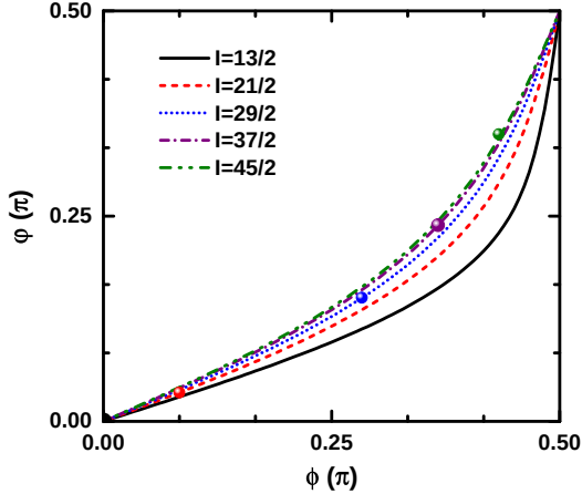
FIG. 9. The azimuthal angle \phi of \mathbf{j} as a function of azimuthal angle \phi of \mathbf{J} obtained by diagonalization of H_{ad} for the selected spins I = 13/2, 21/2, 29/2, 37/2 , and 45/2 . The dot on the curve label the potential minimum for each spin.
