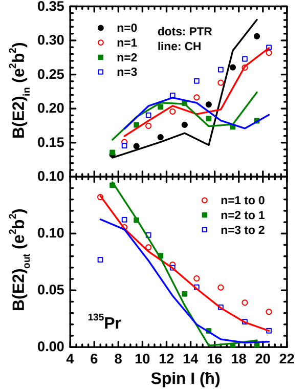
FIG. 6. Upper panel: calculated in-band B(E2)_{\text{in}}(I \rightarrow I-2) , of the bands in Fig. 5, where the same line and color conventions are used. Lower panel: calculated inter-band B(E2)_{\text{out}}(I \rightarrow I-1) transition probabilities between the bands shown in Fig. 5. In order to keep the legend compact, the connecting transitions are labelled by quanta numbers n , which are associated with the states in the TW regime. Beyond, n represents just a counting label for the states.
