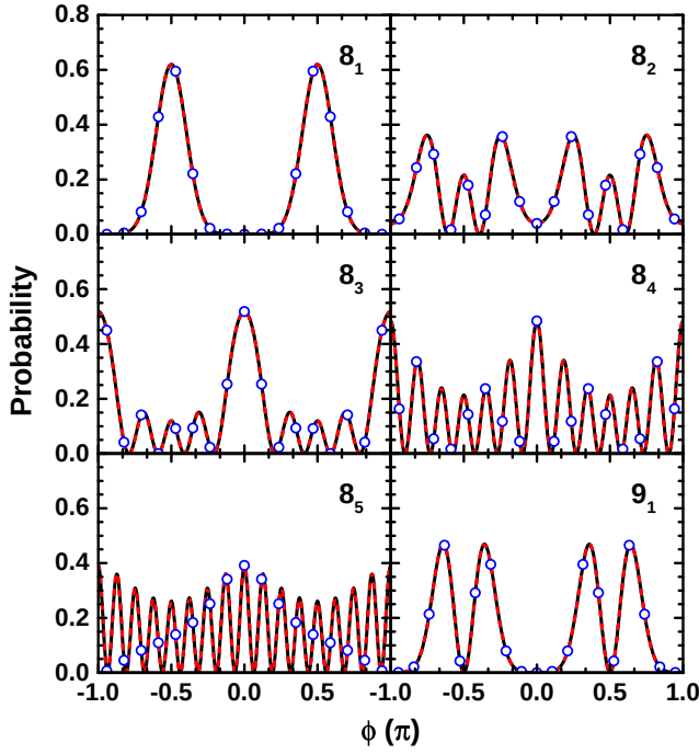
FIG. 3. Probability densities of the SSS for the triaxial rotor states 1-5 of I = 8 and the state 1 of I = 9 . The smooth solid and dashed lines continuous SSS P(\phi)_v obtained by the TRM and collective Hamiltonian, respectively. The dots represent the discrete SSS \frac{2\pi}{2I+1}P(\phi_n)_v .
