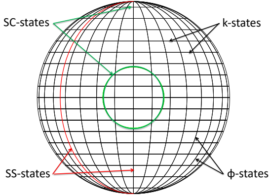
FIG. 1. Schematic illustration of the different states used as basis sets in the j -space. Each state is represented by a curve along which the endpoint of angular momentum vector is distributed with equal probability. The k -states are circles of constant latitude k . The \phi -states are semicircles of constant \phi . The figure displays the pertaining meridians. For the continuous set of SCS only the states |\theta = 0, \phi = 0\rangle and |\theta = \pi/2, \phi = 0\rangle are examples shown. For the continuous set of SSS only the states |\phi = 0\rangle and |\phi = -\pi/4\rangle are shown.
