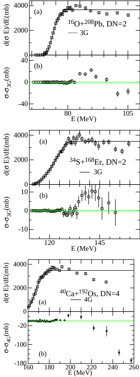
FIG. 3. d(\sigma E)/dE and \sigma - \sigma_{th} spectra for fusion systems ^{16}\text{O} + ^{208}\text{Pb} [22] in upper part, ^{34}\text{S} + ^{168}\text{Er} [26] in middle part, and ^{40}\text{Ca} + ^{192}\text{Os} [19] in lower part, respectively. DN is the step number used in the differentiation process.
