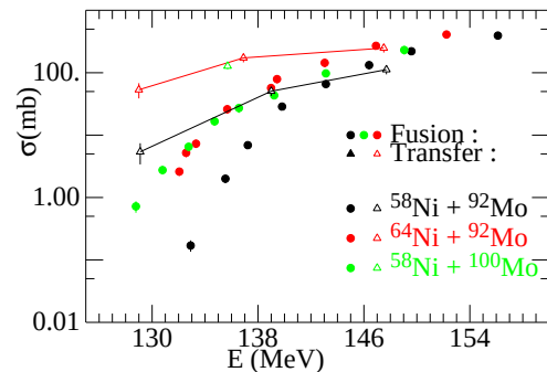
FIG. 5. Excitation functions of fusions and transfer reactions for some systems of Ni + Mo. Data come from Ref. [35–37], respectively.
