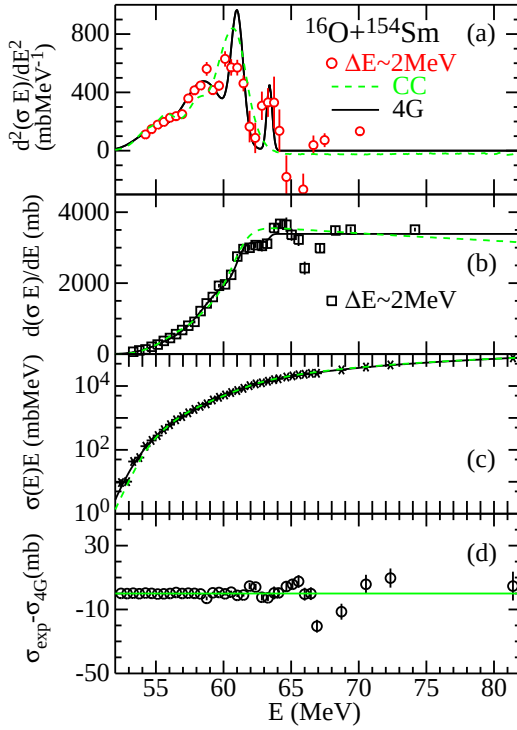
FIG. 2. Various representations vs E plots of fusion cross sections for system ^{16}\text{O} + ^{154}\text{Sm} [17]. Others are the same as in Fig. 1.
