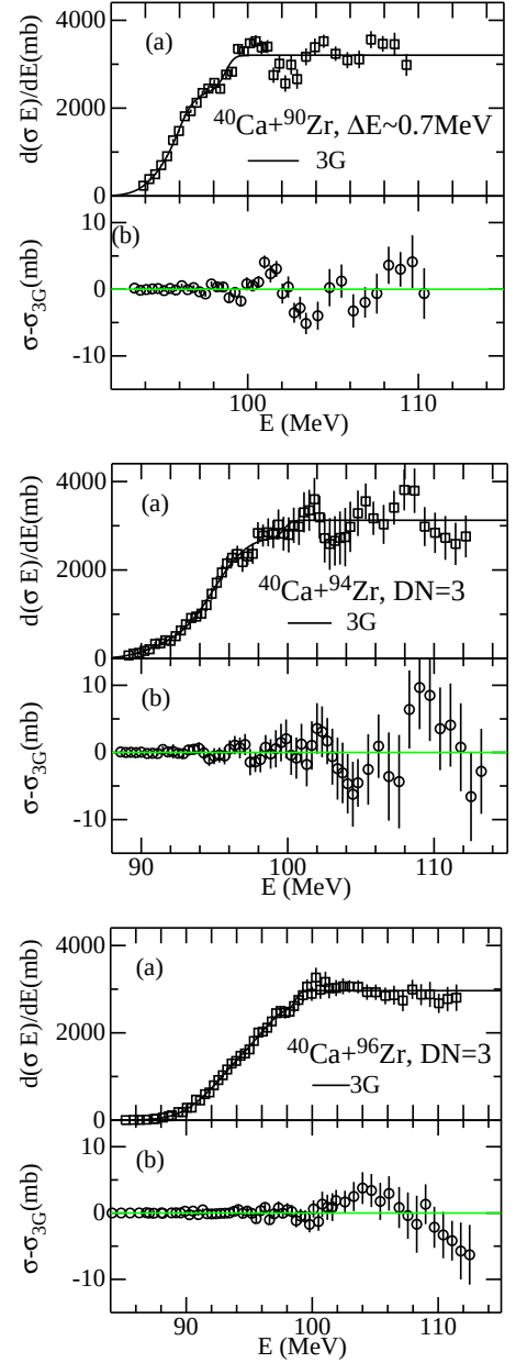
FIG. 4. d(\sigma E)/dE and \sigma - \sigma_{th} spectra for fusion systems ^{40}\text{Ca} + ^{90}\text{Zr} [16] in upper part, ^{40}\text{Ca} + ^{94}\text{Zr} [20] in middle part, and ^{40}\text{Ca} + ^{96}\text{Zr} [21] in lower part, respectively. DN is the step number used in the differentiation process.
