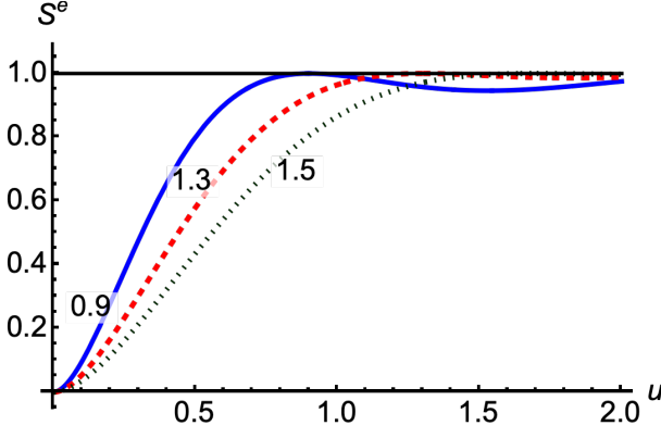
FIG. 2. S^e as a function of the dimensionless variable u for the three different values of v . The values of v are 0.9 (solid), 1.3 (dashed) and 1.5 (dotted). These values correspond to total cross sections of 22 mb, 40 mb and 56 mb for u = v .
