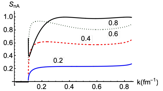
FIG. 1. S_{nA} as a function of k for the four different values of V_{12}/V_1 shown in the figure.
