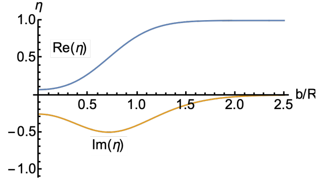
FIG. 3. Real and imaginary parts of \eta(b) .
