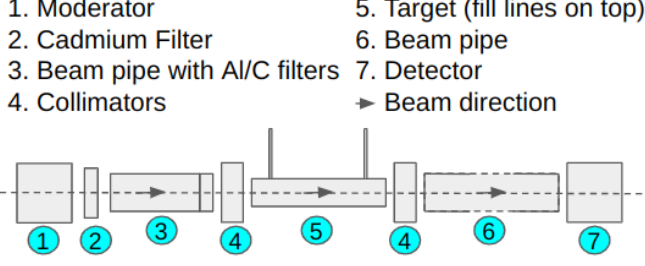
FIG. 1. Configuration of the beam line elements. 1) Mark III LANSCE target and moderator. 2) cadmium filter for suppression of thermal neutrons. 3) \approx 30 m beam pipe where carbon and aluminum filters were mounted. 4) brass collimators. 5) ARTIE target. 6) \approx 30 m beam pipe. 7) 6-Li glass detector at 64 m followed by beam dump.
