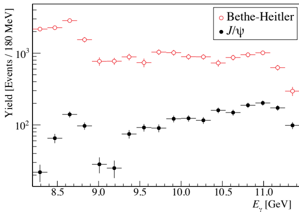
FIG. 7. Comparison of BH and J/\psi yields as function of beam energy.
