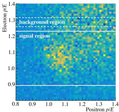
FIG. 3. Electron vs. positron p/E distribution in the BH invariant mass region of 1.2 – 2.5 GeV. The white horizontal lines indicate the background and signal regions used when projecting onto the positron axis. See text for explanations.
