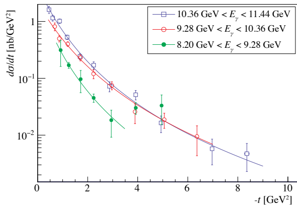
FIG. 15. The differential cross sections for the three energy regions fitted with [d\sigma/dt(0)]/(1-t/m_s^2)^4 , where the cross section at t=0 , d\sigma/dt(0) , and the mass scale, m_s , are free parameters.
