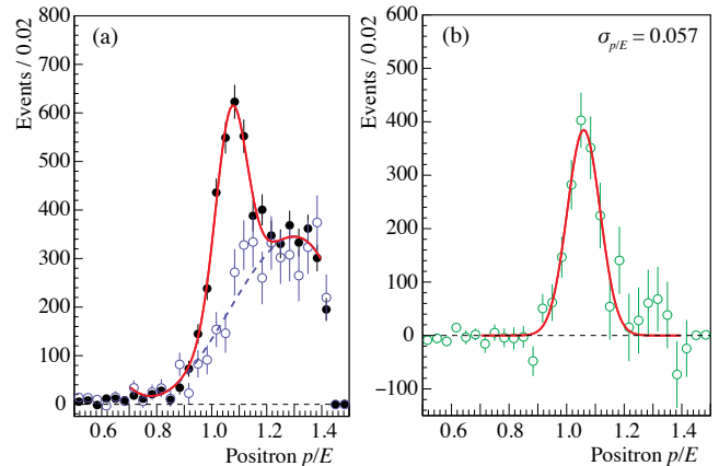
FIG. 4. (a) The p/E distributions in the signal (solid black) and background (open blue) region for the BH invariant mass region of 1.2 – 2.5 GeV. (b) The difference between the signal and background distributions from (a). See text for explanation of the fits.
