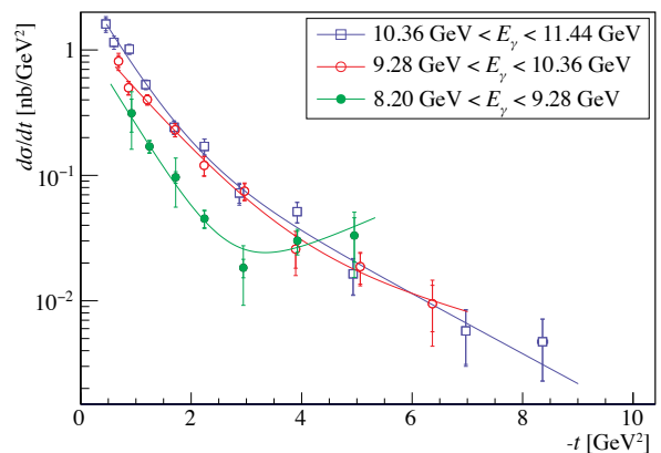
FIG. 13. The measured differential cross sections with both statistical (inner bars) and total (outer bars) uncertainties shown for the three energy regions, from Eq.(5). The points are fitted with a sum of two exponential functions. The second exponential contribution is most significant in the lowest energy bin, where the slope changes sign.
