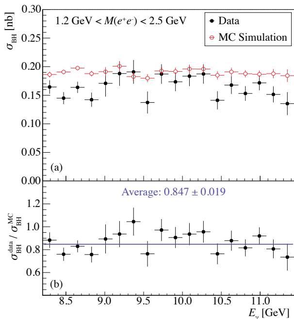
FIG. 5. BH cross section vs. beam photon energy for 1.2 < M(e^+e^-) < 2.5 GeV. (a) BH cross section obtained from data and MC simulation. (b) Ratio of data and MC cross sections from (a) fitted with a constant.
