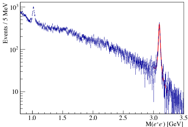
FIG. 1. The e^+e^- invariant mass spectrum for the GlueX Phase-I data set after applying the selections described in Section III. The J/\psi peak is fitted with a linear function and two Gaussians with common mean, which yields a total of 2270 \pm 58 J/\psi 's.
