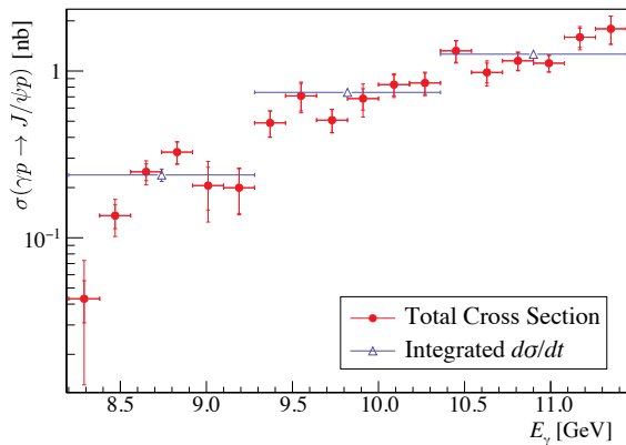
FIG. 11. The filled red points show the measured total cross sections obtained from Eq.(3) in fine photon energy bins. The inner bars represent the statistical errors and outer bars are the total errors, with the statistical and systematic errors added in quadrature. The open blue triangles represent the total cross sections calculated by integrating the functions fitted to the measured differential cross sections for the three beam energy regions, with only the statistical uncertainties shown.
