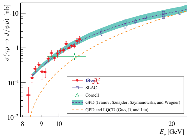
FIG. 17. Comparison of the J/\psi total cross sections from this work (GlueX) to the SLAC [45] and Cornell [47] data and two QCD theoretical calculations in the two-gluon exchange factorization model (in LO) from Ref. [48] and from Ref. [10]. The latter calculation uses gravitational form factors from lattice calculations [44]. The SLAC total cross sections are estimated from their d\sigma/dt|_{t=t_{min}} measurements [45] assuming a dipole t -dependence from the fit of our differential cross section at the highest energy, Fig. 15. The error bars shown for the GlueX data are the statistical and systematic errors summed in quadrature.
