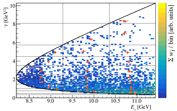
FIG. 12. The distribution of the flux-weighted data in the E_\gamma-t plane and the mean values of the reported cross sections (solid dots) within the corresponding bins. A mass selection of 3.05 < M(e^+e^-) < 3.15 GeV is used for the events in this plot.
