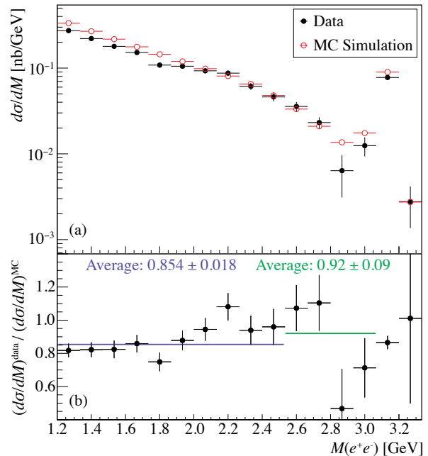
FIG. 6. The sum of BH and J/\psi cross sections as function of e^+e^- invariant mass. (a) Cross section obtained from data and MC simulation. (b) Ratio of data and MC cross sections from (a) fitted with constants in two regions: the region used for normalization of the J/\psi cross section, and the vicinity of the J/\psi peak.
