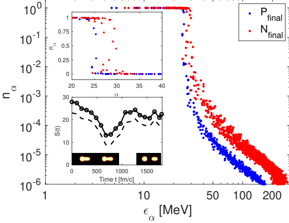
FIG. 5. The final proton and neutron canonical occupation probabilities n_\alpha = n(k) extracted from the TDDFT extended to superfluid systems treatment of induced fission reaction ^{235}\text{U}(n,f) as a function of \epsilon_\alpha = \epsilon(k) . The upper inset shows a small energy interval near the Fermi level. Above \epsilon_\alpha \approx 50 MeV one can see a clear power law behavior compatible with theory prediction n(k) \propto 1/[\epsilon(k)]^2 . The initial state was the compound nucleus close to the top of the outer fission barrier at t = 0 fm/c and in the final state the fission fragments are spatially separated by \approx 30 fm at t = 1,700 fm/c [4]. The non-equilibrium time-evolution of the orbital entanglement entropy S(t) is shown in the lower inset, with solid and dashed lines corresponding to no nucleon number projections and with nucleon number projections respectively [4].
