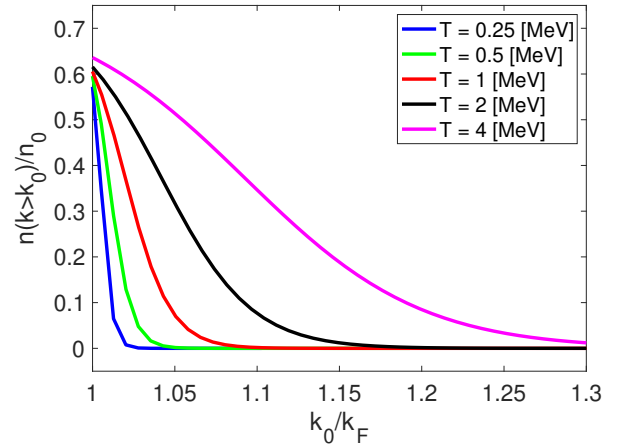
FIG. 4. The fraction of the particles n(k > k_0)/n_0 with momenta k \geq k_0 , where n(k) \propto 1/k^4 . The curves rank by temperature.
