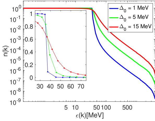
FIG. 1. Typical behavior of the s -wave canonical occupation probabilities in the case of pairing in a finite nuclear system. Three different amplitudes of the pairing field were considered here \Delta_0 = 1, 5 , and 15 MeV [4], the last one comparable to the strength of the pairing field in the unitary limit [56]. For \epsilon(k) > 75 MeV the momentum occupation probabilities have the behavior n(k) = C/k^4 \propto 1/[\epsilon(k)]^2 . The UV-cut-off is determined by \epsilon(k) of the highest canonical state with a wave function located inside the system. The states with \epsilon(k) beyond the UV-cut-off are not expected to be physically relevant [4], as their corresponding canonical occupation probabilities vanish in the continuum limit. In the inset, the occupation probabilities n(k) , shown in a linear scale, have an expected Bardeen-Cooper-Schrieffer [76].
