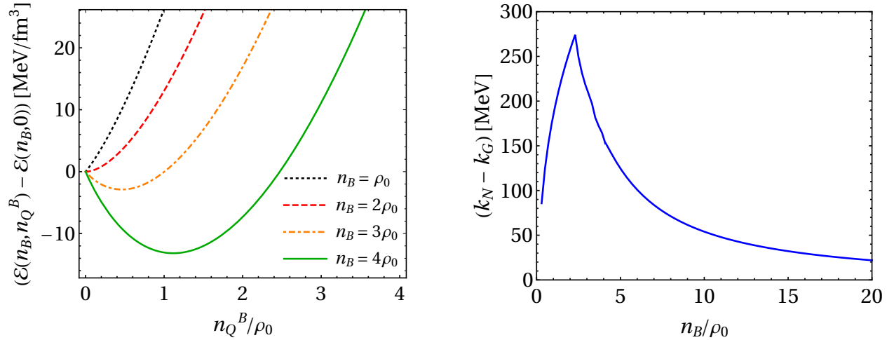
FIG. 2: Left: Energy density as a function of quark density n_Q^B , for an interacting quark model and different values of total baryon density n_B , including only vector interactions in the nucleon sector. Right: Shell thickness, defined as the difference between the nucleon and ghost Fermi momenta k_N - k_G .
