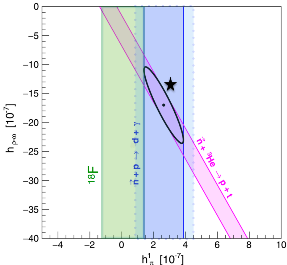
FIG. 1. Constraints on the parity-violating coupling constants h_{\rho-\omega} and h_{\pi}^1 , after Ref. [21]. The couplings are not direct physical observables and thus can be sensitive to the energy scale of the system under consideration, see the text for further discussion. Combining statistical and systematic errors in quadrature and working at 68% CL, we show the value h_{\pi}^1 = (2.6 \pm 1.2) \times 10^{-7} from the measured parity-violating asymmetry in \vec{n} + p \rightarrow d + \gamma [20] as the vertical band bounded by a solid line, and its determination h_{\pi}^1 = (2.7 \pm 1.8) \times 10^{-7} in chiral perturbation theory as the vertical band bounded by a dotted line [6, 13], and the diagonal constraint from the measured parity-violating asymmetry in \vec{n} + {}^3\text{He} \rightarrow p + t [21], with the combined fit of the two experiments yielding the ellipse shown. The analysis of {}^{18}\text{F} radiative decay from its 1.081 MeV excited state yields the bound |h_{\pi}^1| < 1.3 \times 10^{-7} [3], shown as the leftmost vertical band. Our ab initio result at a scale of 2 GeV is represented by the star with the associated error from its inputs roughly by its size. The tension with the {}^{18}\text{F} result at a nominal scale of less than 100 MeV, may also be reflective of an extraction in a different physical setting.
