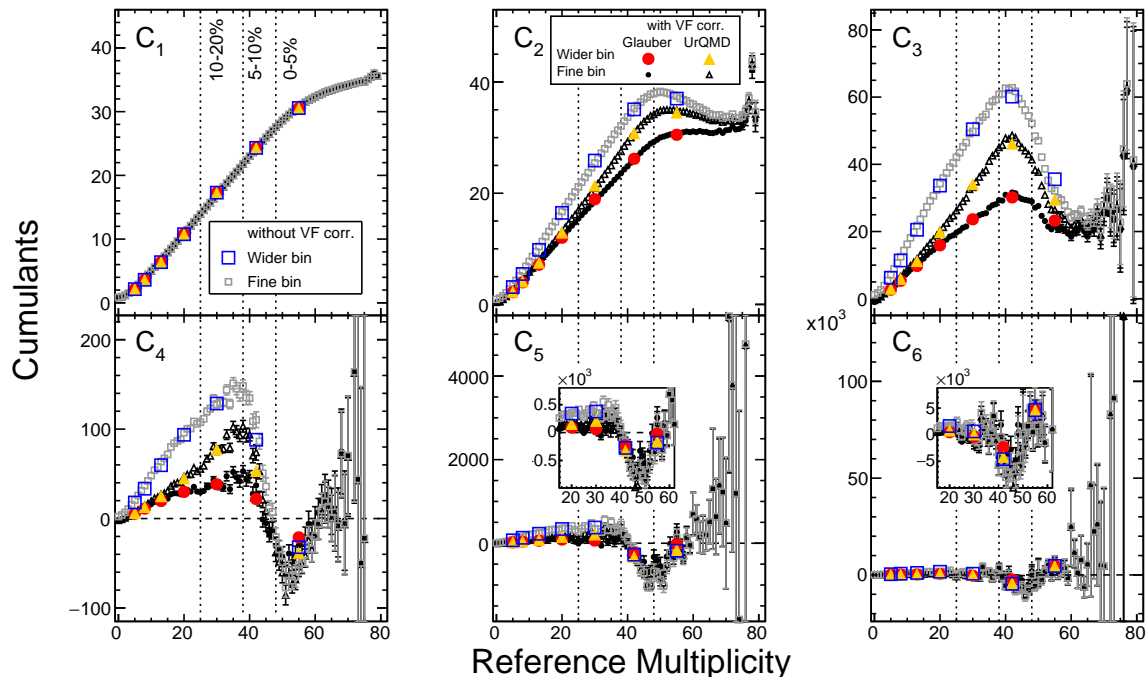
FIG. 11: Proton cumulants up to 6 th -order in \sqrt{s_{\text{NN}}} = 3 GeV Au+Au collisions. Data without volume fluctuation correction is shown as grey open squares while data with volume fluctuation correction using N_{\text{part}} distributions from Glauber and UrQMD models are shown as black circles and black open triangles, respectively. The corresponding centrality binned cumulants are shown in blue squares, red circles, and orange triangles, respectively. Similar to Fig. 6, the vertical dashed lines indicate the centrality classes.
