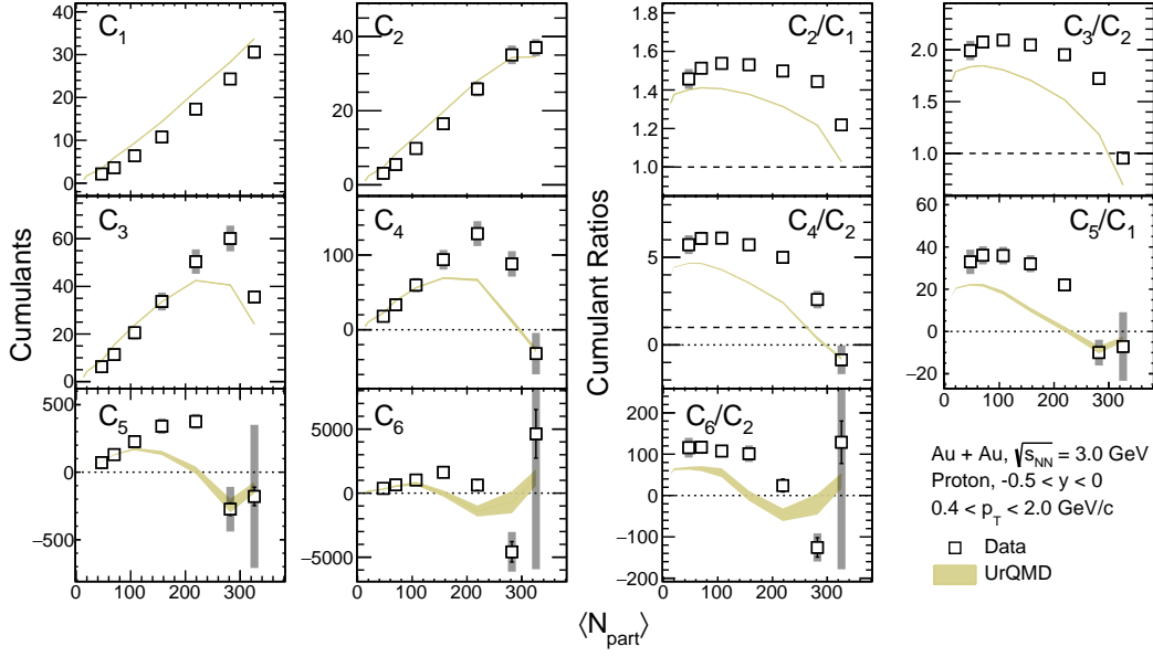
FIG. 16: Cumulants and cumulant ratios of proton multiplicity distributions for Au+Au collisions at \sqrt{s_{\text{NN}}} = 3 GeV. The transverse momentum window is p_T from 0.4 < p_T < 2.0 GeV/c and the rapidity window is -0.5 < y < 0 . Statistical and systematic uncertainties are represented by black and gray bars, respectively. UrQMD predictions are depicted by gold bands.
