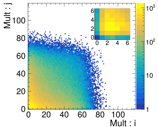
FIG. 5: Correlation between reference multiplicity i and j from single-collision events. The small panel at the top right corner is an expanded plot with i < 7 and j < 7 .
