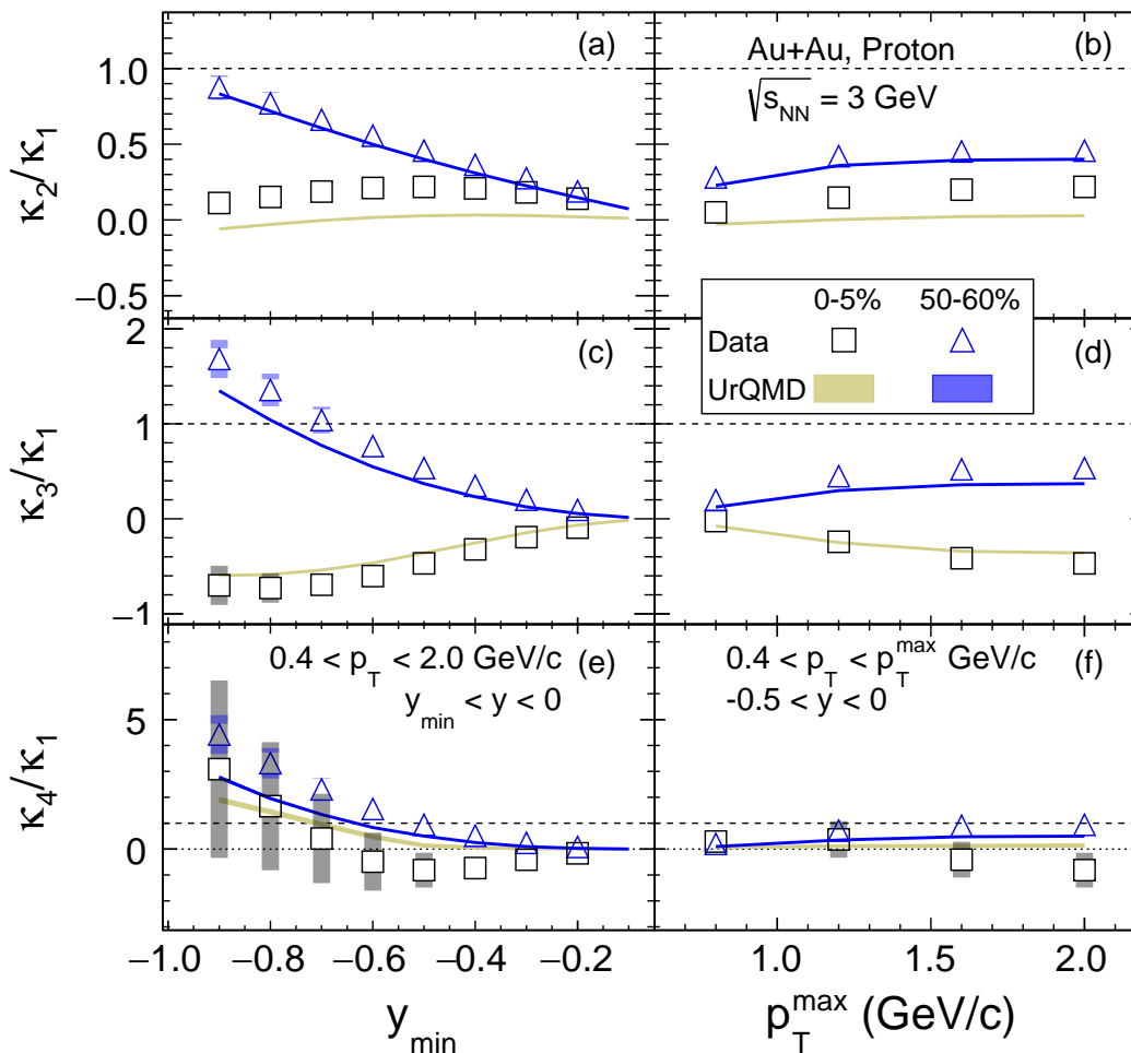
FIG. 19: As Fig. 18 but for transverse-momentum and rapidity dependence of correlation function ratios of proton multiplicity distributions for Au+Au collisions at \sqrt{s_{\text{NN}}} = 3 GeV.
