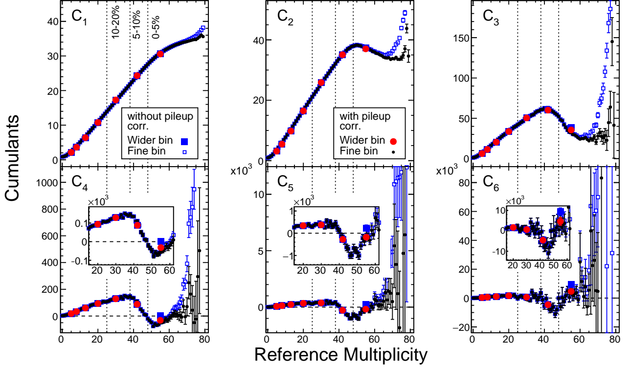
FIG. 6: Proton cumulants as a function of reference multiplicity from \sqrt{s_{\text{NN}}} = 3 GeV Au+Au collisions. Pileup corrected and uncorrected cumulants as a function of reference multiplicity are represented by black circles and blue open squares, respectively. Red circles and blue-filled squares represent the results of centrality binned data.
