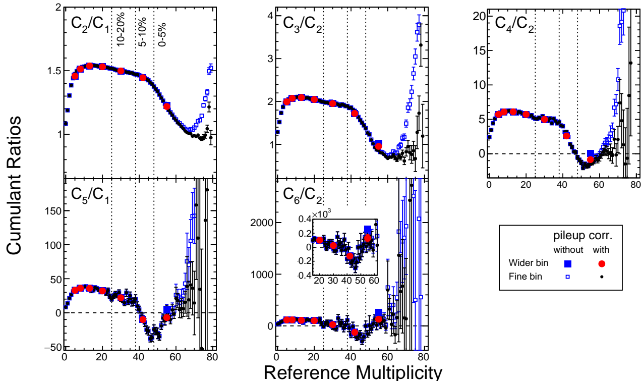
FIG. 7: Ratios of proton cumulants as a function of reference multiplicity from \sqrt{s_{\text{NN}}} = 3 GeV Au+Au collisions. Pileup corrected and uncorrected cumulants are represented by black circles and blue open squares, respectively. Red circles and blue-filled squares represent the results of centrality binned data.
