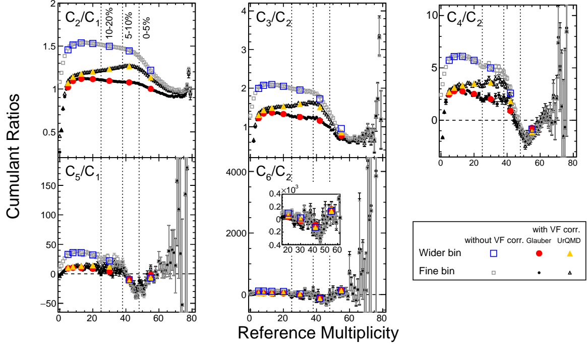
FIG. 12: Proton cumulant ratios up to 6 th -order in \sqrt{s_{NN}} = 3 GeV Au+Au collisions. Data without volume fluctuation correction are shown as grey open squares while data with volume fluctuation correction using N_{part} distributions from Glauber and UrQMD models are shown as black circles and black open triangles, respectively. The corresponding centrality binned cumulants are shown in blue squares, red circles, and orange triangles, respectively. Similar to Fig. 6, the vertical dashed lines indicate the centrality classes.
