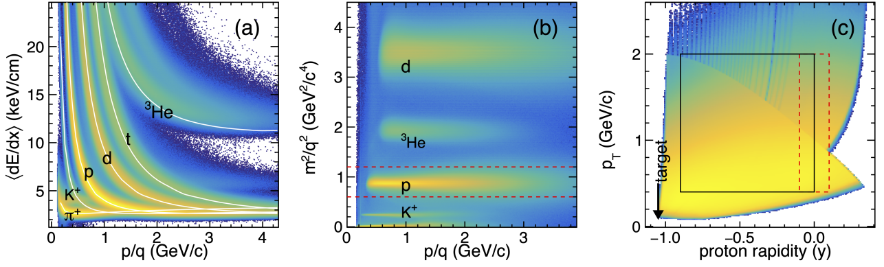
FIG. 2: (a): \langle dE/dx \rangle vs. particle rigidity measured in the TPC; pion, kaon, proton and deuteron bands are labeled. The proton is plotted in red from the Bichsel formula. (b): Mass-squared vs. the particle rigidity measured in the TPC and TOF. Kaon, proton, deuteron, and Helium-3 peaks are labeled. The red dashed lines indicate selection cuts by mass-squared. (c): Analysis acceptance in transverse momentum vs. proton rapidity ( y ) in the center-of-mass frame Au+Au collisions at \sqrt{s_{NN}} = 3 GeV. Black box indicates acceptance for rapidity -0.9 < y < 0 and momentum 0.4 < p_T < 2.0 GeV/c. The Red dashed box indicates a narrower rapidity window |y| < 0.1 , the largest possible symmetric rapidity window from this data set.
