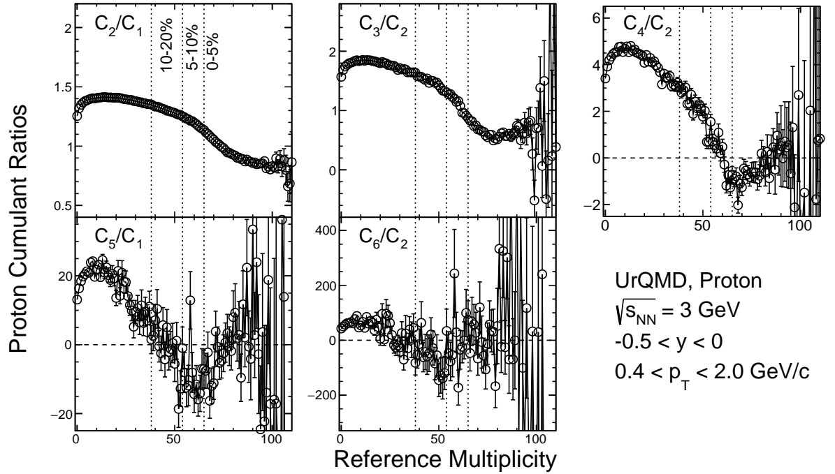
FIG. 13: UrQMD results of proton cumulant ratios up to 6 th -order in Au+Au collisions at \sqrt{s_{NN}} = 3 GeV. The vertical dashed lines indicate the centrality classes.
