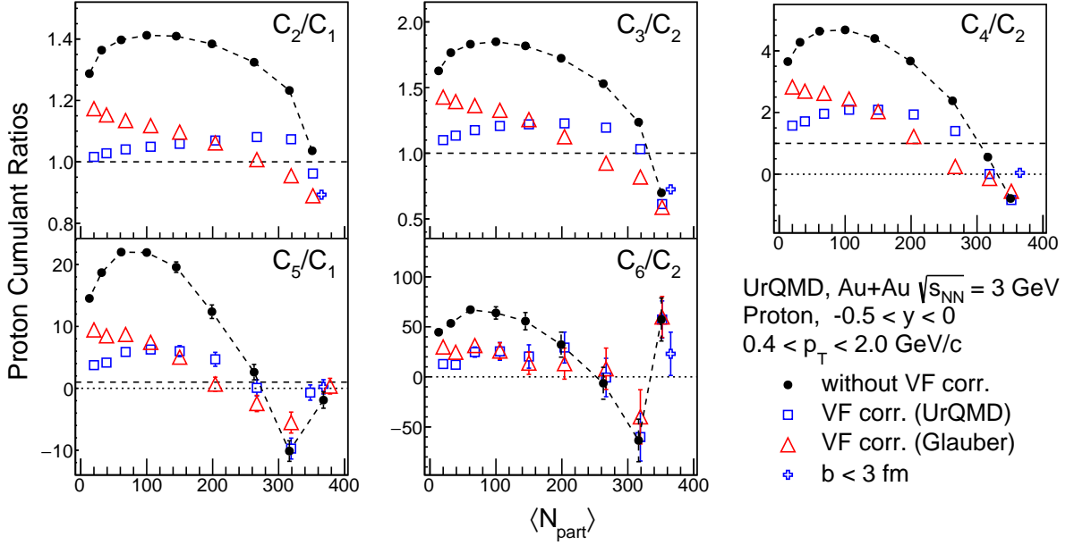
FIG. 10: UrQMD results of the proton cumulant ratios up to 6 th -order in Au+Au collisions at \sqrt{s_{\text{NN}}} = 3 GeV. The black circles are without VF correction while blue squares and red triangles are results with VFC which used N_{\text{part}} distributions from UrQMD and Glauber model, respectively. The blue crosses are calculations using UrQMD events with b \leq 3 fm. The above results are applied CBWC except for the one (blue crosses) using b \leq 3 fm events.
