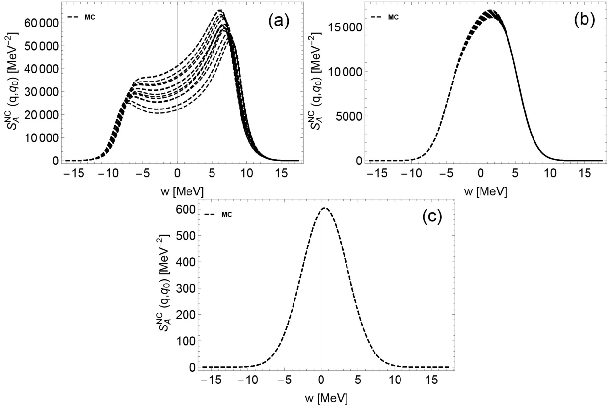
FIG. 7: NC dynamic response based on MC EoSs in axial-vector current channel at T=10 MeV, with q = 3T = 30 MeV. The panel a, b and c are the dynamic response functions at n = 0.15, 0.005, 10^{-4} \text{ fm}^{-3} respectively.
