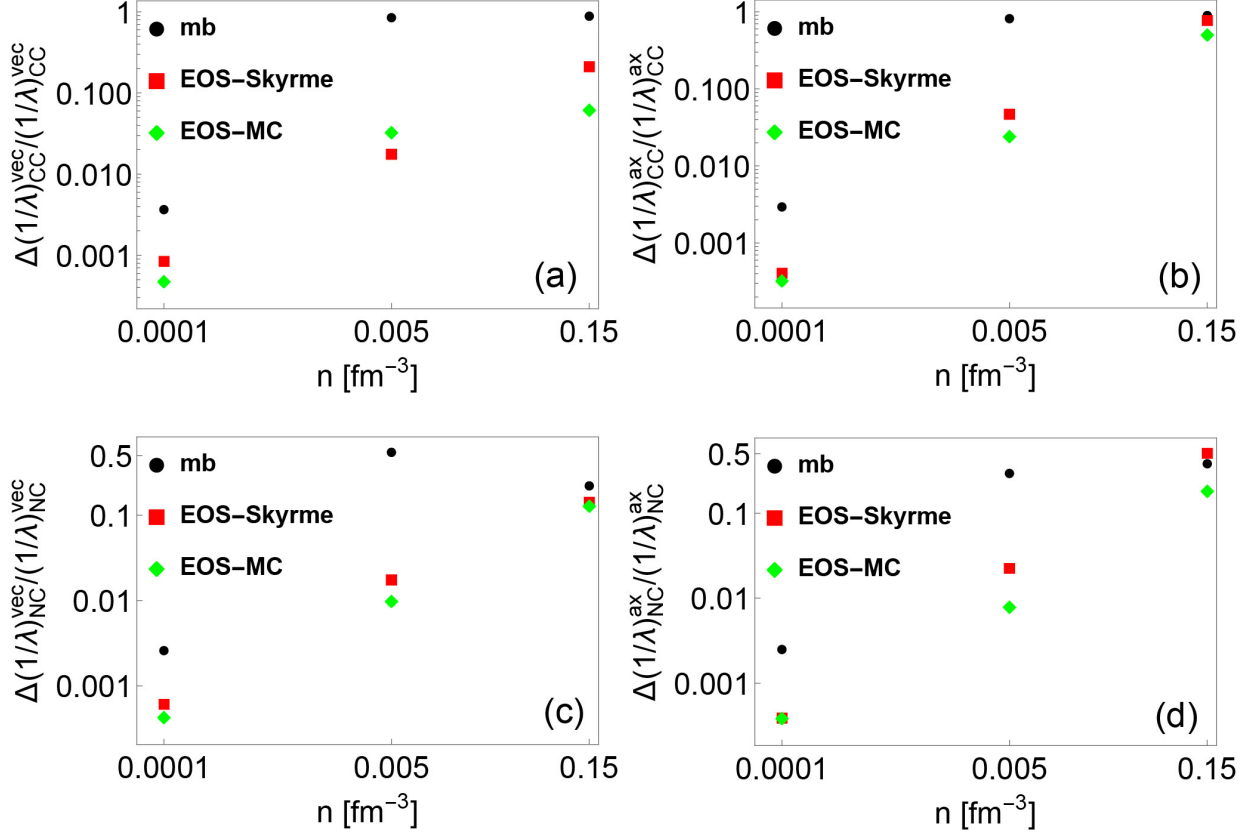
FIG. 5: This figure shows the CC (panel a and b) and NC (panel c and d) uncertainties of IMFPs in vector (panel a and c) and axial vector (panel b and d). The points labeled “mb” show the uncertainty due to many-body methods by showing the difference between the RPA and mean-field estimates for pure Skyrme models. The points labeled “EOS-Skyrme” show the uncertainty due to the constraints used in obtaining the Skyrme-type EOSs. This was computed by comparing the variation across pure Skyrme models which were generated with fits to different sets of nuclear data. Finally, the points labeled “EOS-MC” show just the uncertainties in the mean free path across the Monte Carlo EOSs, which shows the variation due to the inability of the Skyrme model to precisely reproduce the experimental data from McDonnell et al. (2015). See section. III for detailed discussion of the classification of IMFP uncertainties.
