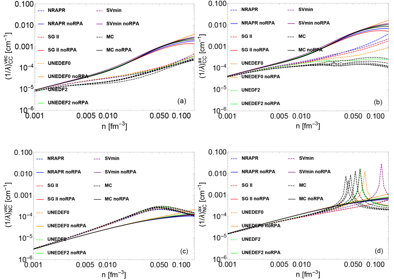
FIG. 4: CC (panel a and b) and NC (panel c and d) IMFPs with and without RPA corrections in vector (panel a and c) and axial vector (panel b and d) channel at T=10 MeV. The colored solid curves stand for IMFPs derived from Skyrme and MC EoSs without RPA corrections. The colored dashed curves stand for IMFPs derived from Skyrme and MC EoSs with RPA corrections. The small peaks observed in a few MC curves are due to the numerical noise.
