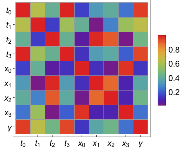
FIG. 8: Pearson coefficients between Skyrme parameters t_i , x_i and \gamma .
