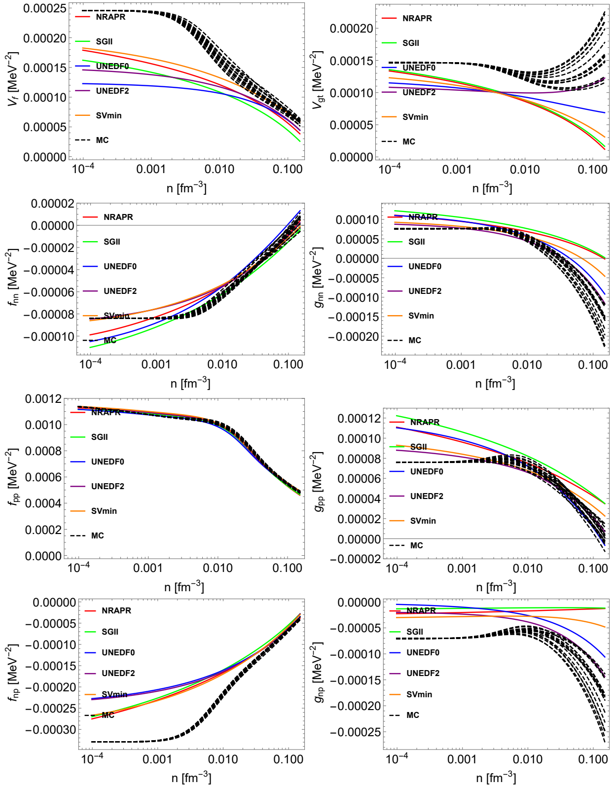
FIG. 1: Residual interactions as function of density. In the left column, residual interactions in vector current channel are shown. In the right column, residual interactions in axial vector current channel are shown. The colored solid curves stand for residual interactions derived from Skyrme-type interactions. The black dashed curves stand for residual interactions derived from MC EoSs, see section II for detailed description of the underlying EoSs used to derive the residual interactions. The detailed formula expression of the residual interactions in NC(CC) channel are provided in the Appendix (see Eqs. (A35), (A38), (A42), and (A43) for NC residual interaction, and Eqs. (A45) and (A46) for CC residual interactions).
