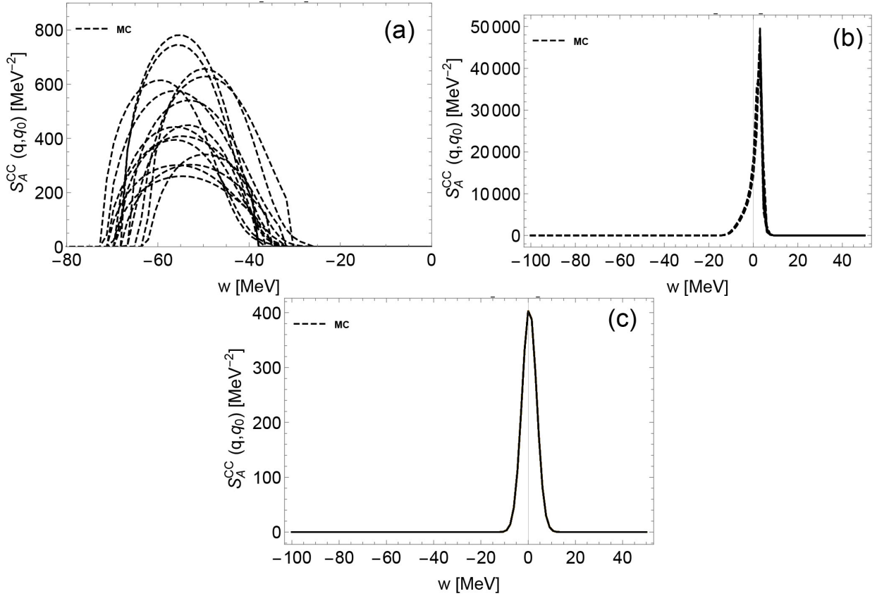
FIG. 6: CC dynamic response based on MC EoSs in axial-vector current channel at T=10 MeV, with q = 3T = 30 MeV. The panel a, b and c are the dynamic response functions at n = 0.15, 0.005, 10^{-4} \text{ fm}^{-3} respectively.
