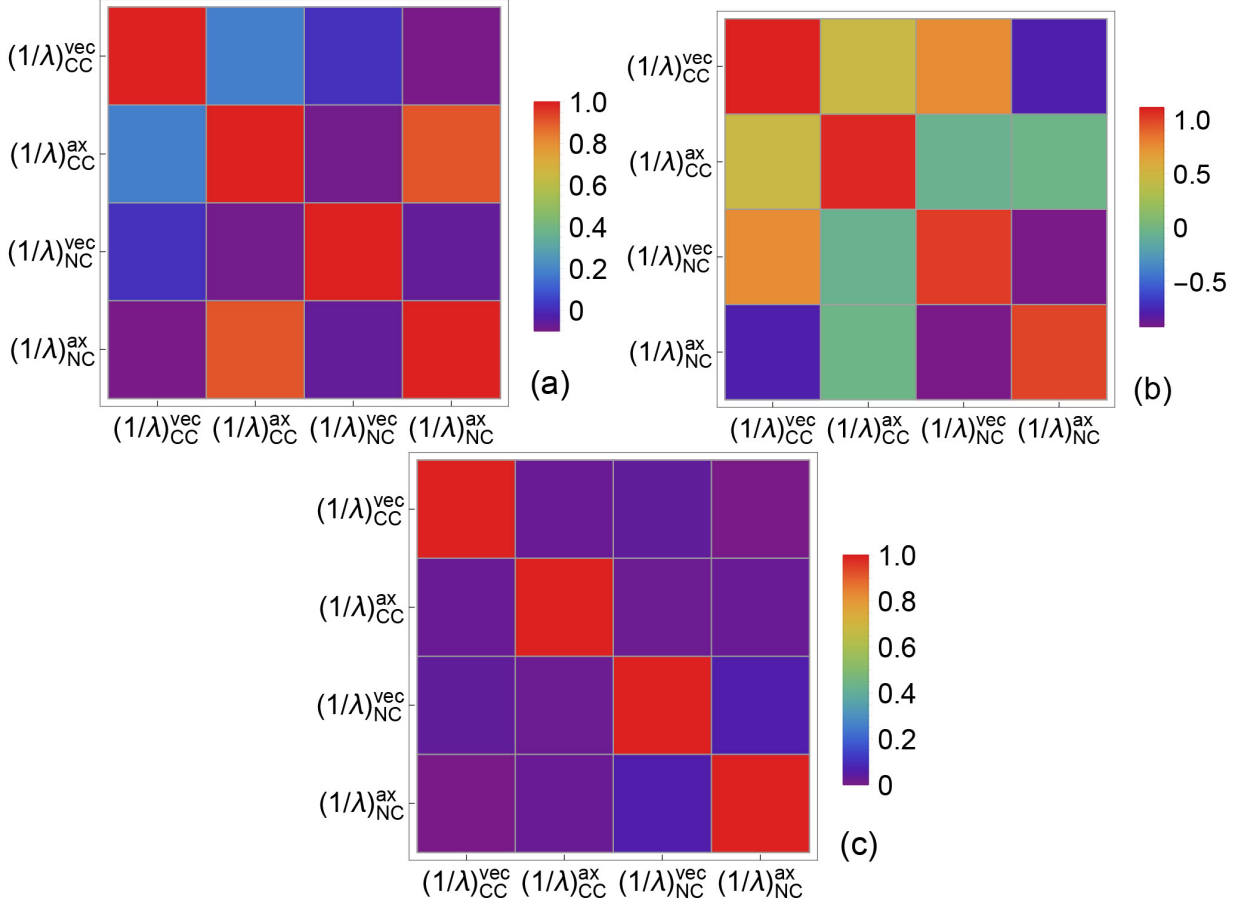
FIG. 12: Pearson coefficients between IMFPs at n = 0.15 fm ^{-3} (a), n = 0.005 fm ^{-3} (b) and n = 10^{-4} fm ^{-3} (c).
