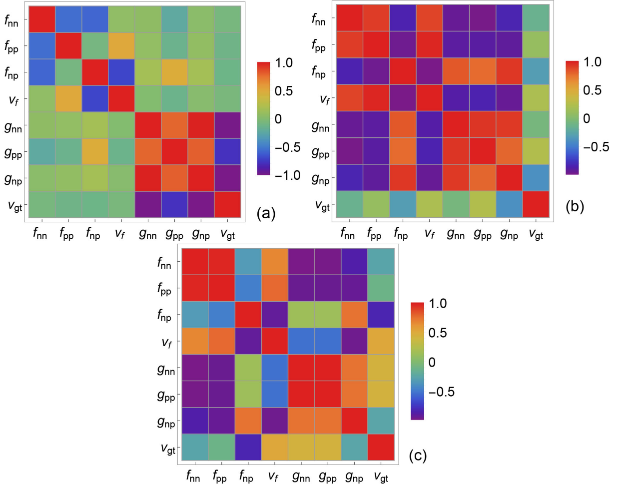
FIG. 9: Pearson coefficients between residual interactions at n = 0.15 \text{ fm}^{-3} (a), n = 0.005 \text{ fm}^{-3} (b) and n = 10^{-4} \text{ fm}^{-3} (c).
