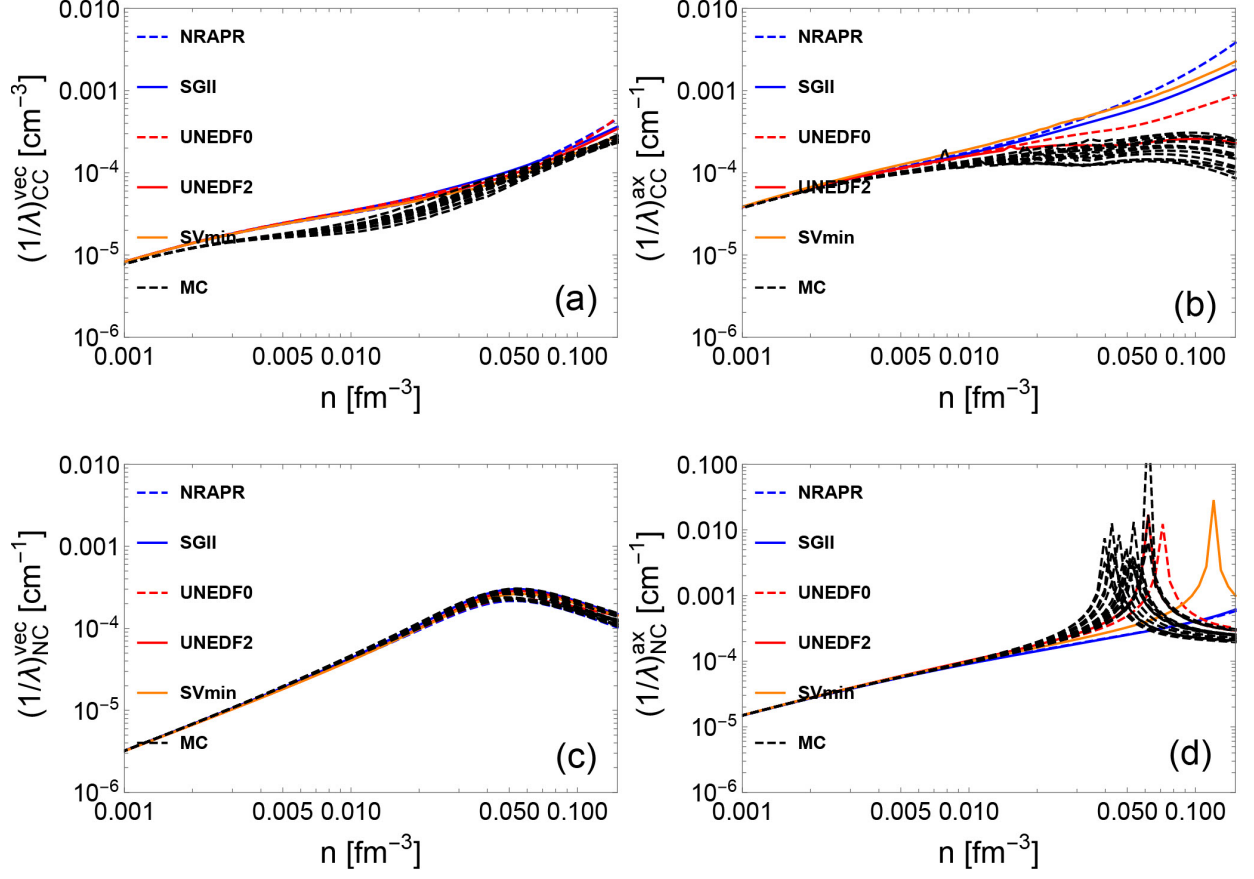
FIG. 2: CC (panel a and b) and NC (panel c and d) IMFPs in vector current (panel a and c) and axial-vector current (panel b and d) channel at T=10 MeV. The colored solid curves stand for IMFPs derived from Skyrme-type interactions. The black dashed curves stand for IMFPs derived from MC EoSs, see section II for detailed description of the underlying EoSs used to derive the residual interactions.
