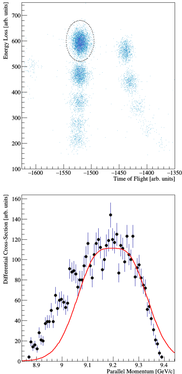
FIG. 1: (Top Panel) Particle identification plot for reaction residues detected in the S800 focal plane following reaction of incoming ^{25}\text{F} . The ^{24}\text{O} reaction residues are highlighted in the dashed oval. (Bottom Panel) Parallel momentum distribution for ^{24}\text{O} reaction residues following proton removal from ^{25}\text{F} . The red line is a calculation of the expected distribution for removal of an \ell=2 proton, folded with the experiment response, and shows good agreement with the width of the distribution. See text for further details.
