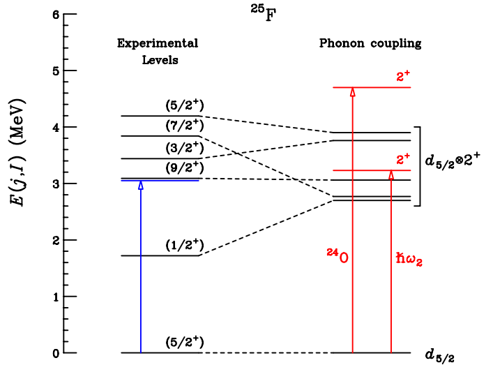
FIG. 2: The experimental level scheme of ^{25}\text{F} from Ref. [28] and the results of the PVC model showing the phonon splitting at first order. For reference, the energies of the 2^+ states in ^{24}\text{O} and of the effective ^{24}\text{O}^* core are shown in red. The phonon frequency determined from the spin weighted average of the multiplet is indicated in blue.
