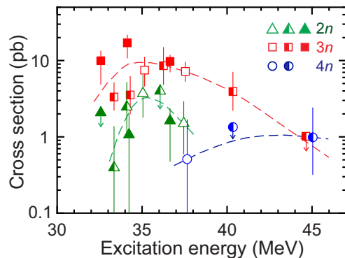
FIG. 2: (Color online) Cross sections for the 2n -, 3n -, and 4n -evaporation channels for the ^{243}\text{Am} + ^{48}\text{Ca} reaction. Vertical error bars correspond to total uncertainties. Symbols with arrows show upper cross-section limits. Data shown by open, half-closed, and closed symbols are from [6], [2], and this work, respectively. The dashed lines through the data are drawn to guide the eye.
