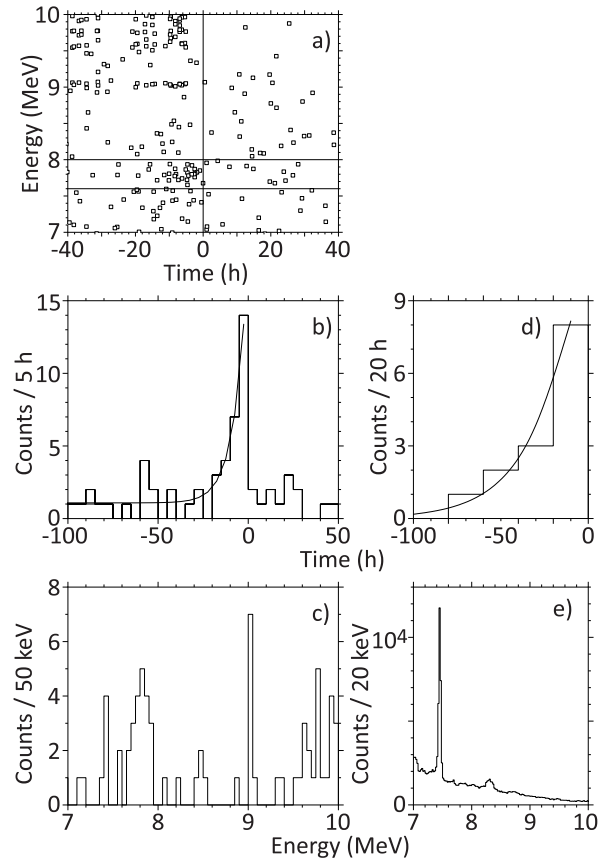
FIG. 1: Energy distribution of \alpha -like events as a function of their detection time with respect to the SF registration time (a), time distribution of events with E_\alpha = 7.6 - 8.0 MeV (b), and energy distribution of events registered in the time interval of 10 hours to SF (c). The most part of events with E_\alpha \geq 9 MeV originates from \alpha decays of ^{272}\text{Bh} - ^{284}\text{Nh} [19]. Fig. 1(d) shows the decay curve of ^{268}\text{Db} , see text. Fig. 1(e) presents the spectrum of \alpha -like events registered during all three runs.
