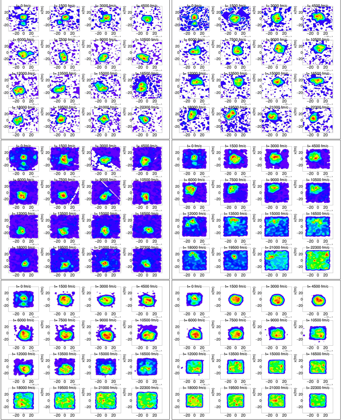
FIG. 2: Evolution of the system ^{140}\text{Ni}+^{460}\text{U} in the nucleon bath with 10% proton concentration calculated using the CoMD code at beam energy 0.01 \text{ MeV/nucleon} and Coulomb interaction cutoff at 10, 7, 5, 4, 3 and 2 fm (from top to bottom and left to right), corresponding to nucleon bath densities \rho_0/100 , \rho_0/50 , \rho_0/30 , \rho_0/17 , \rho_0/10 , and \rho_0/5 , respectively. Incompressibility is K_0 = 254 \text{ MeV} and a soft density dependence of symmetry energy were used. The initial distance is 25 fm. On the time scale up to 25000 fm/c the resulting nucleus appears to dissolve in the nucleon bath with density above \rho_0/30 , even sooner with increasing density.
