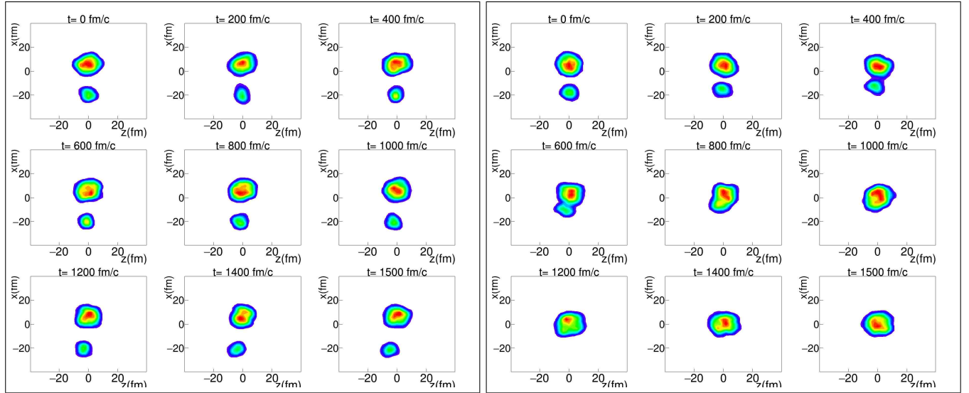
FIG. 1: Typical evolution of nucleonic density for central collision ^{140}\text{Ni} + ^{460}\text{U} calculated using the CoMD code at beam energy 1.25\text{ MeV/nucleon} (Left panel) and 1.5\text{ MeV/nucleon} (Right panel). A Coulomb interaction cutoff 2\text{ fm} , incompressibility K_0 = 254\text{ MeV} and a soft density dependence of symmetry energy were used. Scattering due to a "neutron wind" dominates at lower beam energy (Left panel), while fusion dominates at higher beam energy (Right panel).
