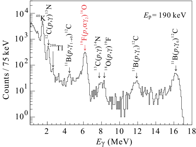
FIG. 3. Typical \gamma -ray spectrum measured at JUNA with a 4\pi BGO array at E_p = 190 \text{ keV} . The 6130-keV \gamma -ray peak for the ^{19}\text{F}(p, \alpha \gamma)^{16}\text{O} reaction is indicated by the red text.
