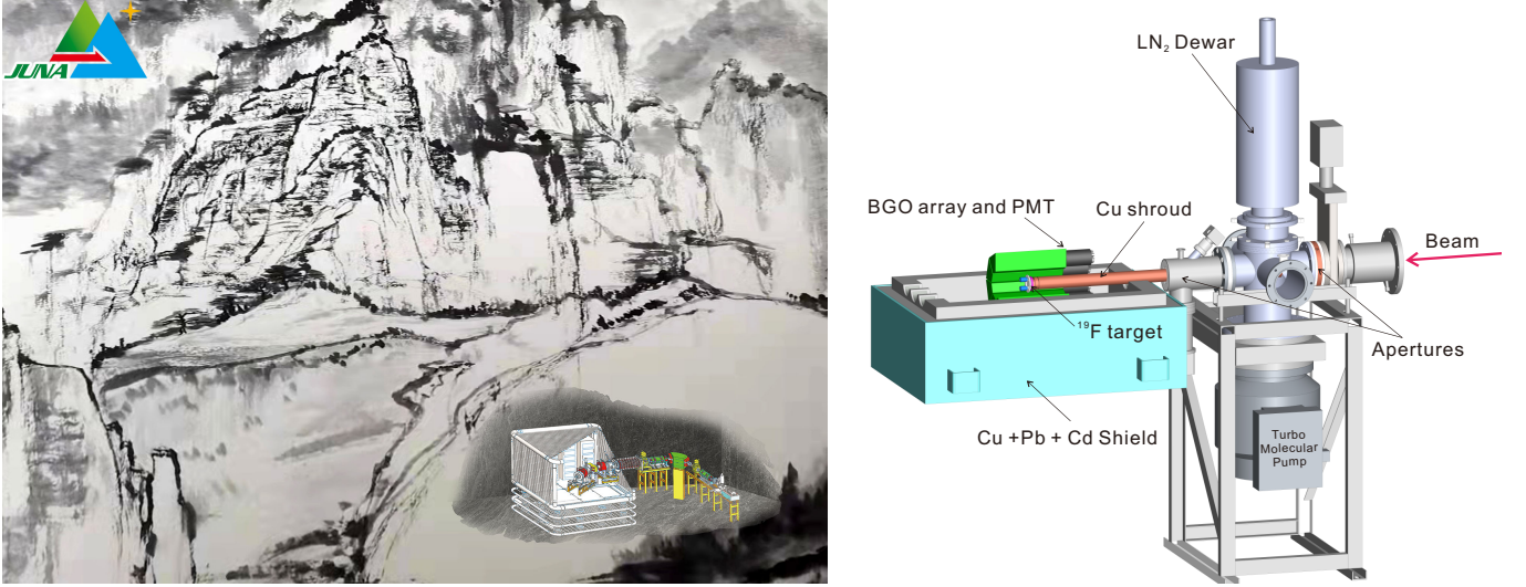
FIG. 2. (Left panel) A combination of science and art rendition of the experimental site and platform for JUNA (credited to L.G. Chen for Chinese ink painting); (Right panel) 3D schematic view of the experimental setup.
