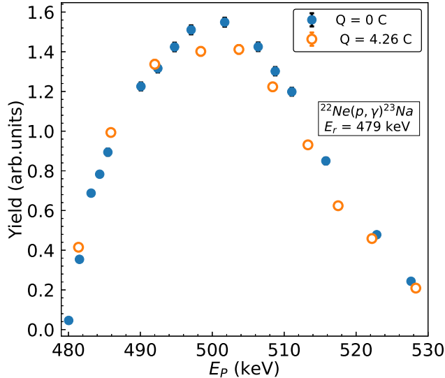
FIG. 4. Yield curve for the E_p^{\text{lab}} = 479 keV resonance in the ^{22}\text{Ne}(p, \gamma)^{23}\text{Na} reaction. The yield curve is obtained from the sum peak in HECTOR [19]. The filled-circle (blue) and open-circle (orange) data points show the difference in yield at the beginning and at end of the experiment. The statistical error in the data is \simeq 1\% , which is why the error bars are not visible.
