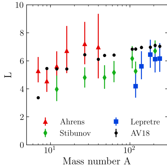
FIG. 2. Average Levinger constant for several nuclei with AV18 comparing to extractions from experiment. The change in predicted L from varying the interval of momentum q over which L is averaged (see text for details) is smaller than the the black AV18 circles.
