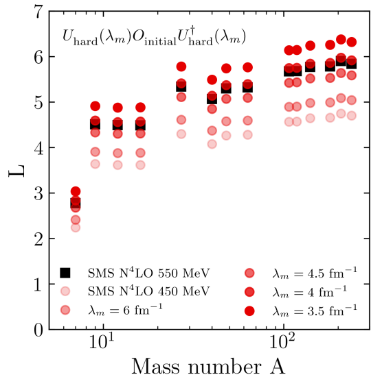
FIG. 6. Average Lvinger constant for several nuclei comparing the SMS N 4 LO 550 MeV (black) and 450 MeV (red) potentials. Results are also shown for the SMS N 4 LO 450 MeV potential with an additional two-body operator due to inverse-SRG transformations from SMS N 4 LO 550 MeV at several values of \lambda_m .
