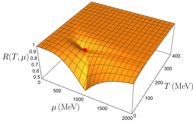
FIG. 2. The dimensionless function R with parameters given in the text. The critical point is indicated by the solid dot.
