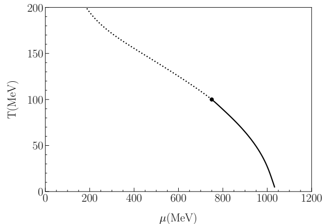
FIG. 1. The choice of critical curve as described in the text. The critical temperature is taken to be 100 MeV and the critical chemical potential to be 750 MeV.
