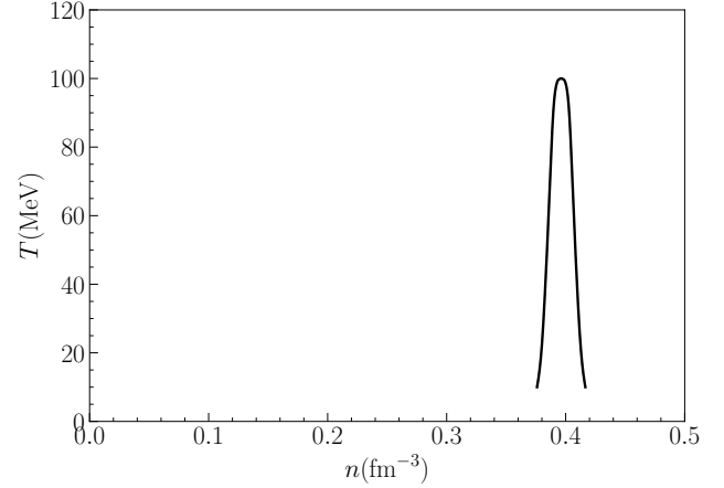
FIG. 4. Temperature versus density separating the two phases.
