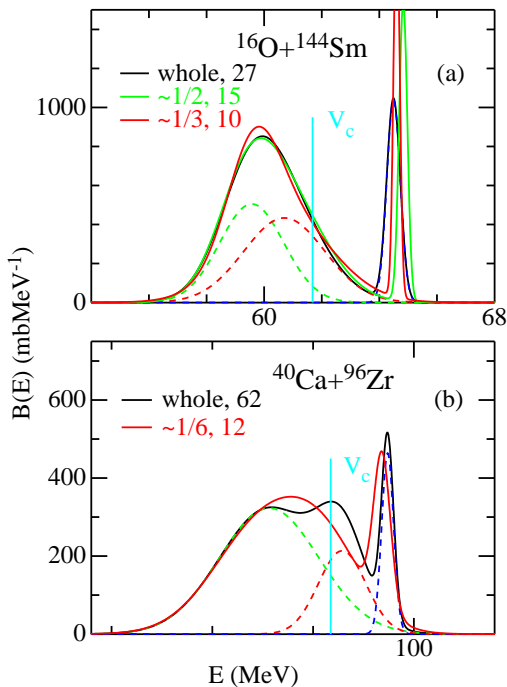
FIG. 6: B(E) spectra for the systems ^{16}\text{O} + ^{144}\text{Sm} [33] (a) and ^{40}\text{Ca} + ^{96}\text{Zr} [30] (b). Solid curves are obtained by using a 3G description for whole or for subsets of the measured cross sections. Dashed curves are the three corresponding components for whole.
