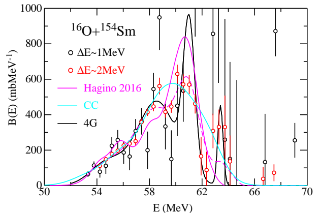
FIG. 5: B(E) spectrum for the system ^{16}\text{O} + ^{154}\text{Sm} . Curves are obtained by using a 4G description, CC and Hagino's analysis by using 5 components of the Wong formula.
