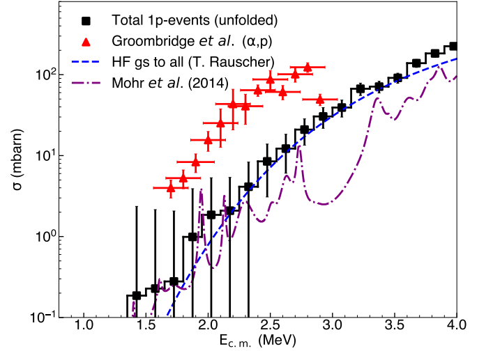
FIG. 14. Comparison of the total (\alpha, p) cross section of this work with the previously obtained (\alpha, p) cross section by Groombridge et al. [10], as well as with theoretical calculations by Mohr et al. [19] and the Hauser-Feshbach code SMARAGD [26, 27]. Only statistical errors are shown.
