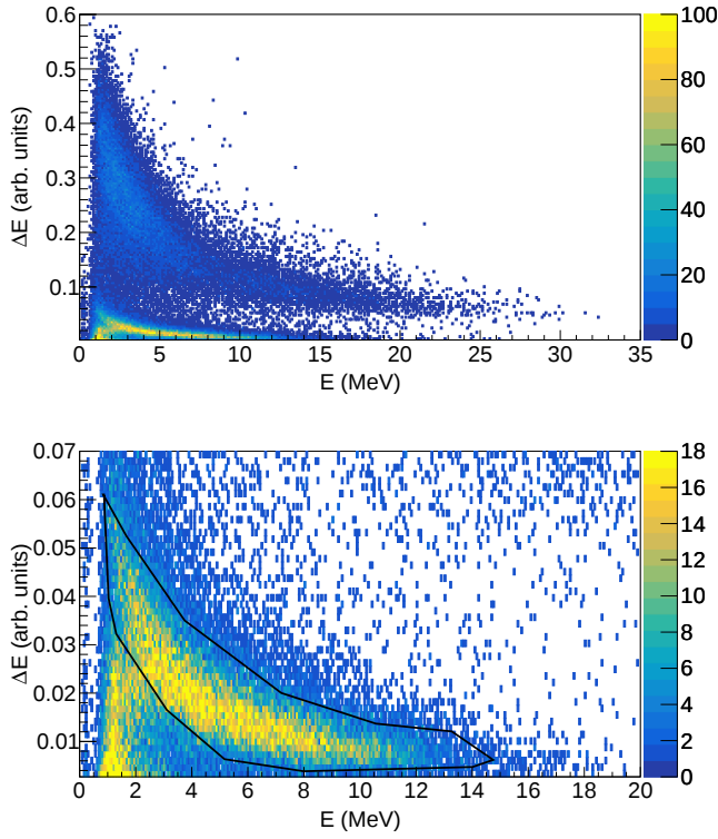
FIG. 2. Top: Energy-loss signals of the proportional-counter anodes vs. the coincident silicon detector signal. The energy-loss information ( \Delta E ) is derived from the PC signals, corrected for the angle-dependent thickness of the active detector volume, and the residual energy ( E ) is measured in the Si detectors. Protons and \alpha -particles show distinct, separate correlation groups. Bottom: Display of the same (Top) histogram expanded to show the region of proton signals and their selection gate.
