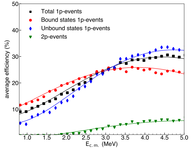
FIG. 10. Average detection efficiencies from a Monte-Carlo simulation of the (\alpha, p) reaction and the corresponding detector response, averaged over various ^{21}\text{Na} excitation-energy regions. Also shown is the efficiency for the coincident detection of two protons from the (\alpha, 2p) reaction
