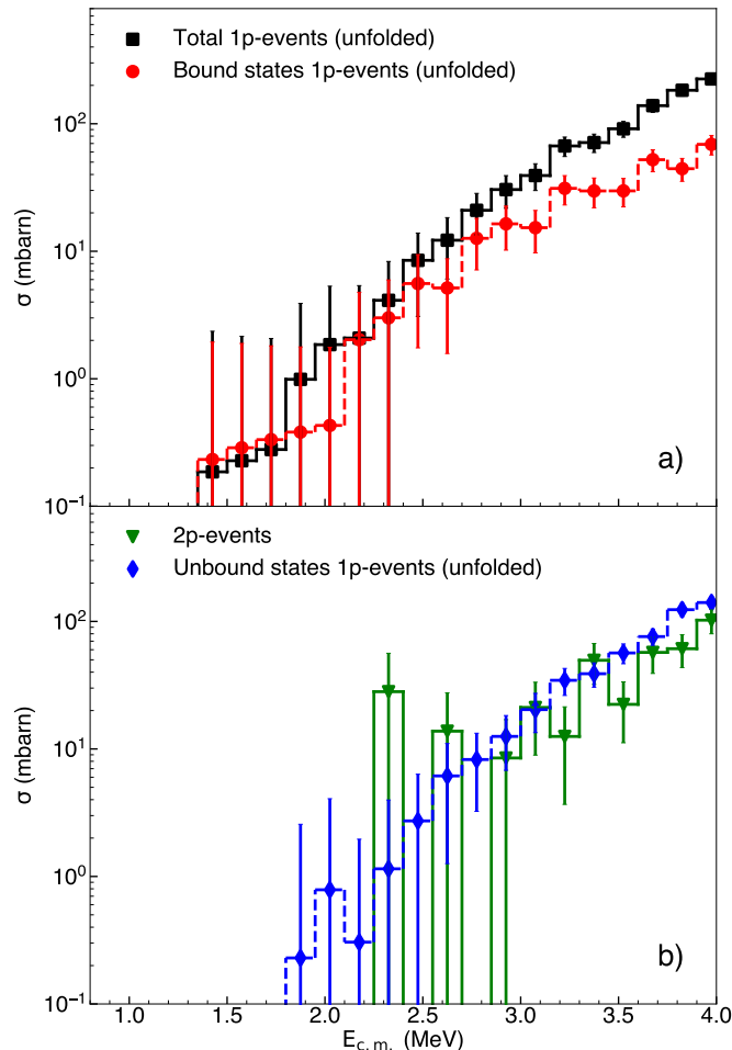
FIG. 12. Panel (a): Cross sections from single-proton events determined from this work and corrected for the experimental energy resolution. The total cross section (black) is compared to cross section for bound states only (red). Panel (b): The unbound states cross sections from the single-proton events analysis, corrected for the experimental energy resolution, compared to the cross section obtained from the independent analysis of the coincident 2p -events. Due to higher resolution, the 2p -events cross section is not subjected to the Gaussian unfolding procedure. Only statistical errors are shown.
