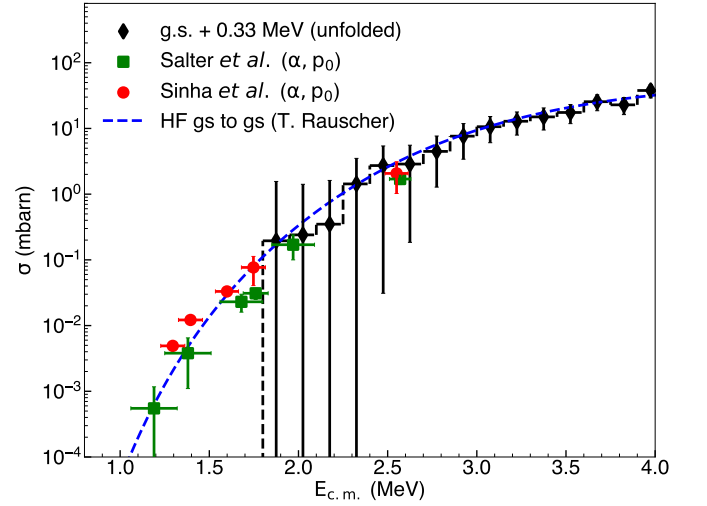
FIG. 13. The ground state cross section, including the first excited state at 0.33 MeV, after resolution adjustment. Previously collected data by Sihna et al. [11] and Salter et al. [12] that correspond to the ground state transition, and the Hauser-Feshbach calculation for ground-state to ground-state transitions are plotted for comparison. Only statistical errors are shown.
