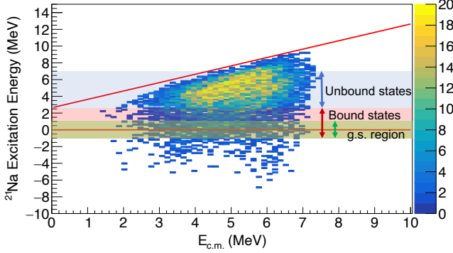
FIG. 4. Single-proton events: Distribution of ^{21}\text{Na} excitation energies with respect to the reaction energy in the center-of-mass frame, reconstructed using the E_{\text{track}} method. The two lines delimit the kinematically allowed event range. The highlighted regions in green, red and blue represent the ground state, bound states' (including the ground-state region) and unbound states' regions respectively, as used in the cross-section analysis of Sect. IV.
