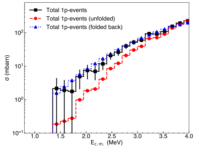
FIG. 11. Demonstration of the unfolding of the observed experimental cross section spectrum with respect to its Gaussian resolution, following the 2-step iteration of the Richardson-Lucy algorithm. The process is verified by folding back the unfolded spectrum with the Gaussian resolution. The error bars on the unfolded and folded-back spectrum are omitted for clarity.
