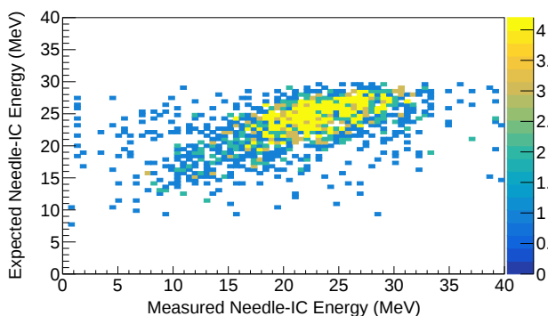
FIG. 8. Two-proton events: Correlation between “expected” and “measured” Needle-IC signals, gated on the ^{20}\text{Ne} ground-state peak.
