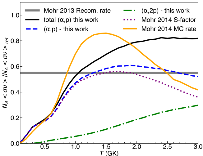
FIG. 15. Comparison of the reaction rates of this work and Mohr et al. 2014 work [19] to the reference reaction rate N_A \langle \sigma v \rangle_{ref} determined in Ref. [18]. The flat line at 0.55 N_A \langle \sigma v \rangle_{ref} is the recommended reaction rate from Ref. [18]. The total (\alpha, p) reaction rate of this work is larger by a factor of 1.5 from the recommended rate of Ref. [18] due to the contributions of the ^{21}\text{Na} unbound states.
