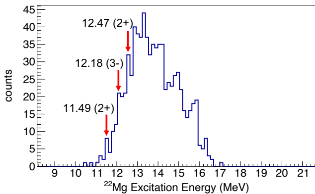
FIG. 7. Two-proton events: ^{22}\text{Mg} excitation-energy distribution reconstructed from the ^{20}\text{Ne}+2p energies and the E_{\text{kine}} method.
