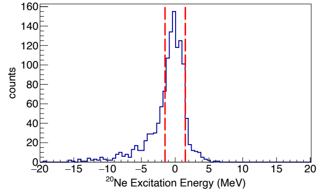
FIG. 5. Two-proton events: ^{20}\text{Ne} excitation-energy distribution, using the E_{\text{track}} -reconstruction of the reaction energies. The gate around the main peak, between Ex [-1.5,1.5] MeV, is used in the analysis of the two-proton events.
