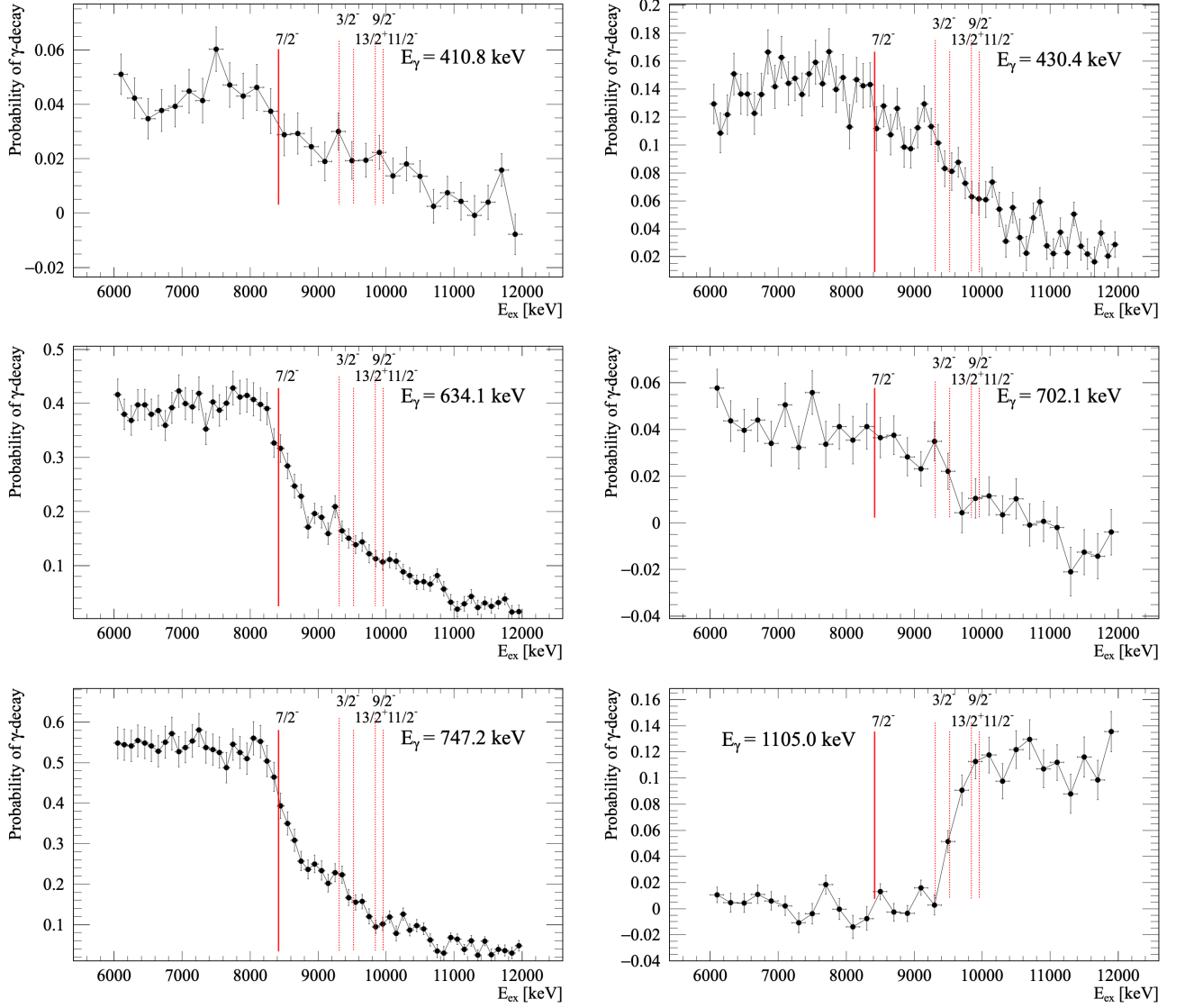
FIG. 8. Extracted \gamma -decay probabilities for the transitions in ^{146}\text{Sm} , via the (p, t) reaction channel. The solid line denotes the neutron separation energy S_n , and the dotted lines correspond to the energies of the first few discrete states in ^{145}\text{Sm} . The spins and parities of the ^{145}\text{Sm} levels are noted on the figure.
