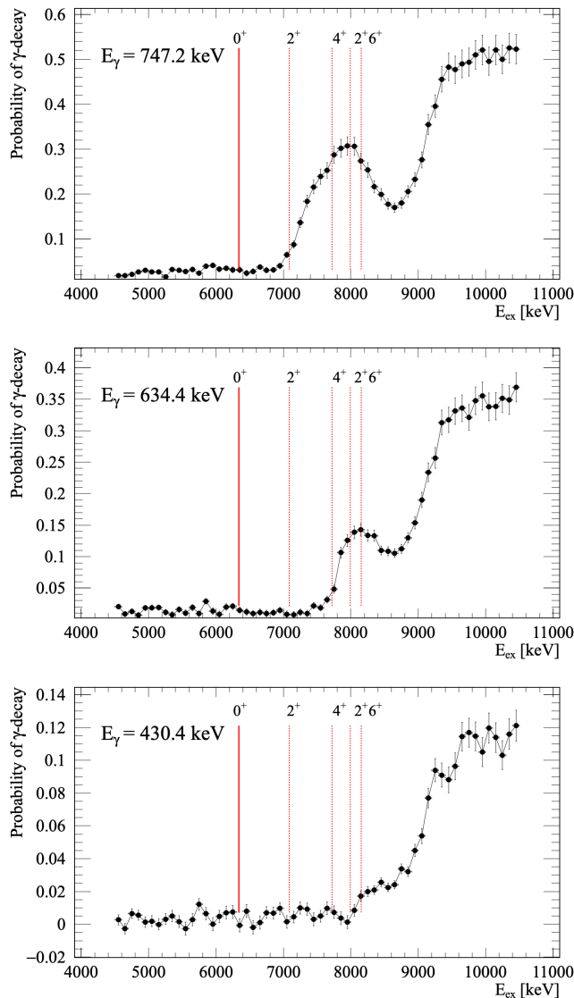
FIG. 5. Extracted \gamma -decay probabilities for the first three transitions in ^{146}\text{Sm} , via the (p, dn) reaction channel. The solid line denotes the neutron separation energy S_n , and the dotted lines correspond to the energies of the first few discrete states in ^{146}\text{Sm} . The spins and parities of the ^{146}\text{Sm} levels are noted on the figure.
