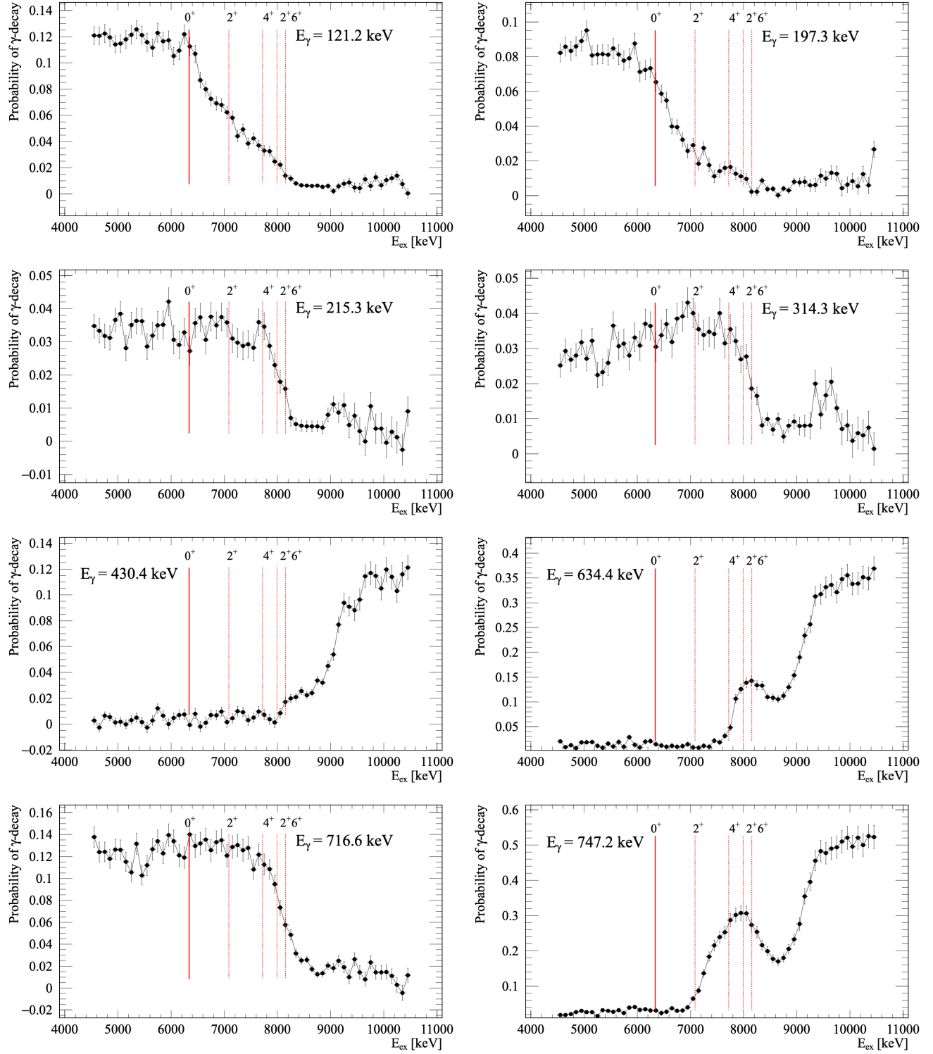
FIG. 6. Extracted \gamma -decay probabilities for the transitions in ^{147}\text{Sm} , via the (p, d) reaction channel. The solid line denotes the neutron separation energy S_n , and the dotted lines correspond to the energies of the first few discrete states in ^{146}\text{Sm} . The spins and parities of the ^{146}\text{Sm} levels are noted on the figure.
