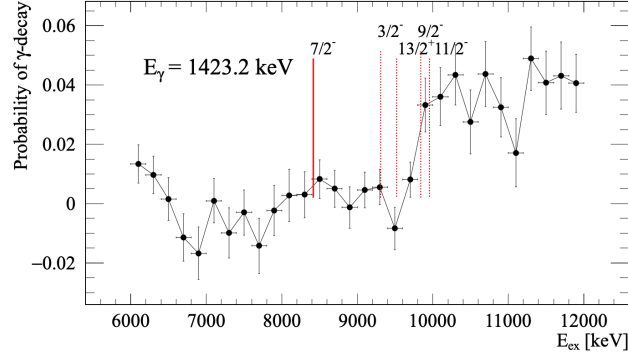
FIG. 9. (continued) Extracted \gamma -decay probabilities for the transitions in ^{146}\text{Sm} , via the (p, t) reaction channel. The solid line denotes the neutron separation energy S_n , and the dotted lines correspond to the energies of the first few discrete states in ^{145}\text{Sm} . The spins and parities of the ^{145}\text{Sm} levels are noted on the figure.
