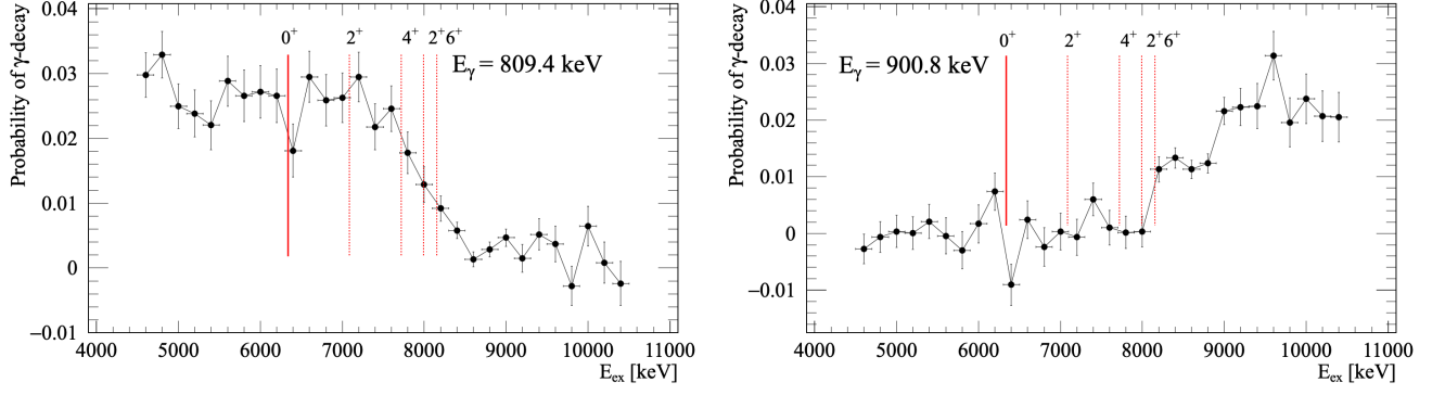
FIG. 7. (continued) Extracted \gamma -decay probabilities for the transitions in ^{147}\text{Sm} , via the (p, d) reaction channel. The solid line denotes the neutron separation energy S_n , and the dotted lines correspond to the energies of the first few discrete states in ^{146}\text{Sm} . The spins and parities of the ^{146}\text{Sm} levels are noted on the figure.
