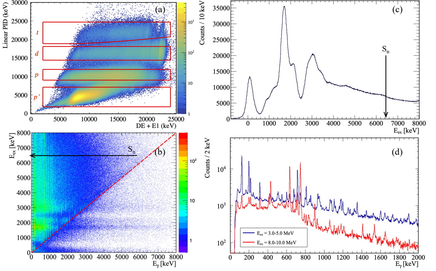
FIG. 1. Example experimental data obtained from the ^{148}\text{Sm}(p,d)^{147}\text{Sm} reaction measured with Hyperion: (a) Linearized particle identification (PID) plot used to select the (p,d) reaction that populates ^{147}\text{Sm} nucleus. Red contours denote coincidence gates applied to select protons, deuterons and tritons in the outgoing particle channel. (b) E_{ex}-E_{\gamma} matrix. The red dashed line denotes E_{ex} = E_{\gamma} . Discrete transitions appear to dominate below about 3.5 MeV, after which point the \gamma -decay seems to follow a probabilistic, continuous behavior. The arrow indicates the neutron-separation energy in ^{147}\text{Sm} . (c) Particle singles spectrum for (p,d)^{147}\text{Sm} channel. The arrow indicated the neutron-separation energy in ^{147}\text{Sm} . (d) \gamma -ray spectrum from the ^{148}\text{Sm}(p,d) reaction. The blue histogram shows \gamma -ray transitions in coincidence with excitation energies between 3.0-5.0 MeV, where only the (p,d) channel is present. The red histogram represents \gamma -ray transitions in coincidence with excitation energies between 8.0-10.0 MeV, where both the (p,d) and (p,dn) channels are open.
