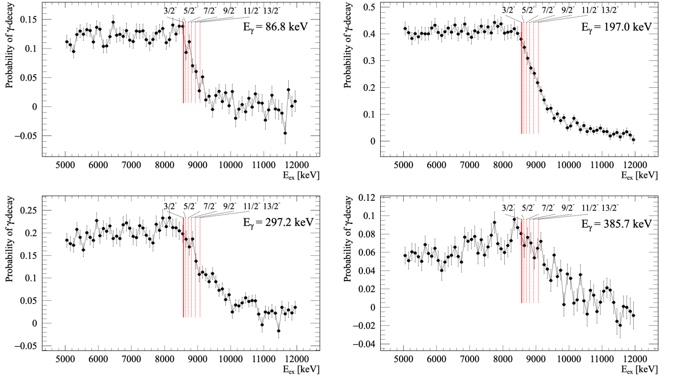
FIG. 10. Extracted \gamma -decay probabilities for the transitions in ^{160}\text{Dy} , via the (p, t) reaction channel. The solid line denotes the neutron separation energy S_n , and the dotted lines correspond to the energies of the first few discrete states in ^{159}\text{Dy} . The spins and parities of the ^{159}\text{Dy} levels are noted on the figure.
