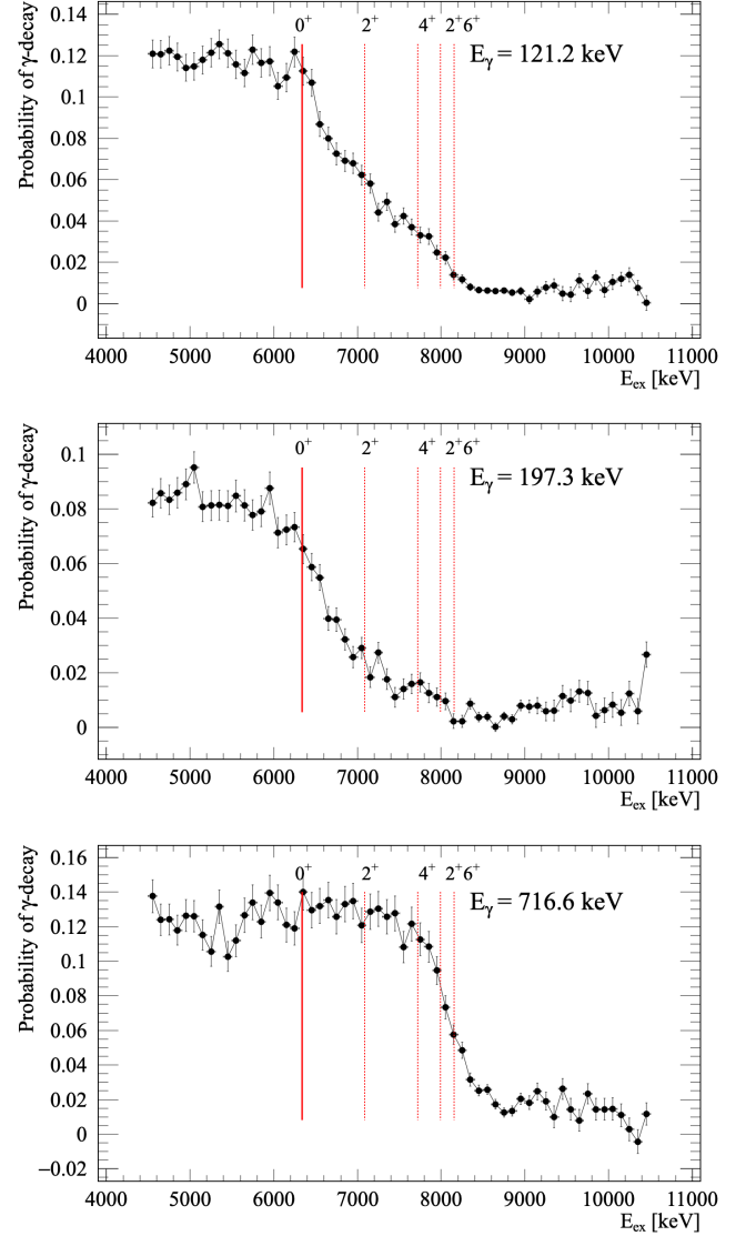
FIG. 4. Extracted \gamma -decay probabilities for the first three transitions in ^{147}\text{Sm} , via the (p, d) reaction channel. The solid line denotes the neutron separation energy S_n , and the dotted lines correspond to the energies of the first few discrete states in ^{146}\text{Sm} . The spins and parities of the ^{146}\text{Sm} levels are noted on the figure.
