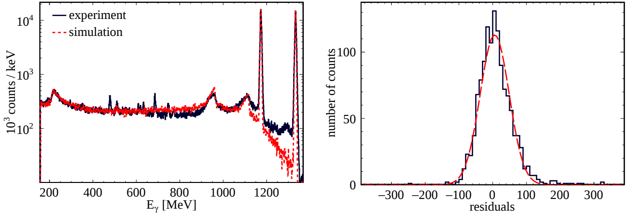
FIG. 2. (Left) A comparison between the Geant4 simulation (red dashed line) and measured spectra (black) for ^{60}\text{Co} . The differences in the spectra are primarily due to contaminants that were present in the singles spectra. (Right) A histogram of residual differences between the measured ^{60}\text{Co} spectrum and a simulated one. A Gaussian fit (red dashed line) was used to determine the width of the distribution.
