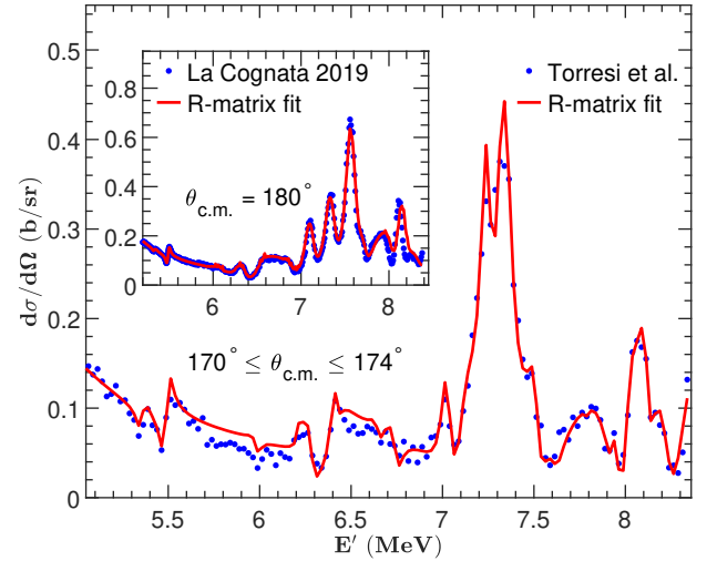
FIG. 3. Excitation function for the \alpha+^{15}\text{O} elastic scattering, points show data from D. Torresi et al, [9]. Inset shows the mirror excitation function for \alpha+^{15}\text{N} scattering and data from La Cognata 2019 [8].
