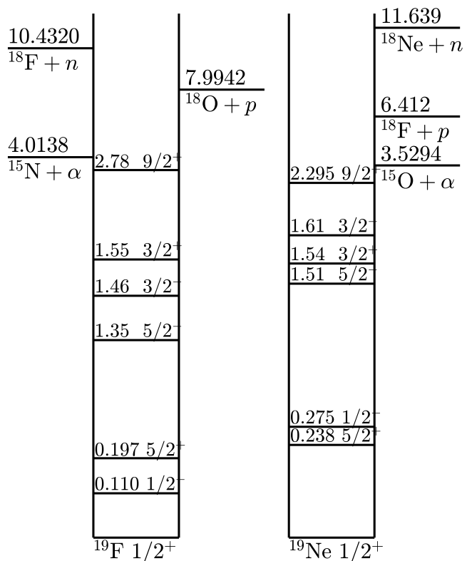
FIG. 4. Scheme of the lowest levels in mirror nuclei ^{19}\text{F} and ^{19}\text{Ne} .
