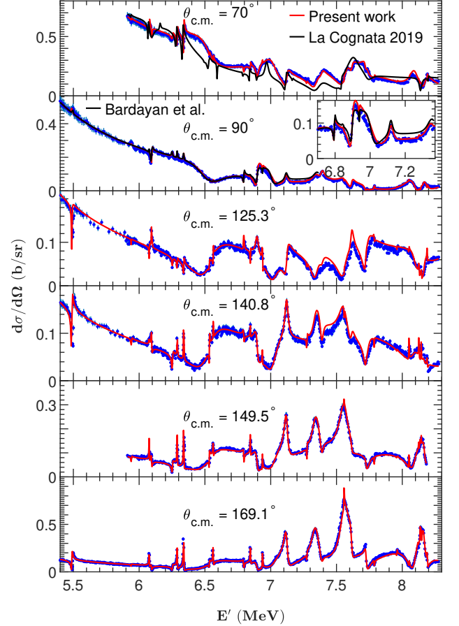
FIG. 1. Excitation functions for the \alpha+^{15}\text{N} elastic scattering [5] and R -matrix fit. See text for explanations. Top panel for 70^\circ compares our calculations to those with parameters from La Cognata 2019 in Ref. [8]; the next panel for 90^\circ includes comparison with the fit with parameters of Bardayan et al in Ref.[6]; inset magnifies the area around 7 MeV.
