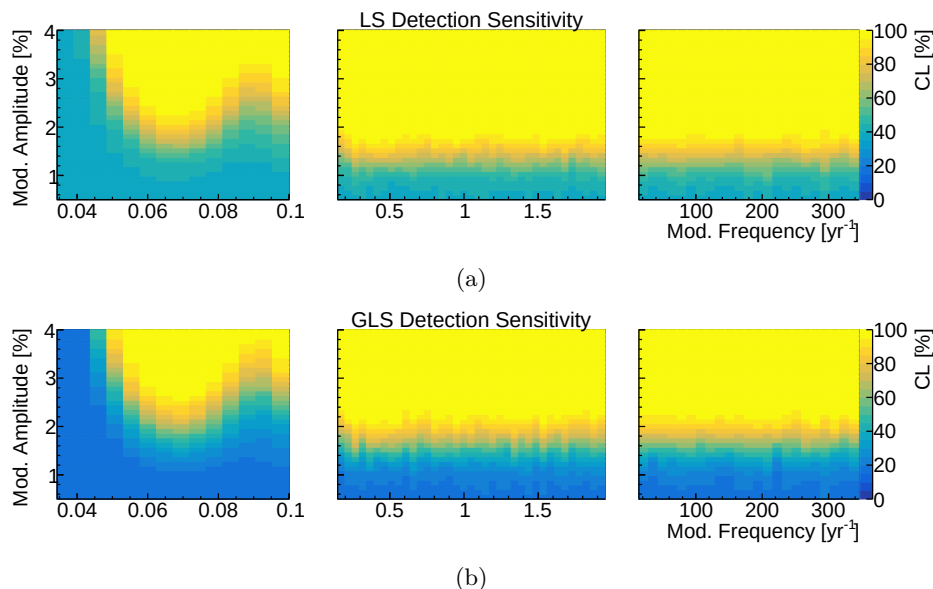
FIG. 3: LS (a) and GLS (b) detection sensitivity as a function of modulation parameters A and f ( \phi = 0 ) in three frequency regimes: low, mid, and high. The z-axis, color, at each point denotes the estimated CL value of the largest peak, averaged over 100 periodograms.
