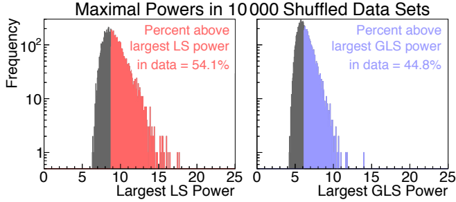
FIG. 2: A distribution of the maximal LS (left) and GLS (right) powers in 10 000 randomly shuffled null-hypothesis data sets (no applied modulations). These distributions are used to calculate the 90% CL lines in Fig 1.
