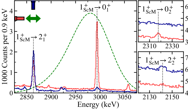
FIG. 1. Three extracts of the ^{150}\text{Nd} NRF spectra of the two HPGe detectors placed perpendicular to the beam axis. The color-coded azimuthal detector positions are indicated in the top left schematic along the \gamma -ray beam's polarization represented by the green arrow. The here discussed 2994 keV 1_{\text{ScM}}^+ state's transitions are labeled and the state's positive parity is apparent through the pronounced azimuthal asymmetry of its 0^+ transitions. The green dashed line represents the beam's intensity profile.
