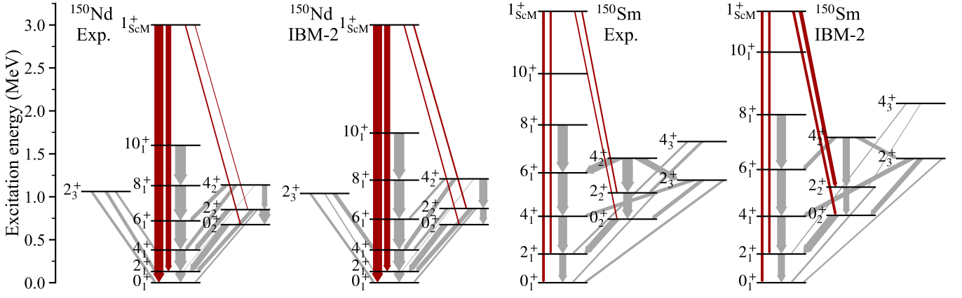
FIG. 3. Comparison of our IBM-2 calculations (using the Hamiltonian of Eq. (3) with its parameters given in Table III) to experimental values for ^{150}\text{Nd} and ^{150}\text{Sm} . The dark red arrows represent the newly obtained M1 transition strengths (line widths \propto B(M1) ), the light gray arrows E2 transition strengths (line widths \propto \sqrt[3]{B(E2)} ). The B(E2) values and excitation energies were taken from [30].
