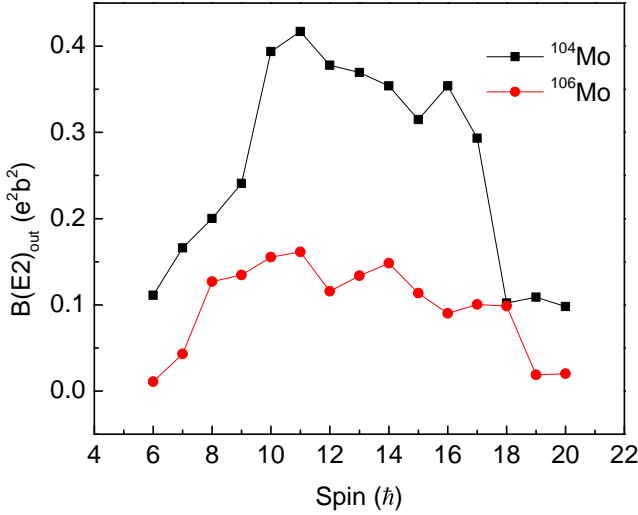
FIG. 20. (Color online) B(E2, I \rightarrow I - 1)_{out} values for the transitions connecting bands 5 and 4 from TPSM calculation.
