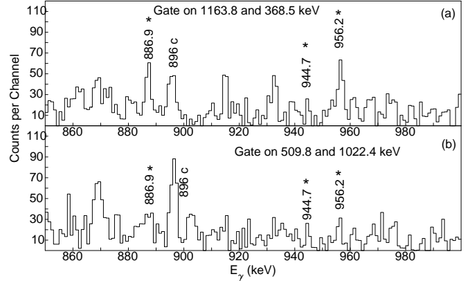
FIG. 7. Partial \gamma -ray coincidence spectra by gating on (a) 1163.8 and 368.5 keV transitions and (b) 509.8 and 1022.4 keV transitions in ^{104}\text{Mo} . New transitions are labeled with an asterisk.
