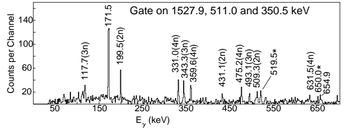
FIG. 11. Partial \gamma -ray coincidence spectra by gating on 1527.9, 511.0 and 350.5 keV transitions in ^{106}\text{Mo} . New transitions are labeled with an asterisk. Fission partner transitions are labeled with neutron evaporation numbers. Here 2n, 3n, 4n, 5n denote ^{144}\text{Ba} , ^{143}\text{Ba} , ^{142}\text{Ba} and ^{141}\text{Ba} , respectively.
