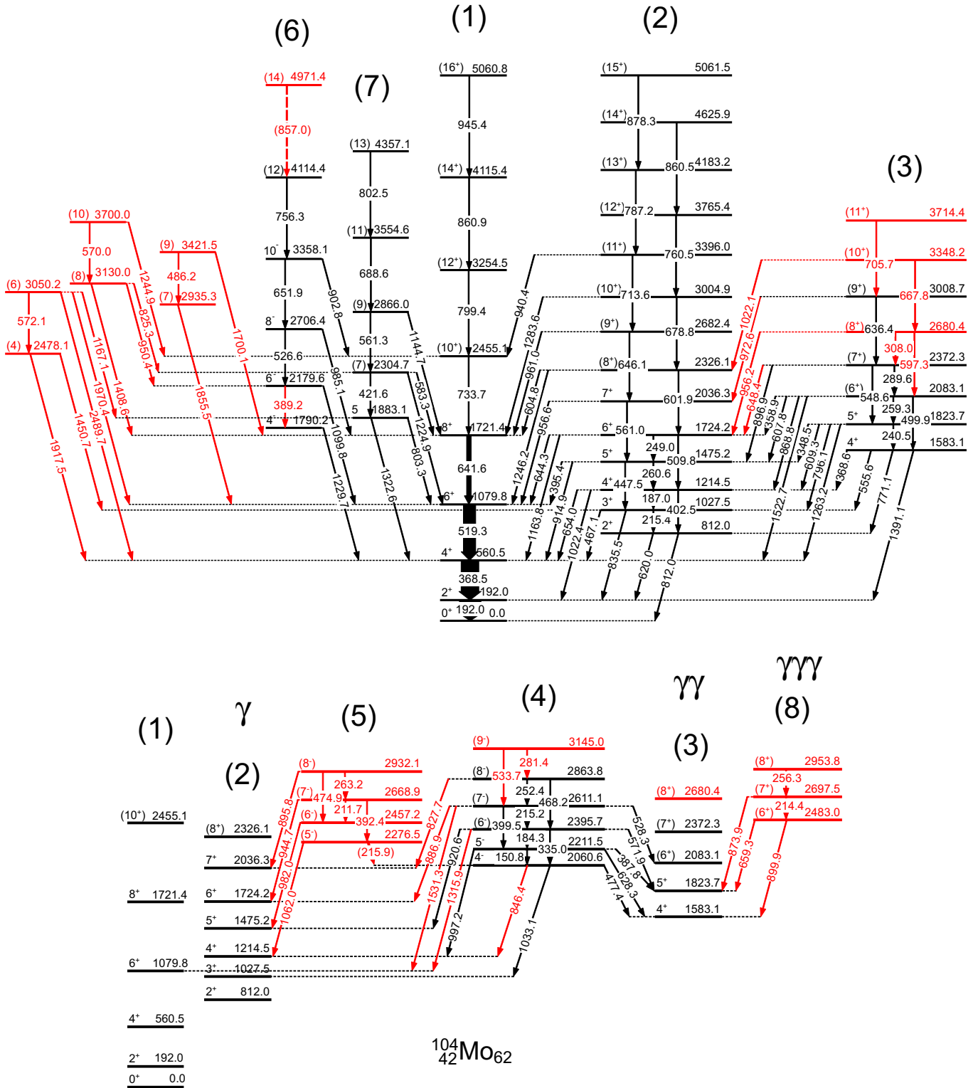
FIG. 1. (Color online) Partial level scheme of ^{104}\text{Mo} obtained in the current work. New levels and transitions are labeled in red.
