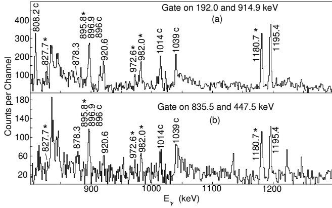
FIG. 4. Partial \gamma -ray coincidence spectra by gating on (a) 192.0 and 914.9 keV transitions and (b) 835.5 and 447.5 keV transitions in ^{104}\text{Mo} . New transitions are labeled with an asterisk. Contamination transitions are labeled with a "c". Note that the 1180 and 1195 keV transitions are not placed in the level scheme.
