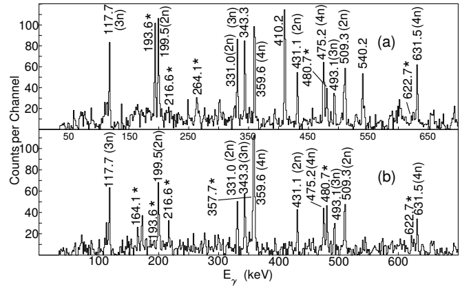
FIG. 10. Partial \gamma -ray coincidence spectra in ^{106}\text{Mo} (a) by gating on the 1780.6, 350.5 and 171.5 keV transitions, and (b) by gating on the 1616.5, 350.5 and 171.5 keV transitions. New transitions are labeled with an asterisk. Fission partner transitions are labeled with neutron evaporation numbers. Namely, 2n, 3n, 4n denote ^{144}\text{Ba} , ^{143}\text{Ba} , ^{142}\text{Ba} , respectively.
