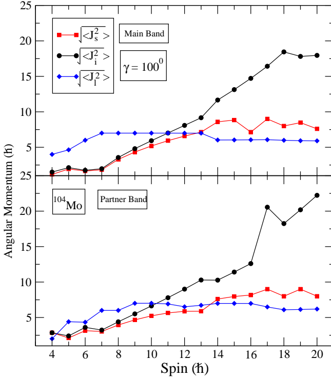
FIG. 21. (Color online) The expectation values of the squared angular momentum components for the main band (B4) and partner band (B5) for the total nucleus in ^{104}\text{Mo} . The value \gamma = 100^\circ was used in order to mitigate small errors caused by the truncation of the configuration space in the TSPM code. The change \gamma = 20^\circ \rightarrow 100^\circ only inter changes the intrinsic order of the axes in the code.
