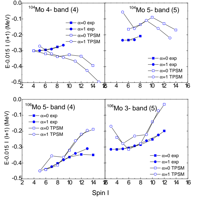
FIG. 14. (Color online) Comparison of the measured energy levels E-0.015 \cdot I \cdot (I+1) vs Spin ( I ) for ^{104,106}\text{Mo} with TPMSM calculated values. Data for ^{106}\text{Mo} has been taken from Ref. [9] and the current work. Here E is normalized to the band 4 bandhead energies in ^{104,106}\text{Mo} , respectively.
