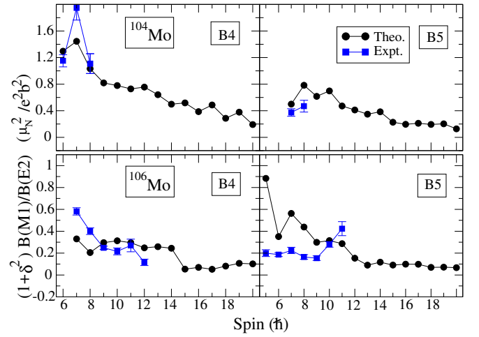
FIG. 19. (Color online) Comparison of the measured B(M1)(\mu_N^2)/B(E2)(e^2b^2) * (1 + \delta^2) shown as square with TPSM calculated values shown as circle for ^{104,106}\text{Mo} nuclei. Here B(M1) depicts \Delta I = 1 chiral in-band reduced transition probabilities, while B(E2) \Delta I = 2 chiral in-band reduced transition probabilities.
