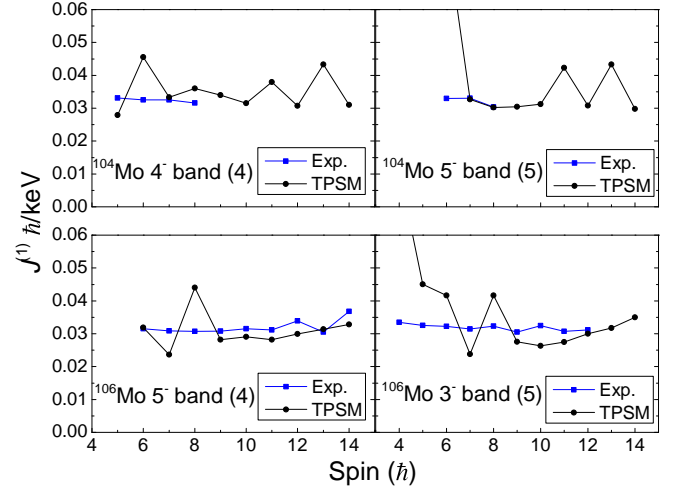
FIG. 18. Comparison of the J^{(1)} moments of inertia in band 4 and 5 between TPSM calculations and experimental data.
