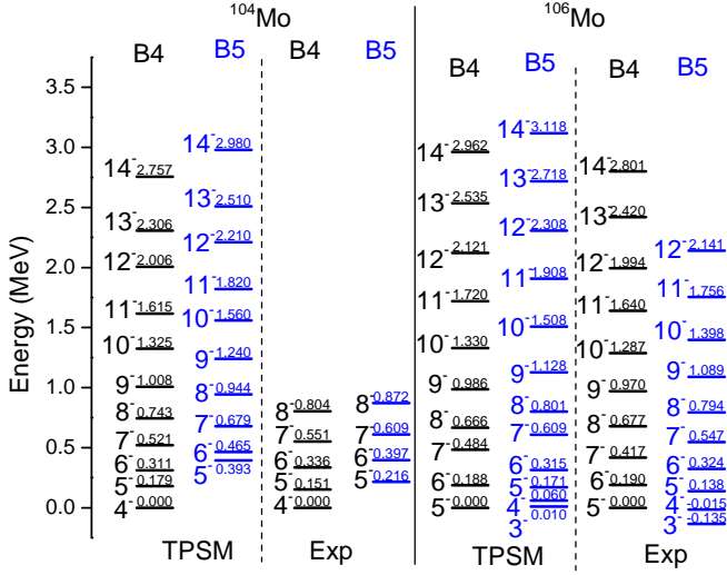
FIG. 17. Comparison of the TPSM calculated energy level to the experimental data. Energies are normalized to the 4^- state of band 4 of ^{104}\text{Mo} and 5^- state of band 4 of ^{106}\text{Mo} , respectively.
