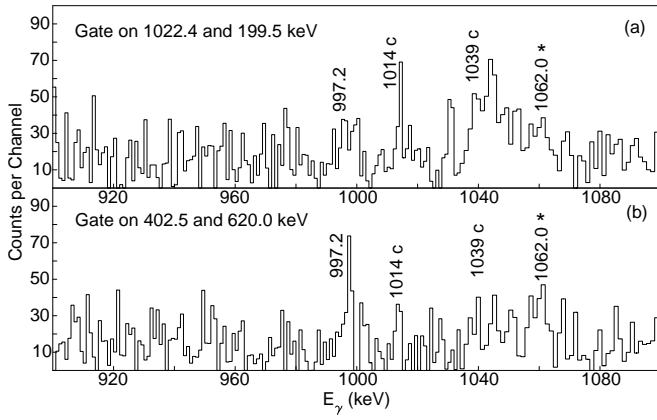
FIG. 8. Partial \gamma -ray coincidence spectra by gating on (a) 1022.4 keV transition in ^{104}\text{Mo} and 199.5 keV transition from the fission partner ^{144}\text{Ba} , and (b) 402.5 and 620.0 keV transitions in ^{104}\text{Mo} . New transitions are labeled with an asterisk. Contamination transitions are labeled with a "c".
