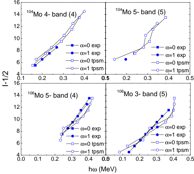
FIG. 15. Plots of I - 0.5 vs rotational frequency \hbar\omega = (E(I) - E(I - 2))/2 for ^{104,106}\text{Mo} from the experiment and TPMSM calculations.
