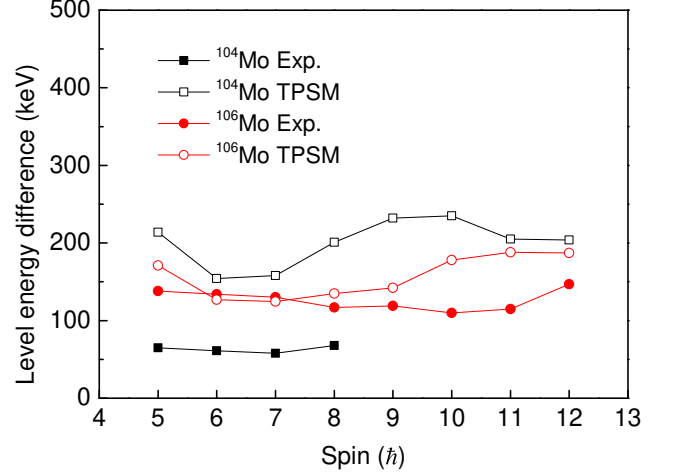
FIG. 16. Level energy differences E_5(I) - E_4(I) between chiral doublet bands in ^{104,106}\text{Mo} from the experiment and TPMSM calculations.
